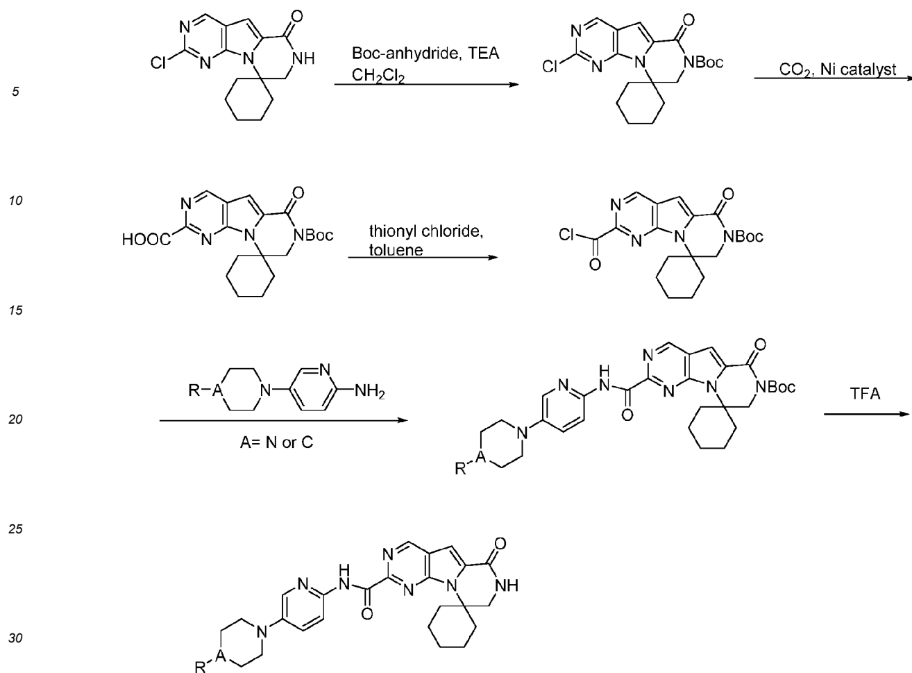
Scheme 10
