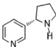
(S)-nornicotine
