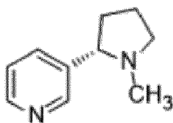
(S)-nicotine
