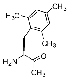
2,4,6-trimethyl-L-phenylalanine (Tmp)
