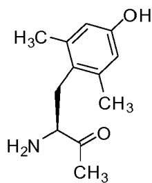
2,6-dimethyl-L-tyrosine (Dmt)
