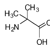
alpha-amino isobutyric acid (Aib)
