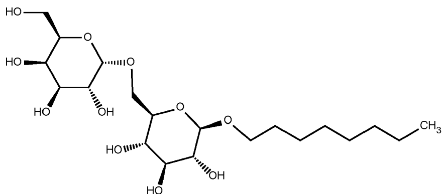
1-Octyl beta-D-melibioside
