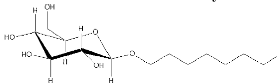
Octylglucoside
