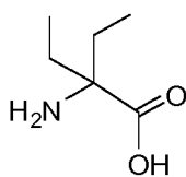
2,2-diethylglycine (Deg)
