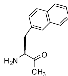
2-(2-naphthyl-L-alanine (Nal(2))
