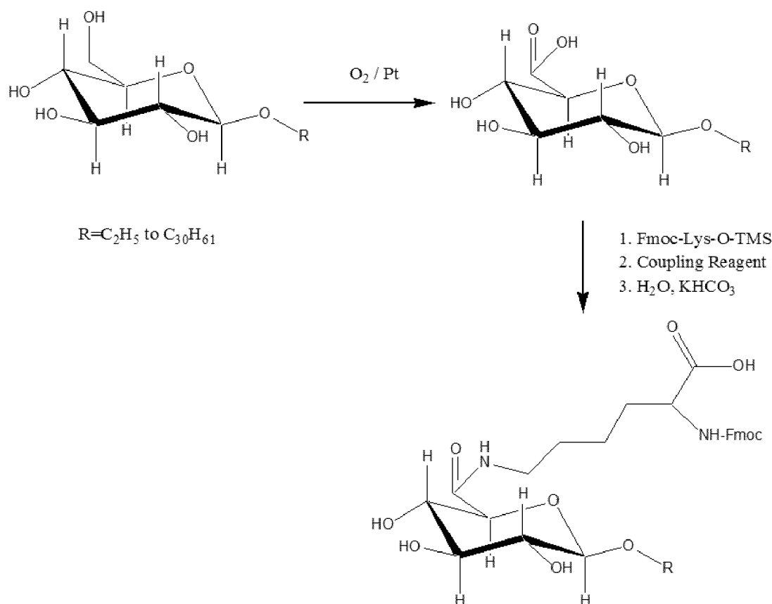
Scheme 4. Example of a preparation of a reagent.
