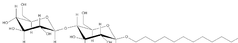
Dodecylmaltoside
