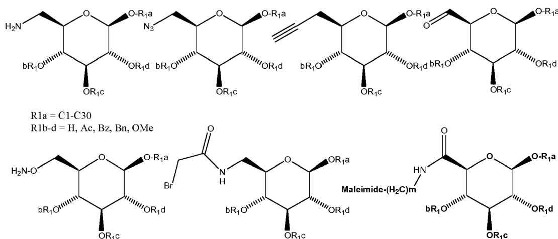
Scheme 6. Additional reagent examples.
