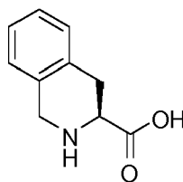
1,2,3,4-tetrahydroisoquinoline- 3-carboxylic acid (Tic)
