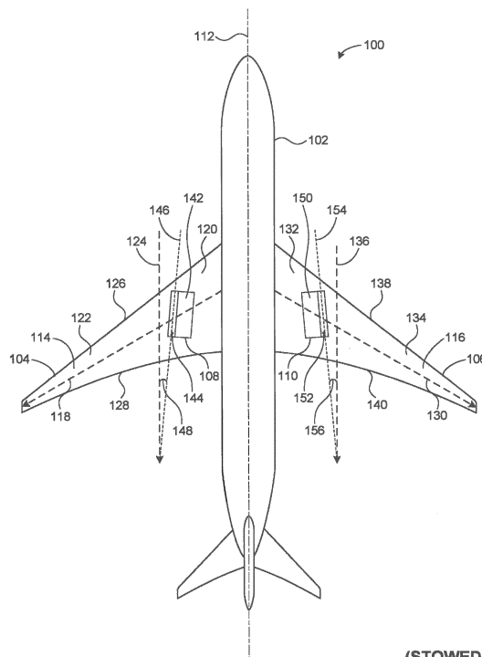
(STOWED) FIG. 1
