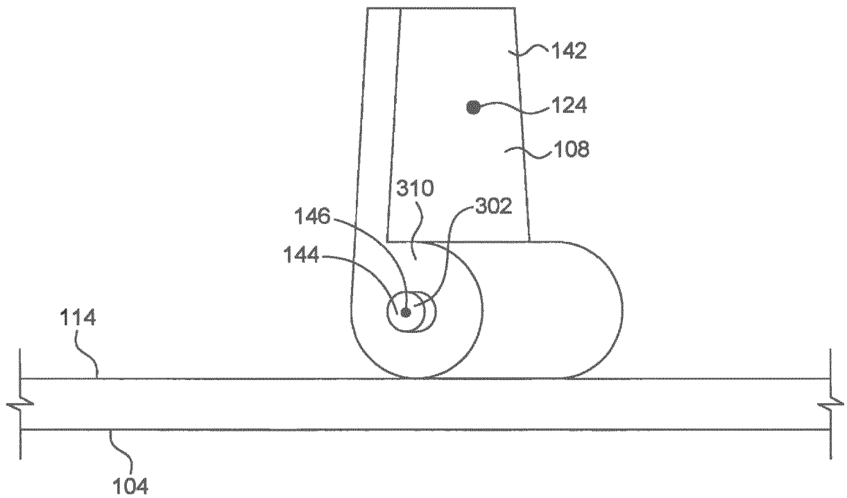
(DEPLOYED) FIG. 9
