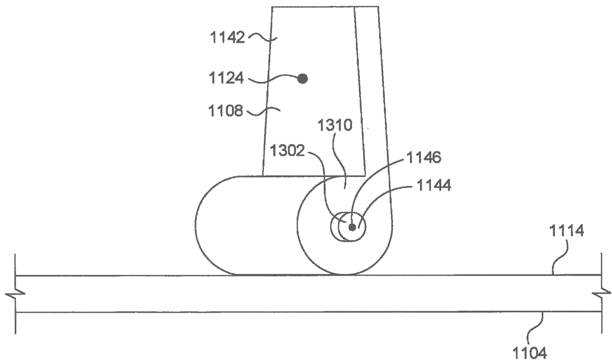
(DEPLOYED) FIG. 19
