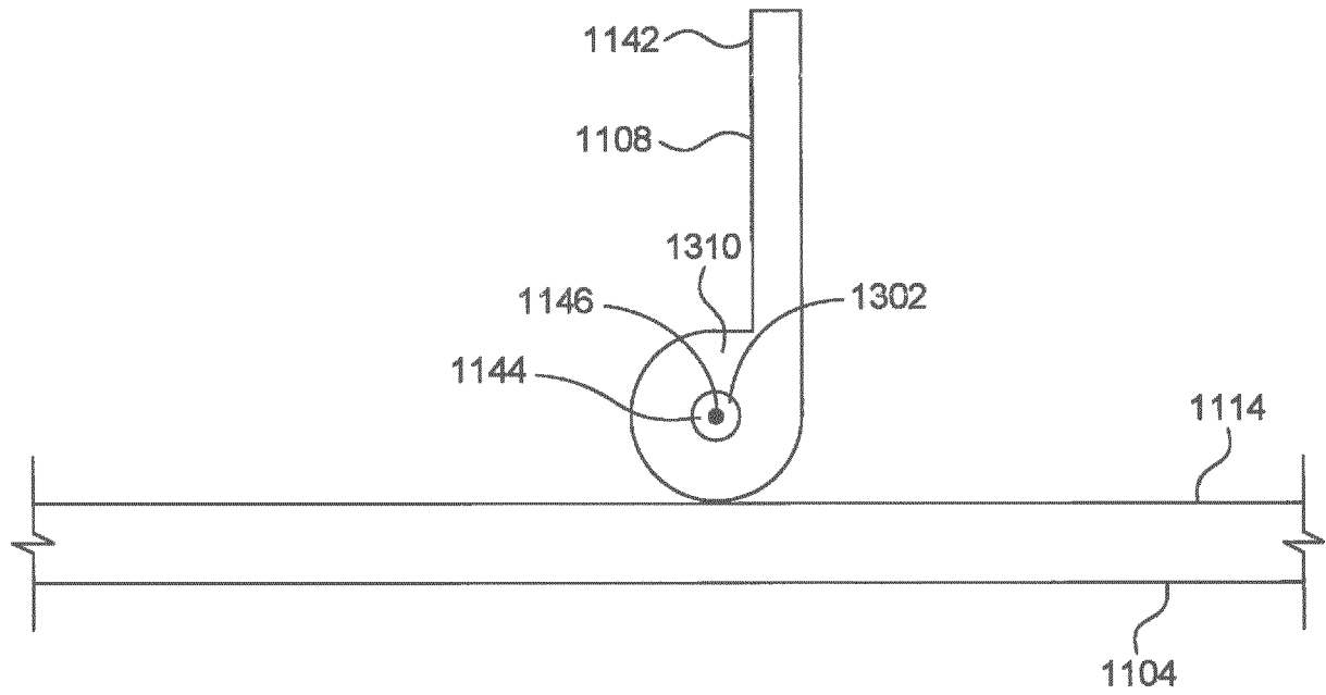
(DEPLOYED) FIG. 18
