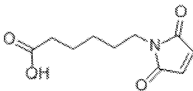
Compound I
