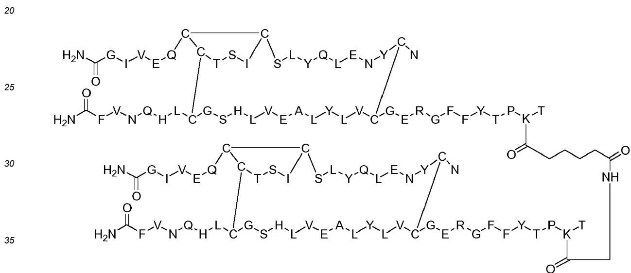
Dimer 60;
