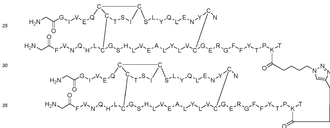
Dimer 49;
