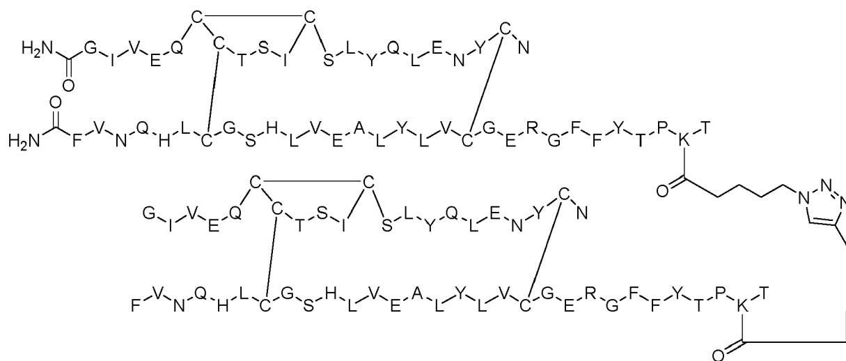
Dimer 45;
