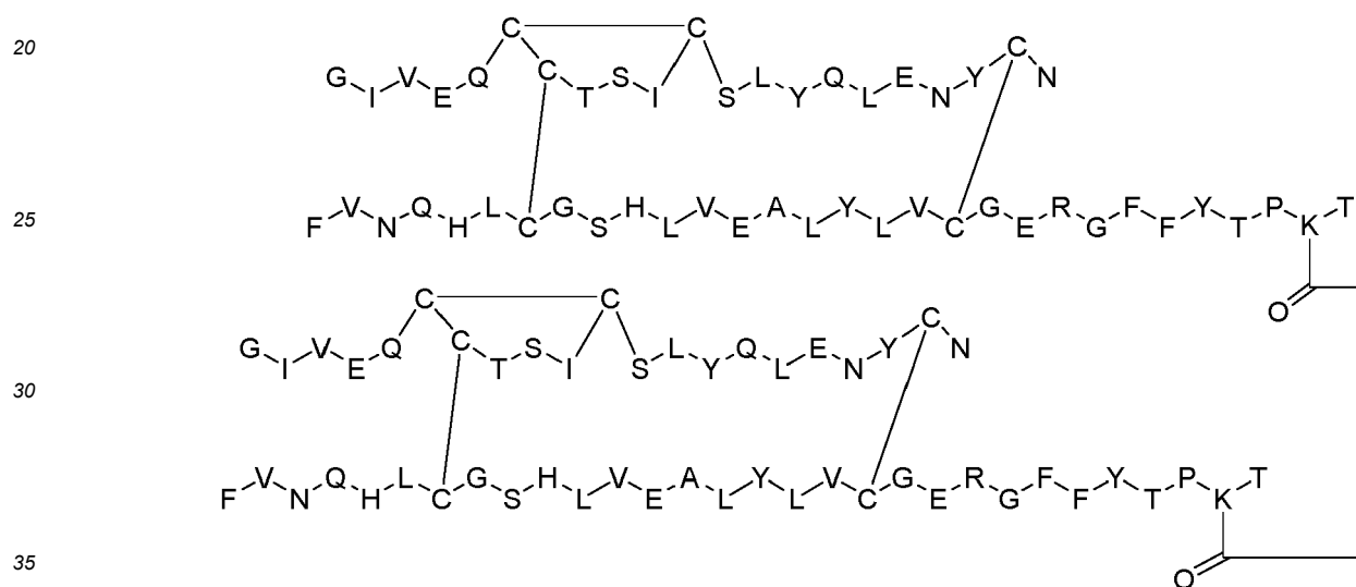
Dimer 7;
