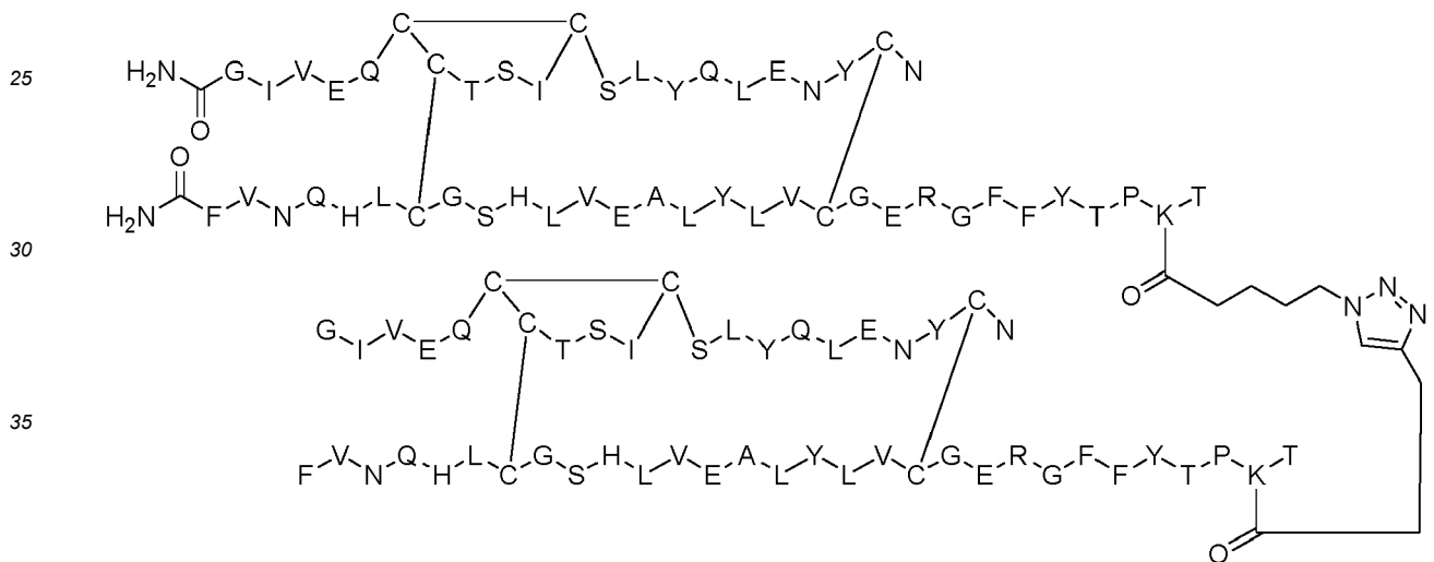
Dimer 45;
