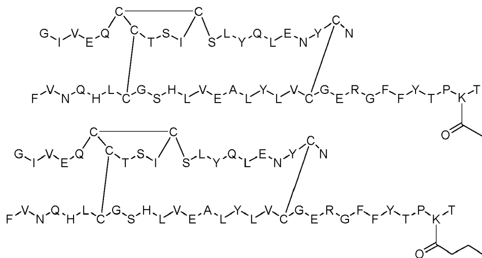
Dimer 9;
