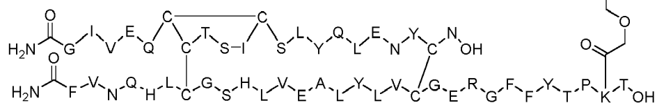
Dimer 3;
