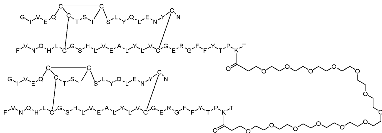
Dimer 6;
