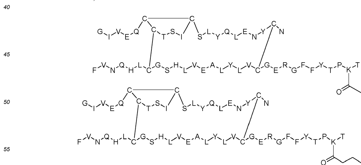
Dimer 9;
