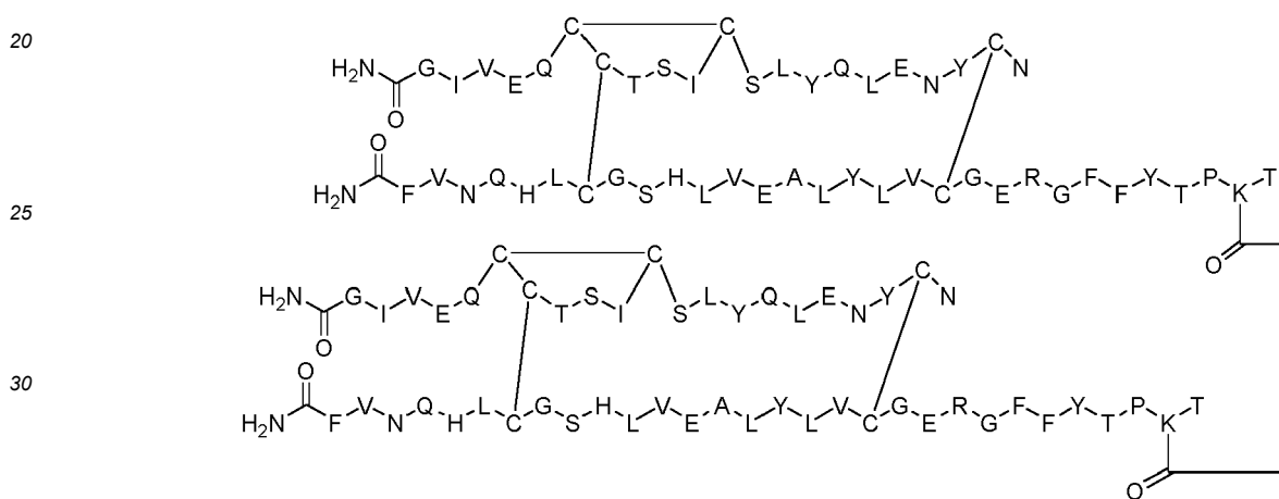
Dimer 12;
