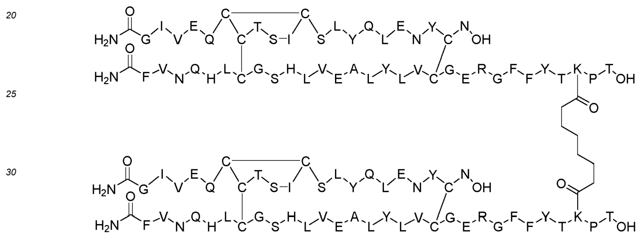
Dimer 32;
