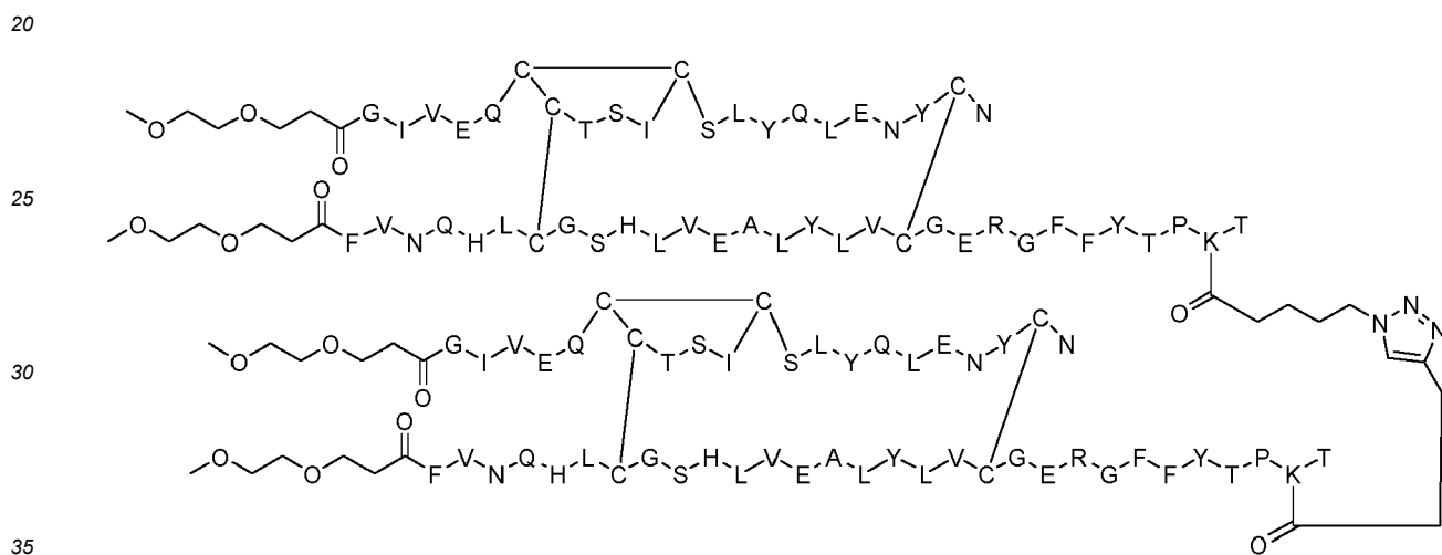
Dimer 50;
