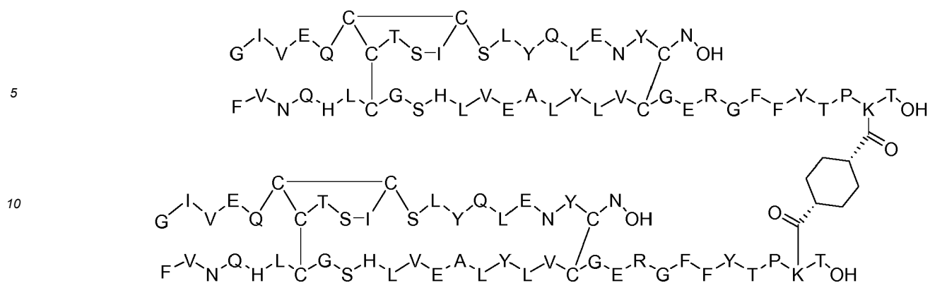
Dimer 72;
