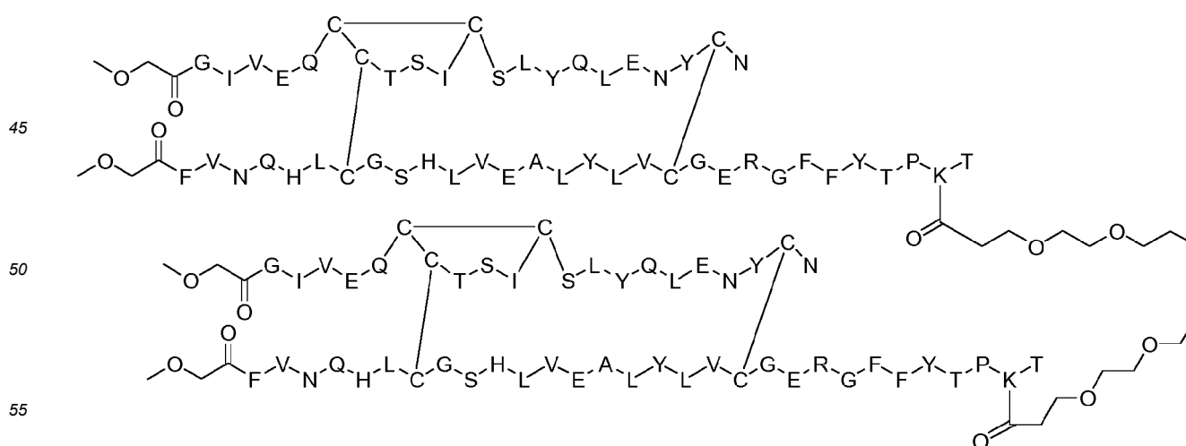
Dimer 70;
