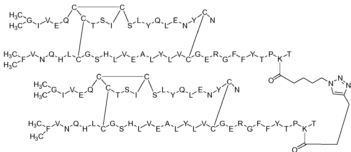
Dimer 60;
