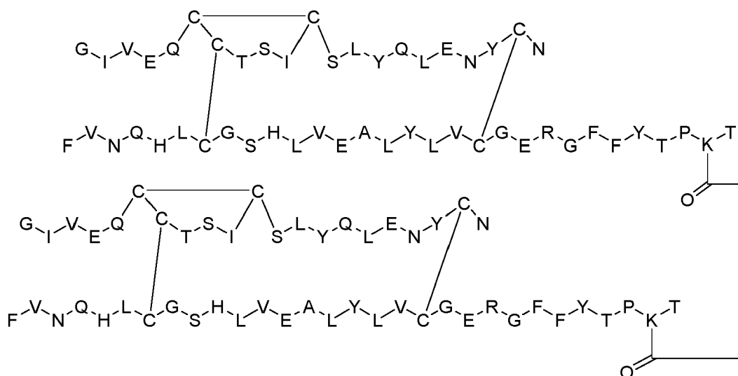
Dimer 8;
