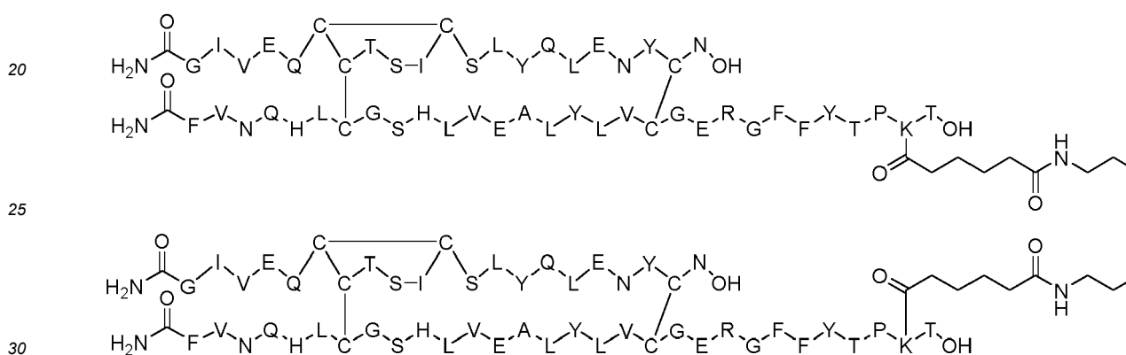
Dimer 27;
