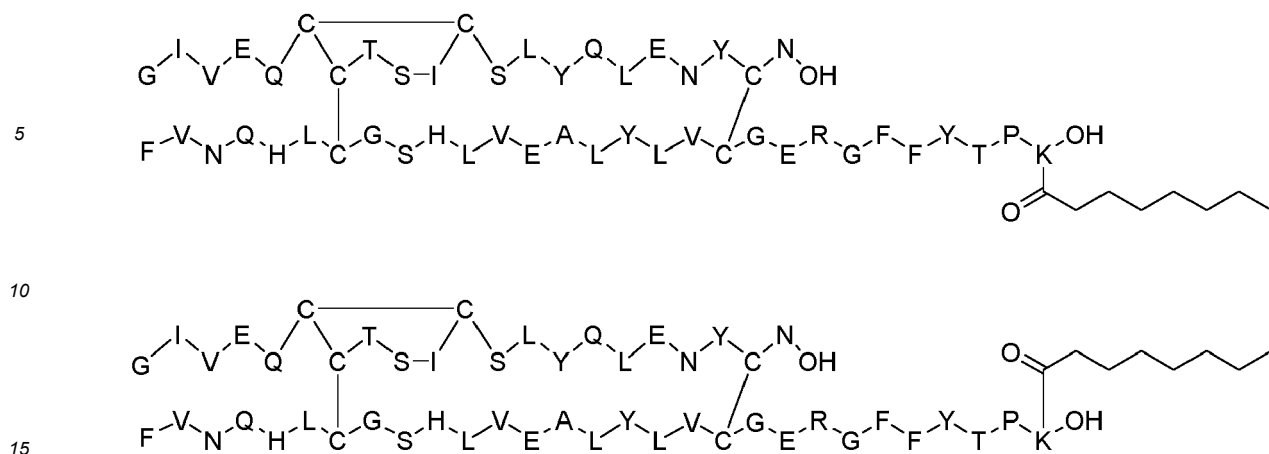
Dimer 38;
