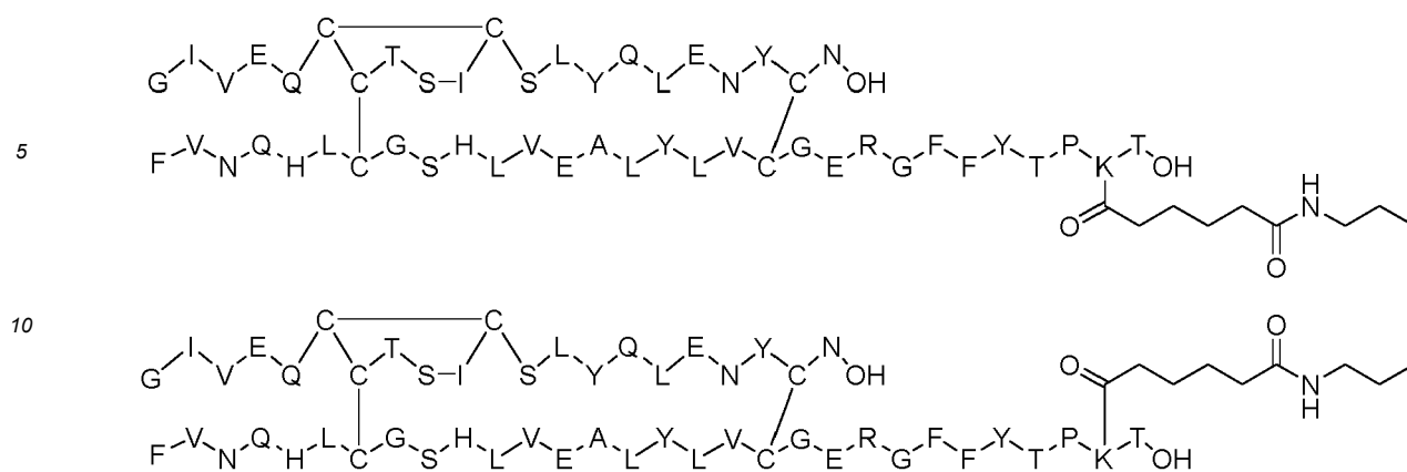
Dimer 26;
