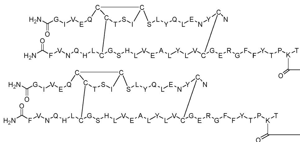
Dimer 12;
