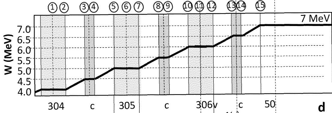
FIG.3(b1) 7 MeV
