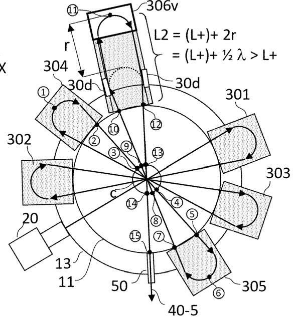
FIG.3(c2) 5 MeV
