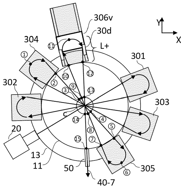
FIG.3(b2) 7 MeV
