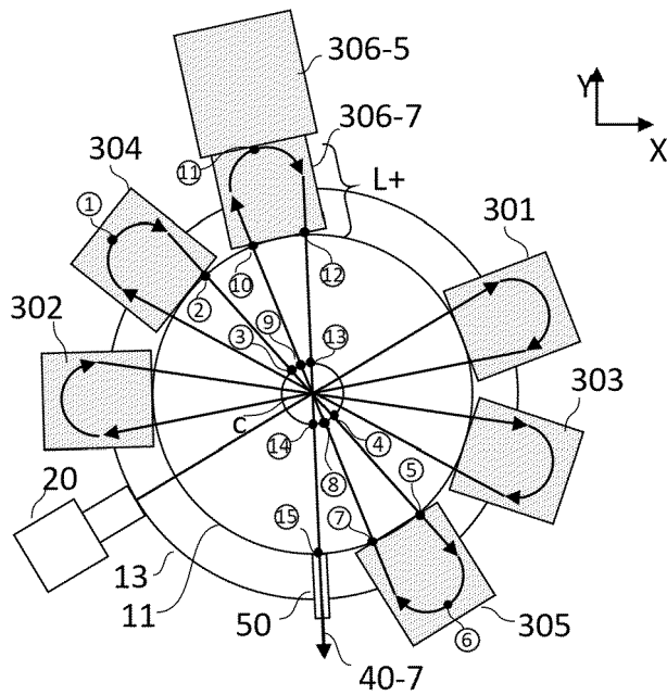
FIG.3(b2) 7 MeV
