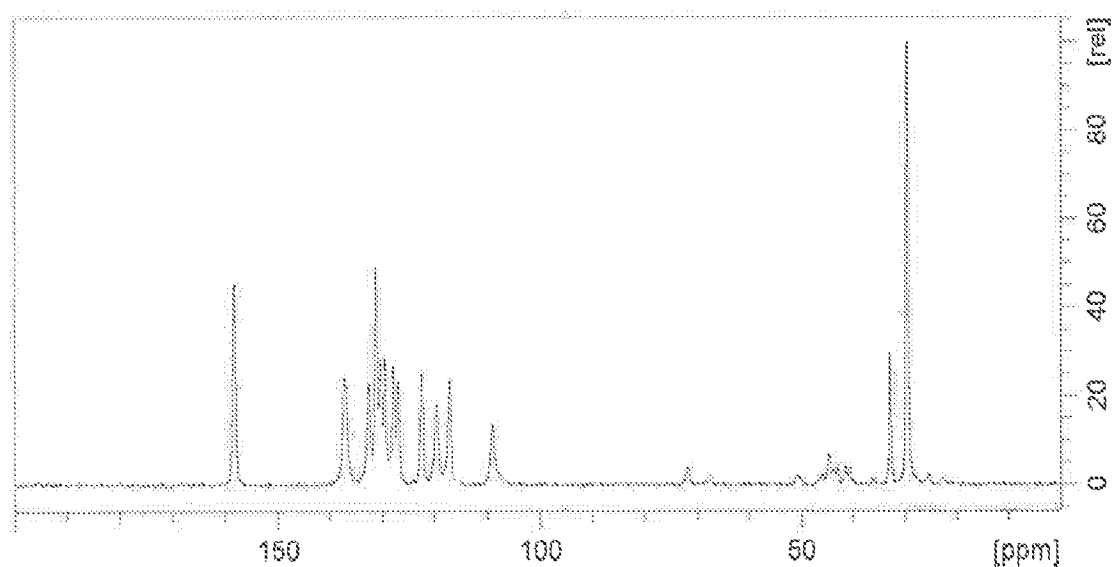
Figure 24: Solid state ^{13}\text{C} NMR spectrum of Plinabulin hydrochloride Form Alpha at the range of 200-0 ppm.
