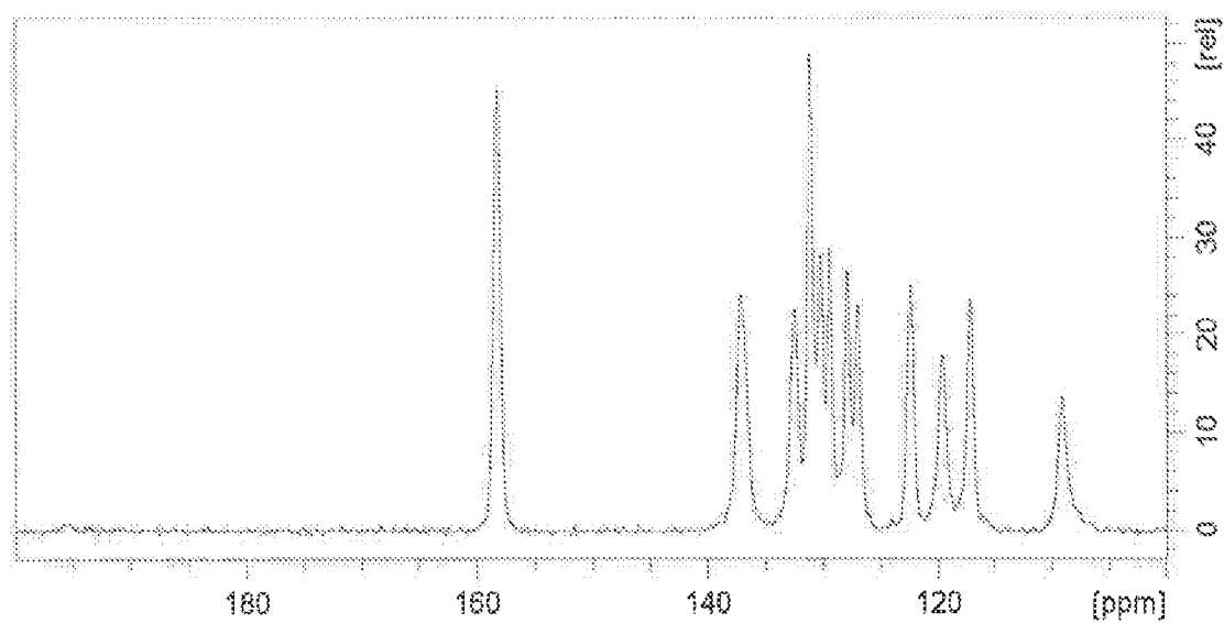
Figure 25: Solid state ^{13}\text{C} NMR spectrum of Plinabulin hydrochloride Form Alpha at the range of 200-100 ppm.
