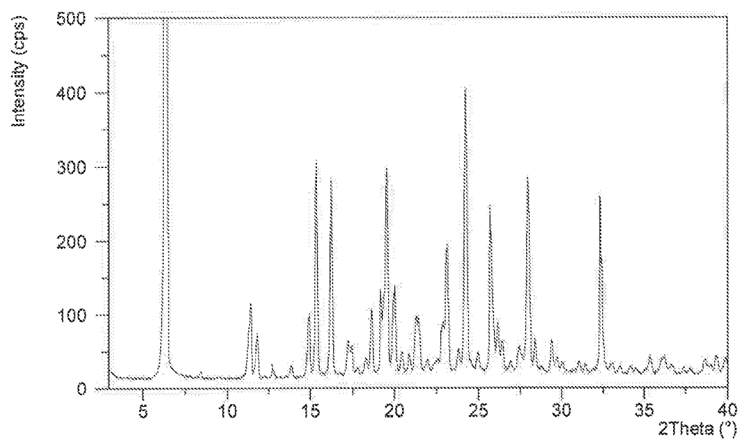
Figure 6: XRPD pattern of Plinabulin Form F obtained in Example 6
