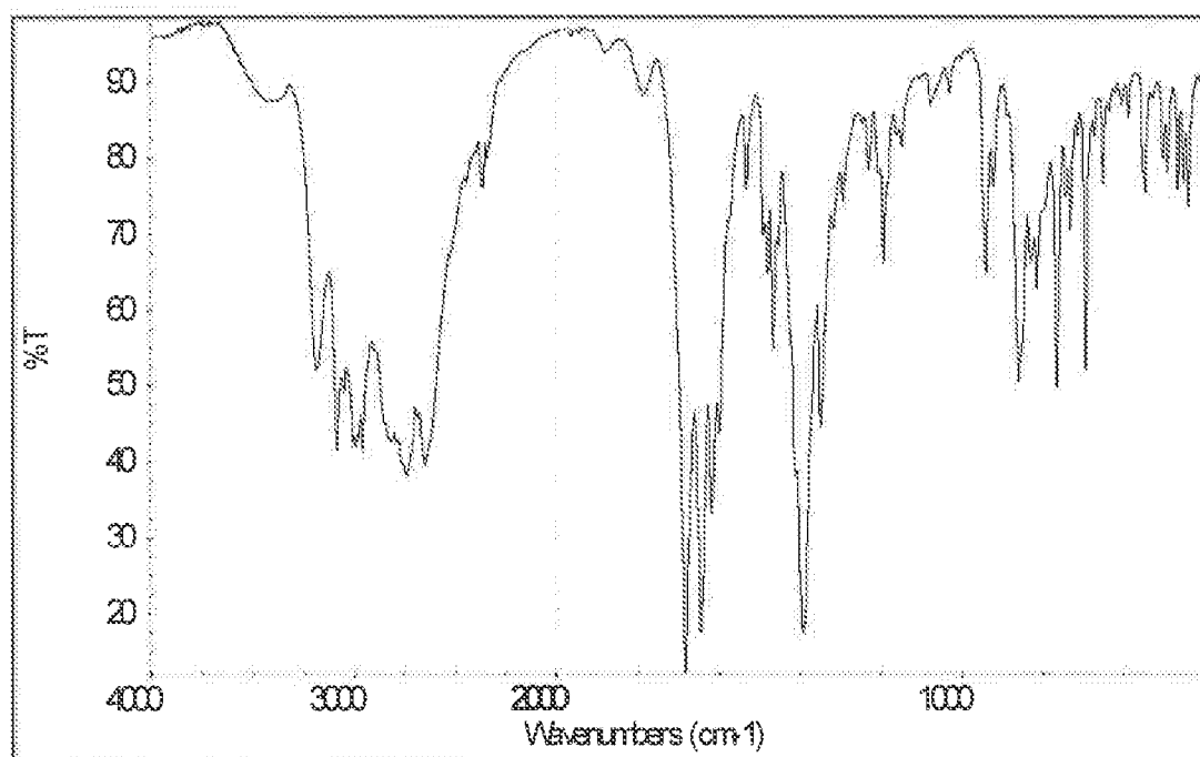
Figure 27: Fourier-transform infrared (FTIR) spectrum of Plinabulin hydrochloride Form Alpha at the range of 400-4000 \text{cm}^{-1} .
