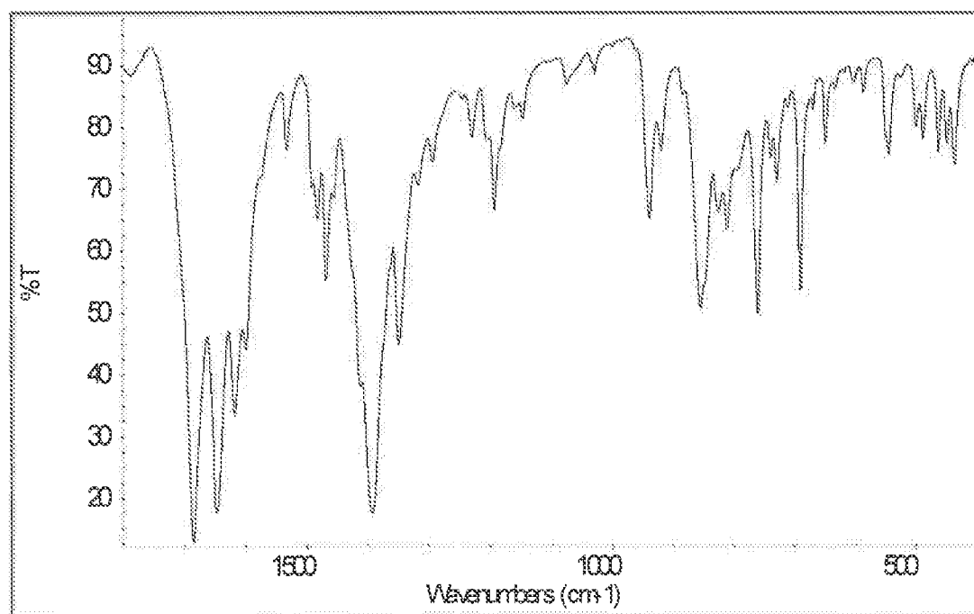
Figure 28: Fourier-transform infrared (FTIR) spectrum of Plinabulin hydrochloride Form Alpha at the range of 400-1800 \text{cm}^{-1} .
