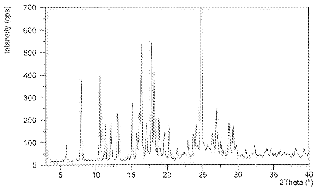
Figure 7: XRPD pattern of Plinabulin Form G obtained in Example 7
