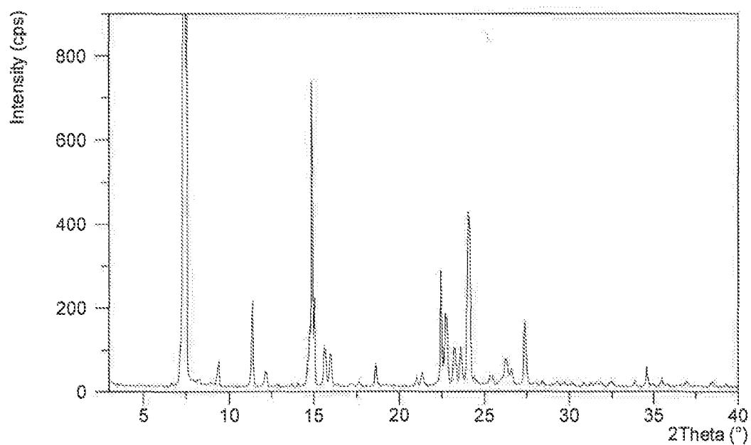
Figure 1: XRPD pattern of Plinabulin Form A obtained in Example 1
