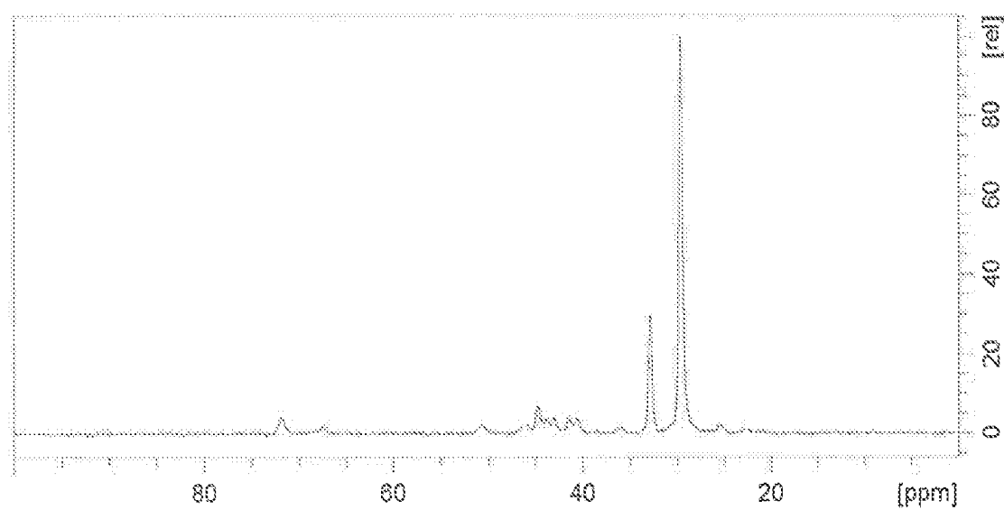
Figure 26: Solid state ^{13}\text{C} NMR spectrum of Plinabulin hydrochloride Form Alpha at the range of 100-0 ppm.
