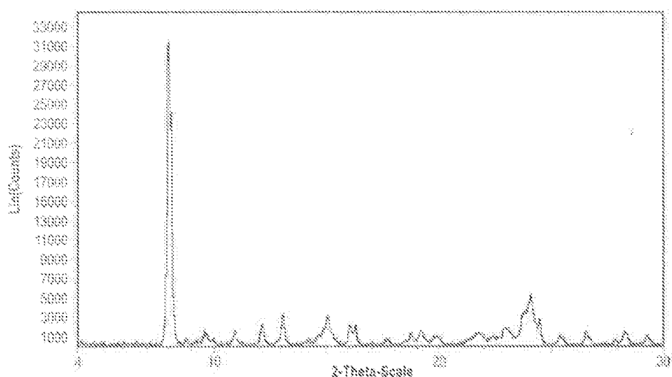
Figure 10: XRPD pattern of form 5 which is described in PCT application WO2017011399.
