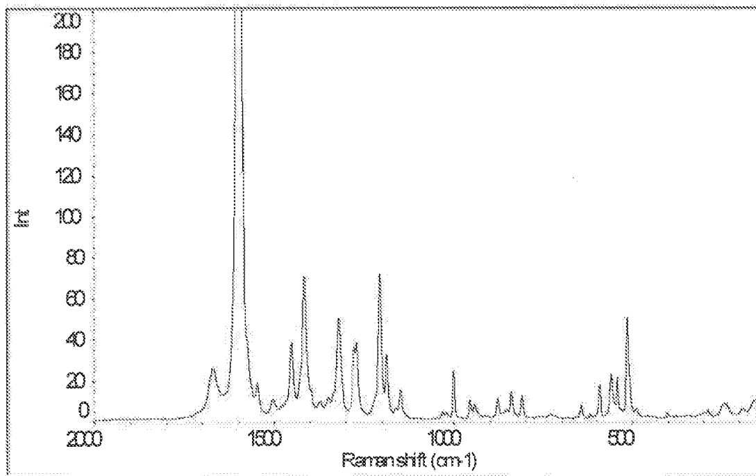
Figure 23: FT-Raman spectrum of Plinabulin Form G at the range of 400-2000 \text{cm}^{-1} .
