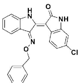
[Chemical formula 4]
