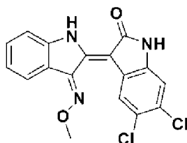
[Chemical formula 3]
