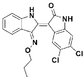
[Chemical formula 4]
