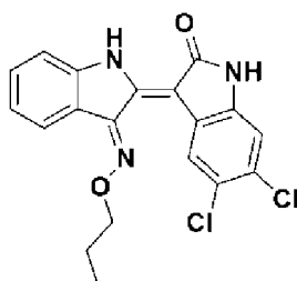
[Chemical formula 3]
