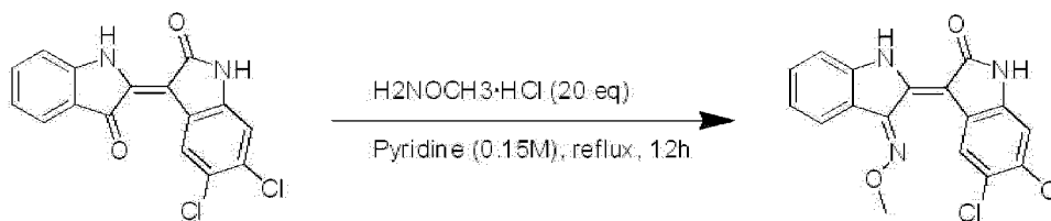
5,6-dichloro-[2,3'-biindolinylidene]-2,3-dione
