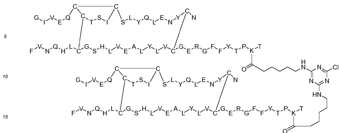
Dimer 68;
