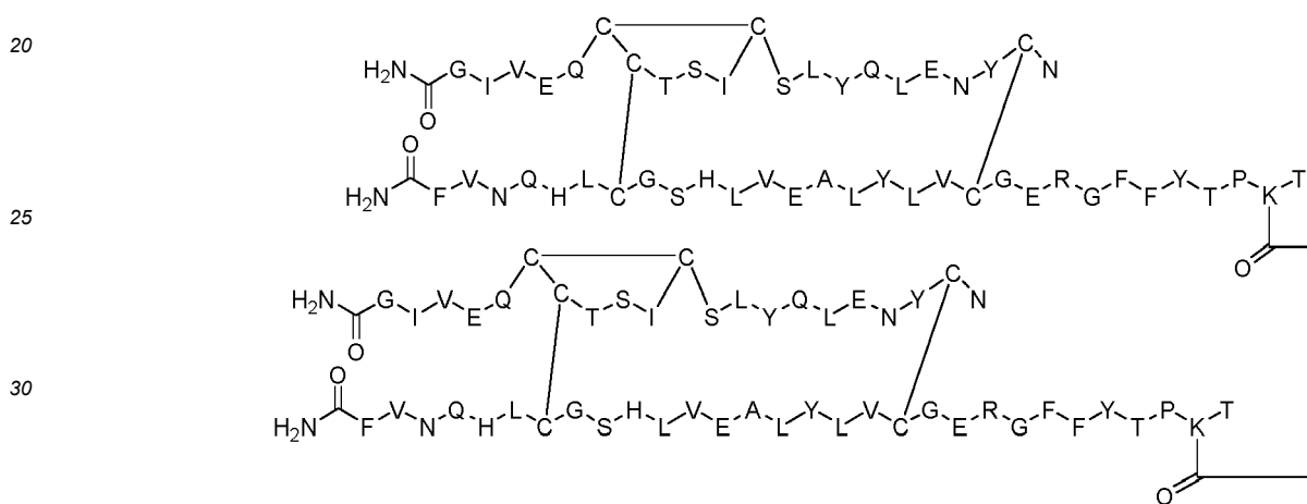
Dimer 12;
