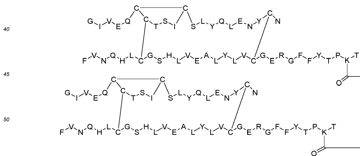
Dimer 8;
