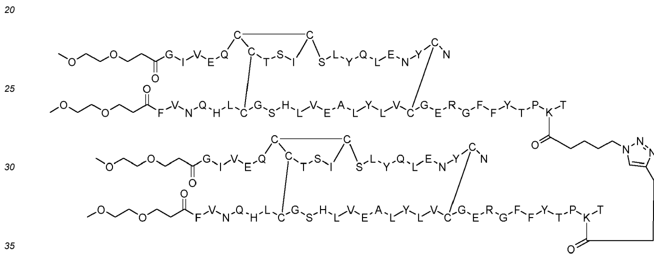
Dimer 50;
