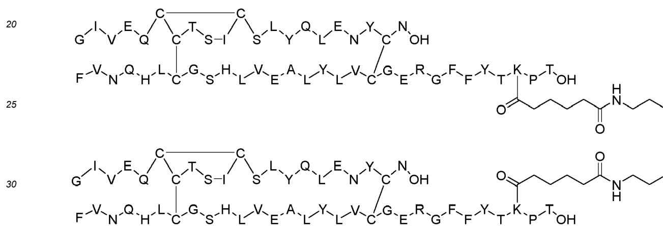
Dimer 34;
