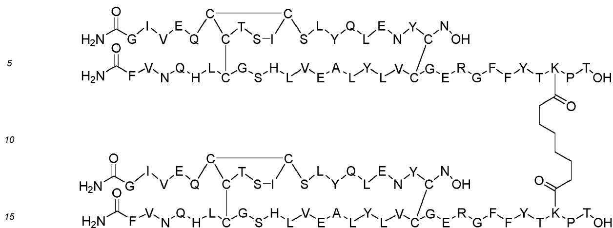
Dimer 32;
