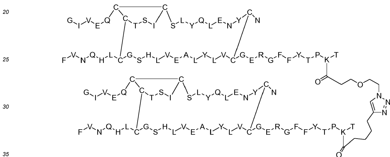
Dimer 82;
