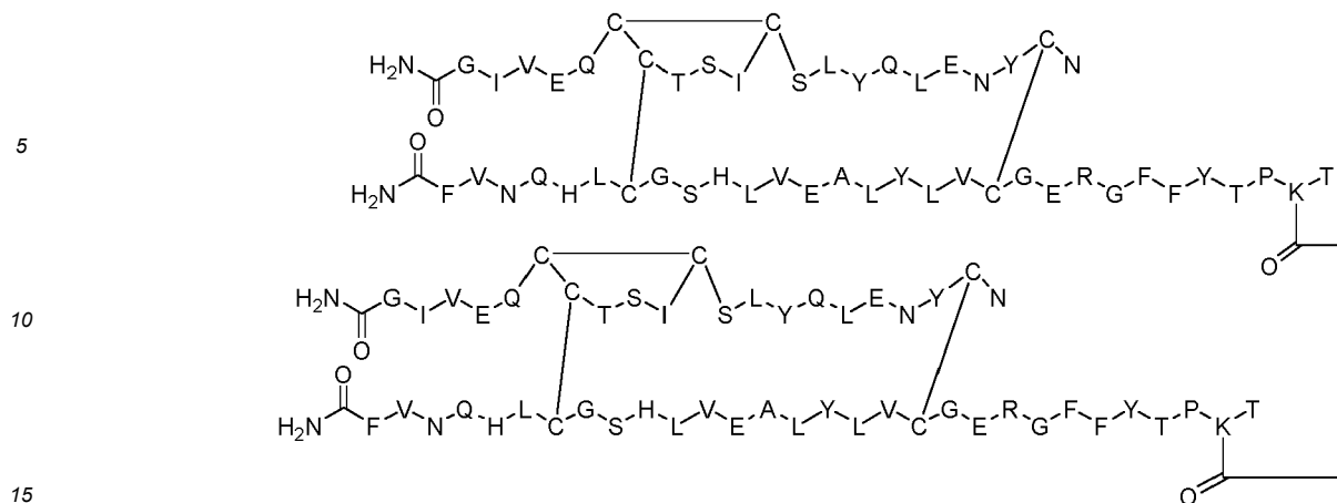
Dimer 12;
