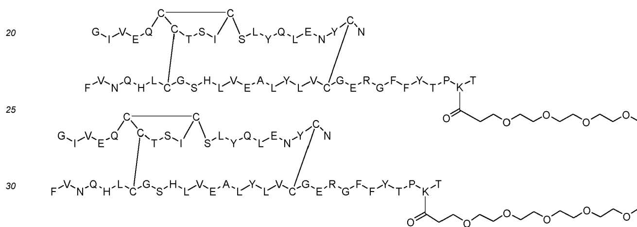
Dimer 7;
