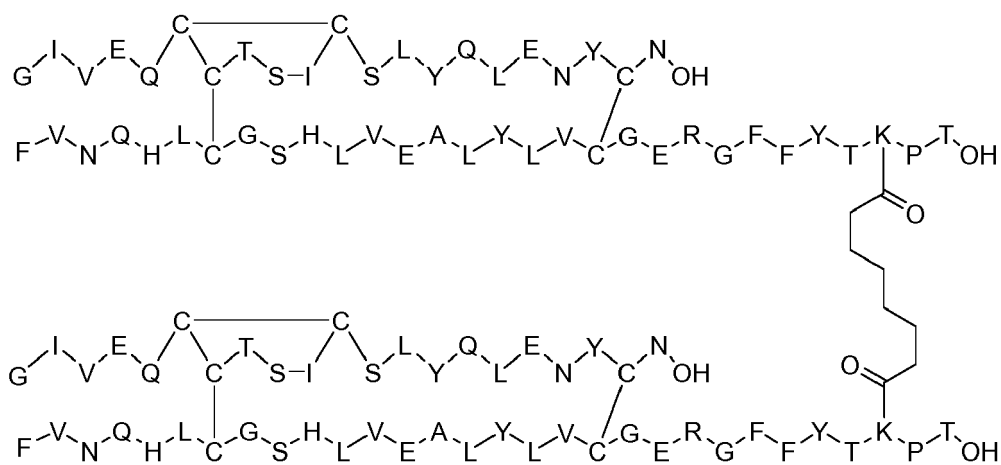
Dimer 18;
