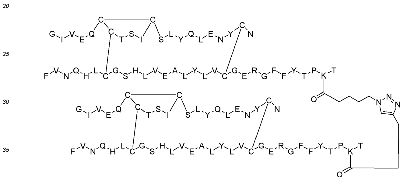
Dimer 40;
