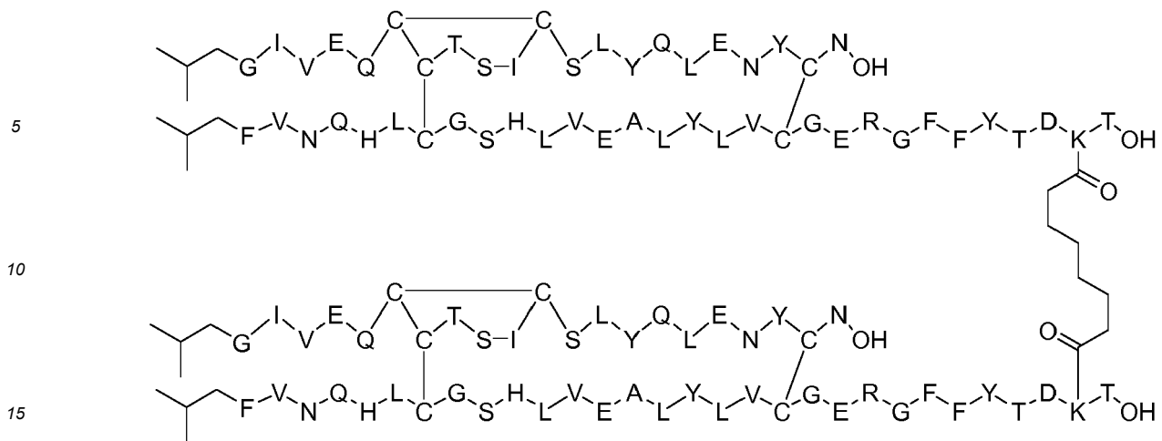
Dimer 65;
