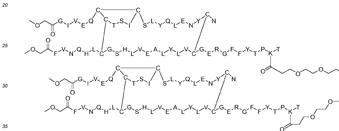
Dimer 70;
