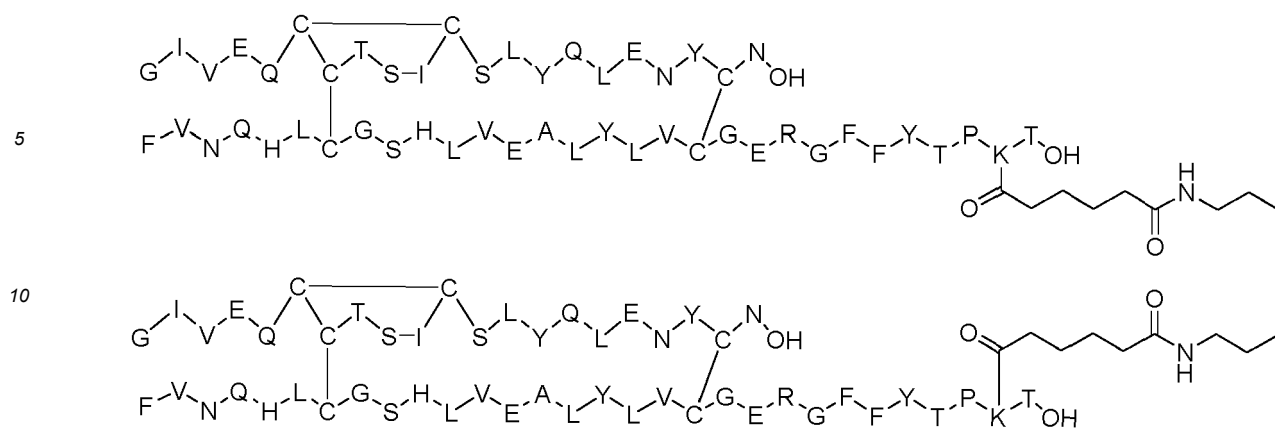
Dimer 26;
