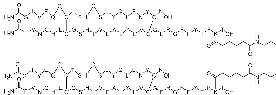
Dimer 27;
