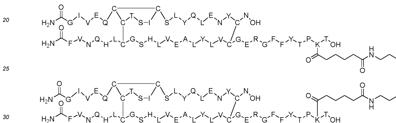
Dimer 27;
