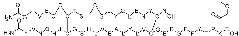
Dimer 3;
