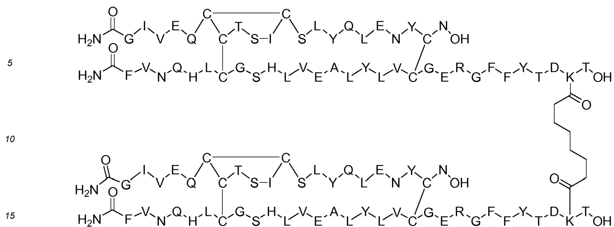
Dimer 83;
