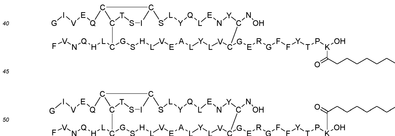
Dimer 38;
