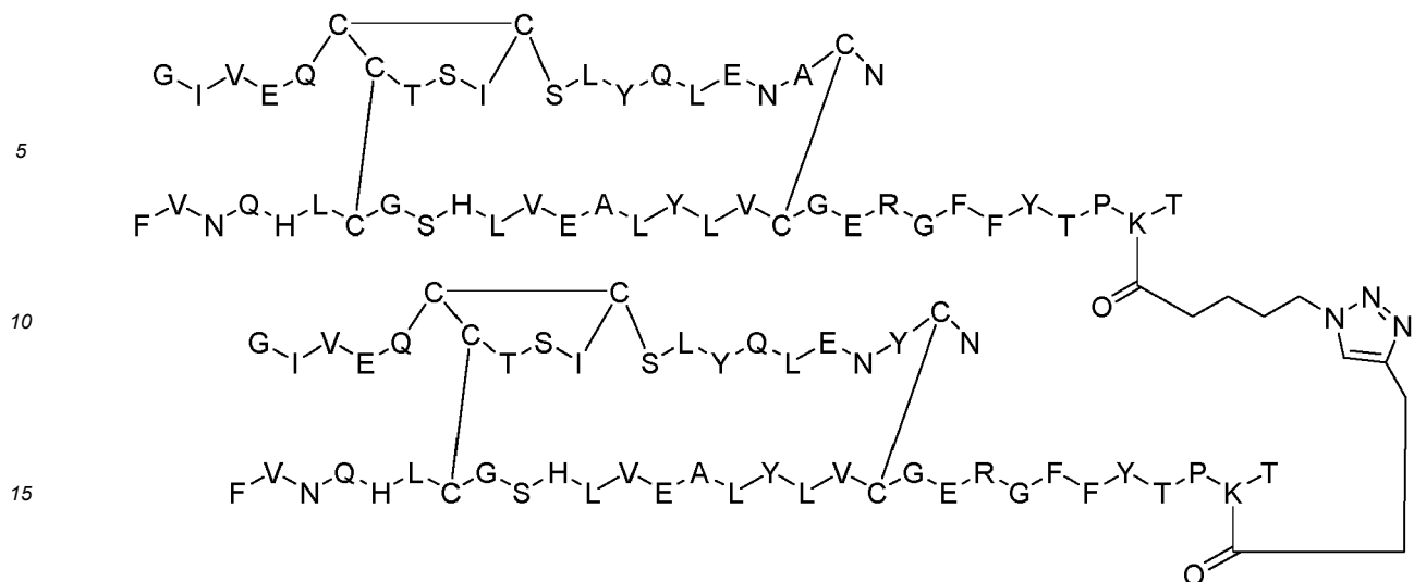
Dimer 41;
