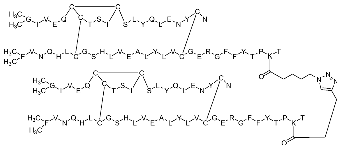
Dimer 60;
