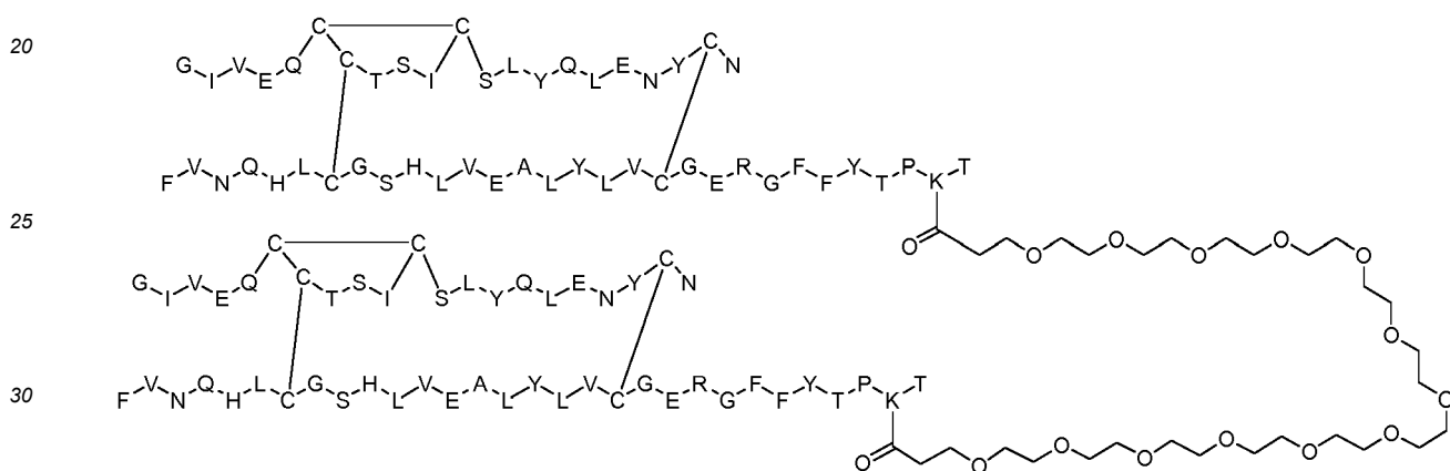
Dimer 6;
