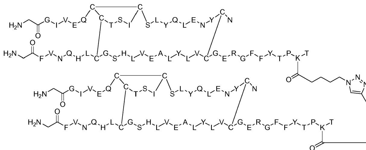
Dimer 49;
