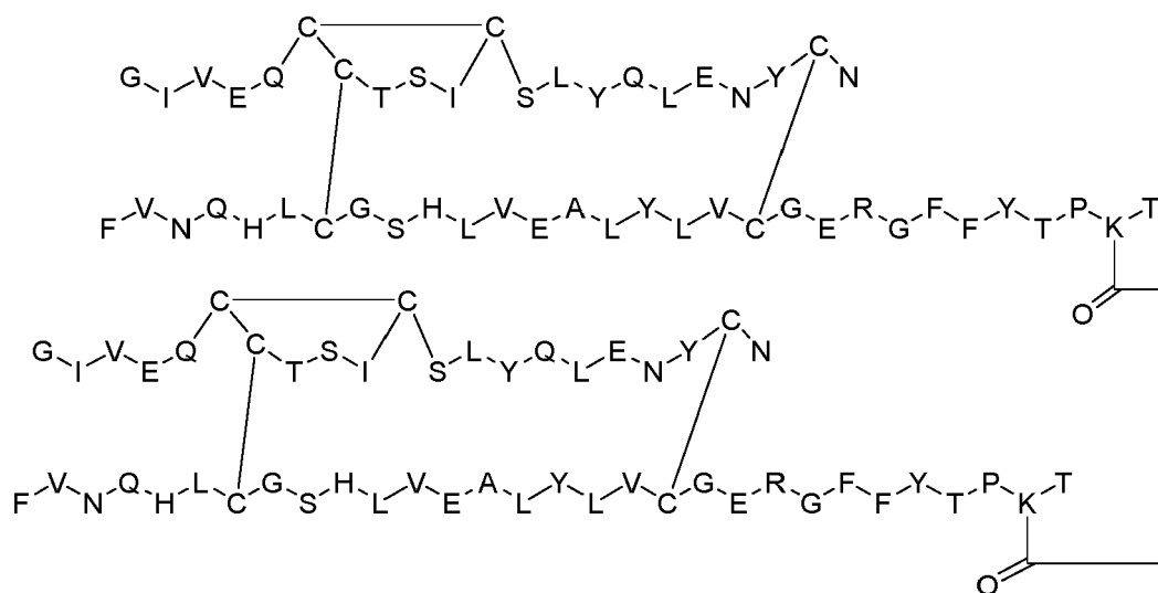
Dimer 8;
