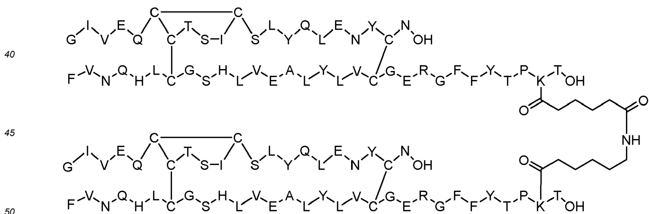
Dimer 22;
