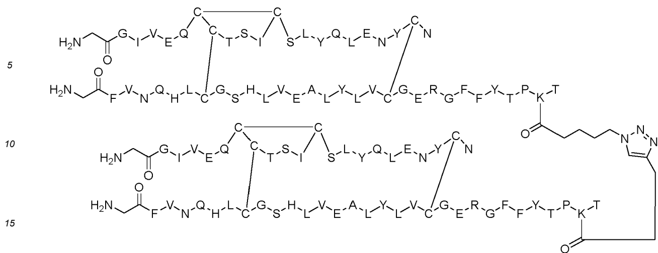
Dimer 49;
