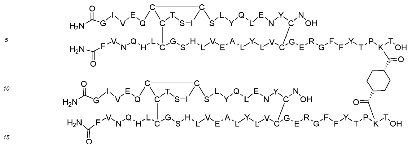
Dimer78;
