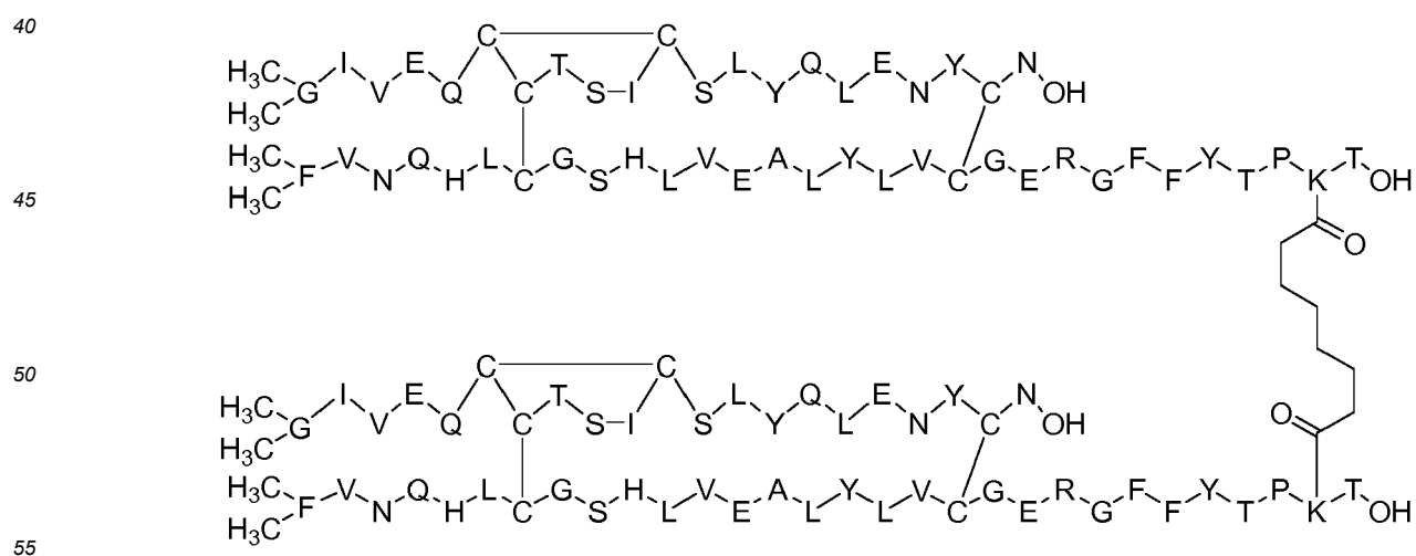
Dimer 58;
