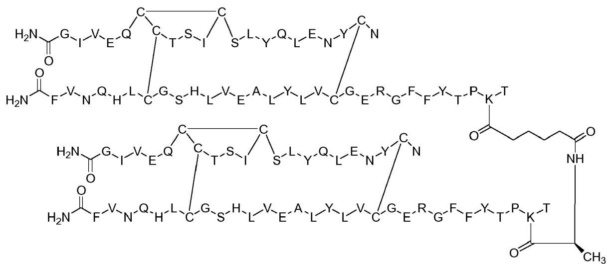
Dimer 62;
