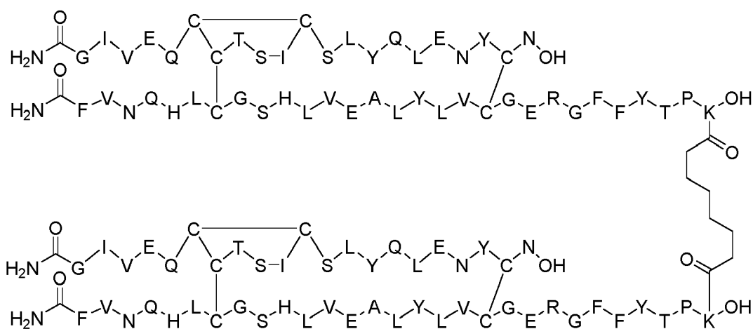
Dimer 28;
