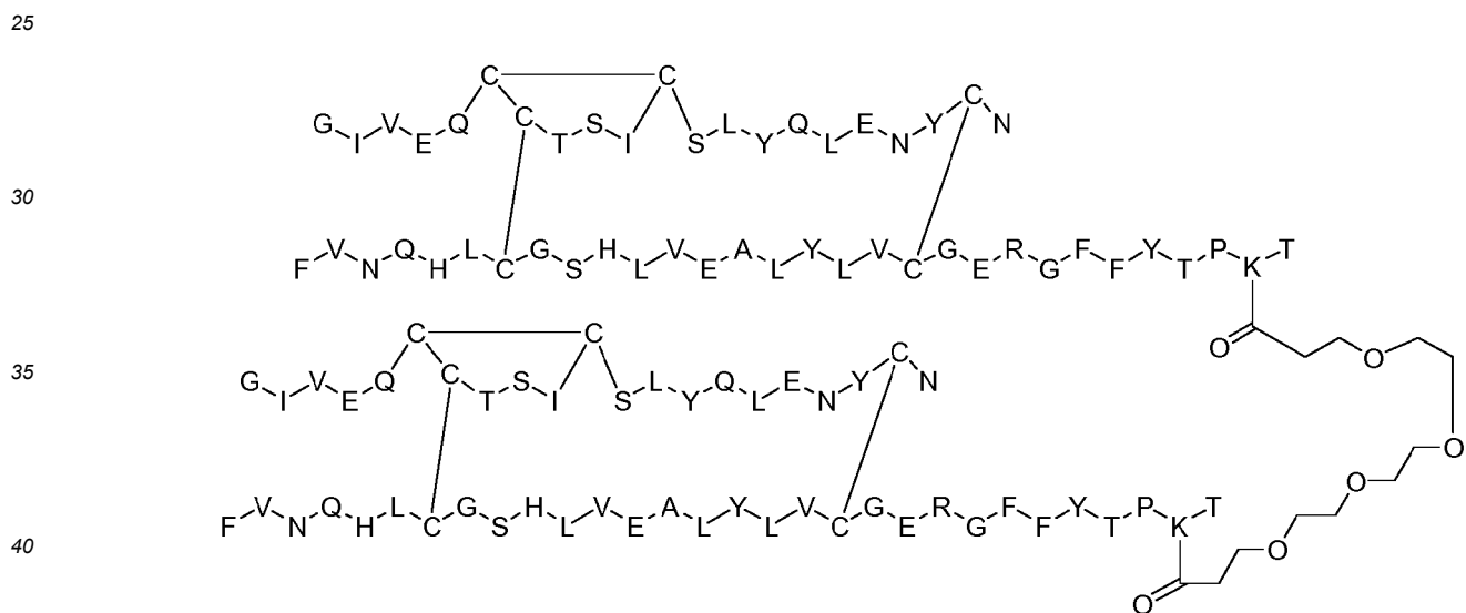
Dimer 88;
