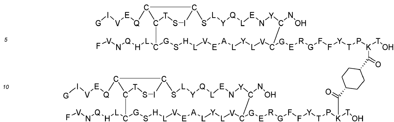
Dimer 72;
