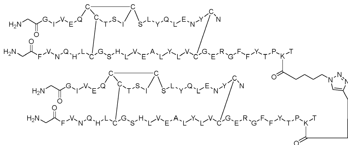
Dimer 49;
