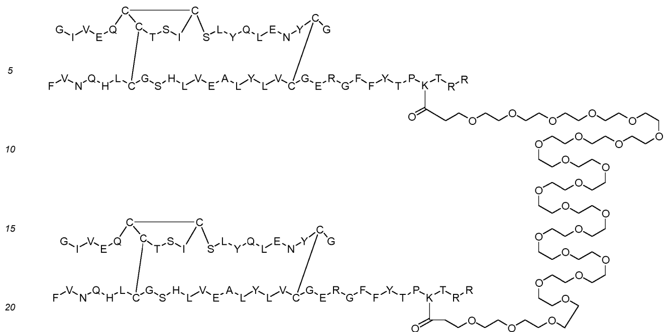
Dimer 87;
