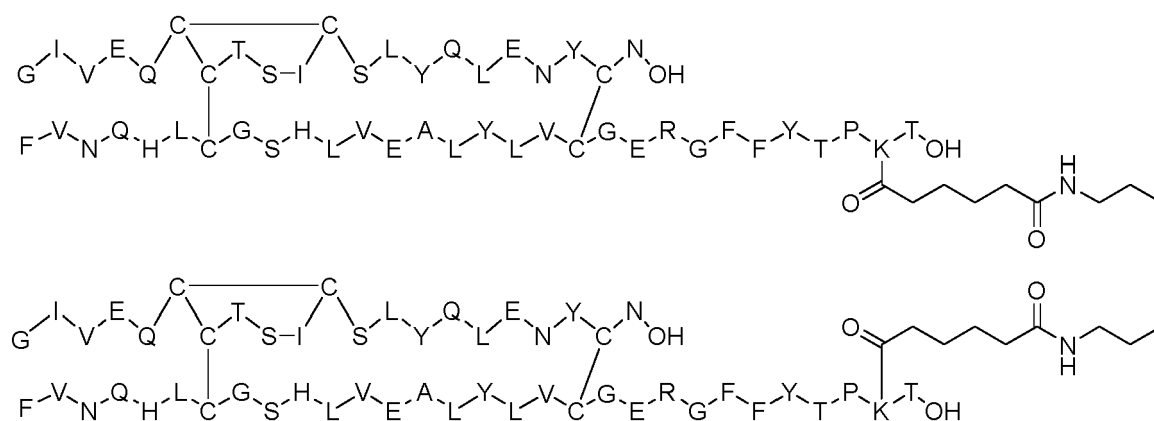
Dimer 26;
