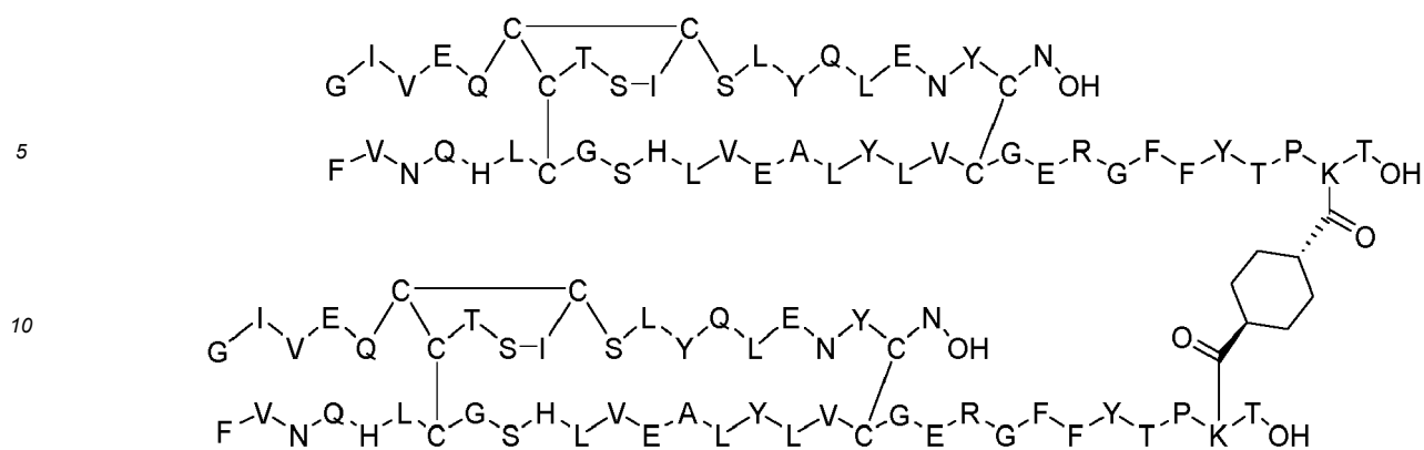
Dimer 71;
