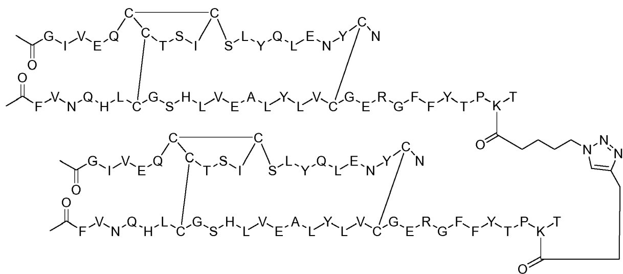
Dimer 48;
