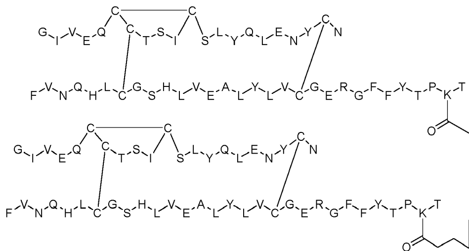
Dimer 9;
