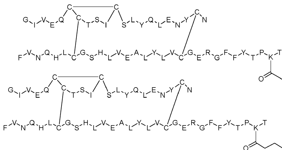
Dimer 9;
