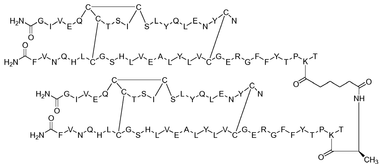
Dimer 62;
