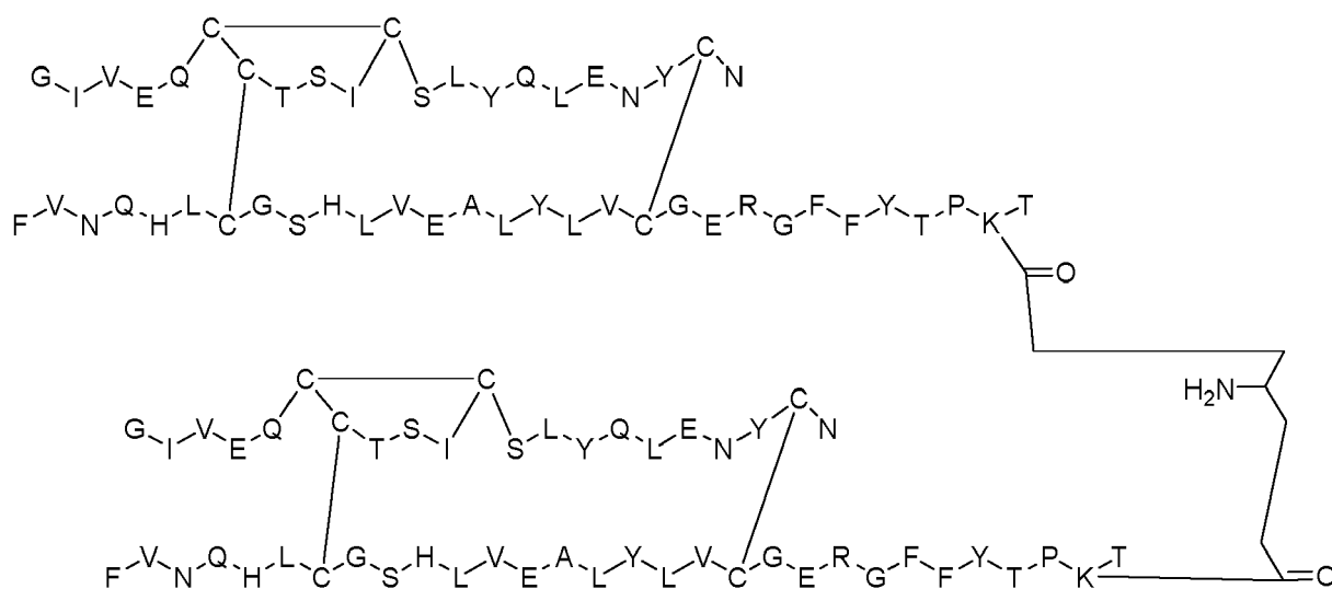
Dimer 94
