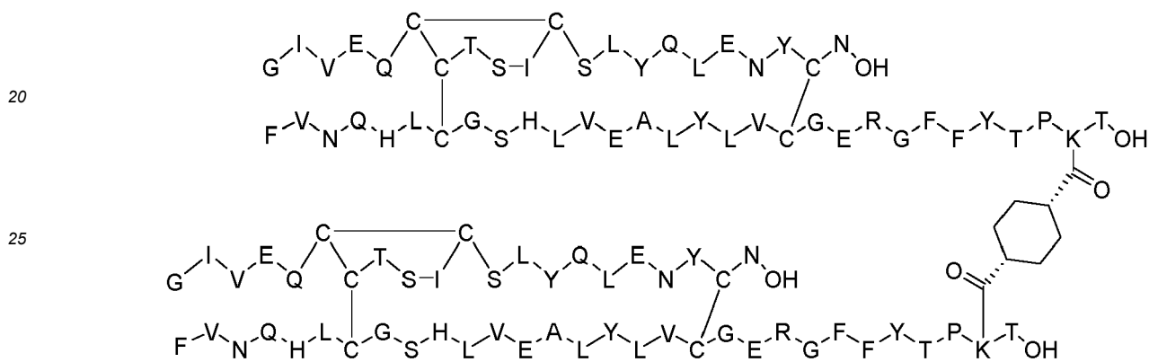
Dimer 72;
