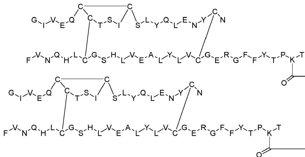
Dimer 8;
