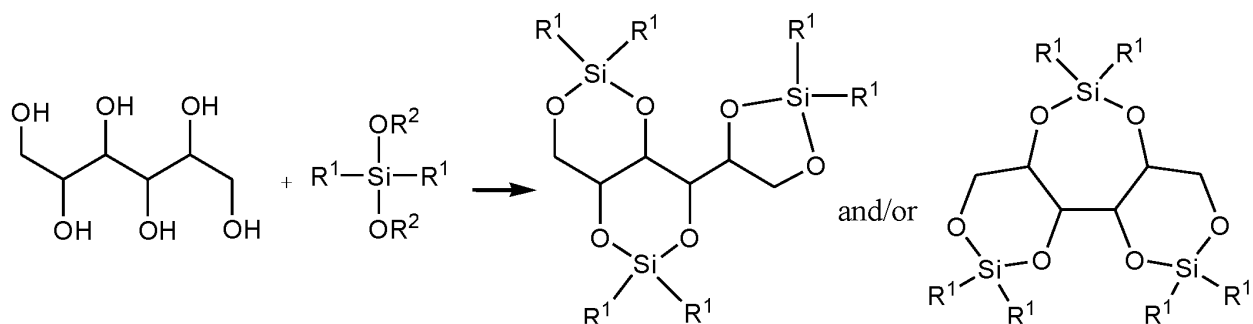
Scheme 3
