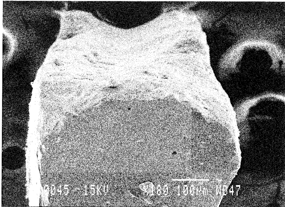
Fig. 10 PRIOR ART
