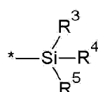
[Chemical Formula 3]
