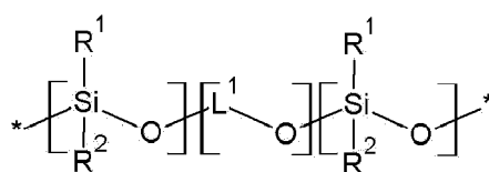
[Chemical Formula 1]
