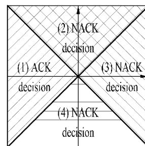
(b) Proposed 1-bit ACK/NACK decision region
