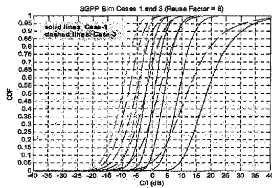
Figure 3: C/I distributions of 6 best sites detected by a uniformly-dropped UE (Reuse Factor = 6).
