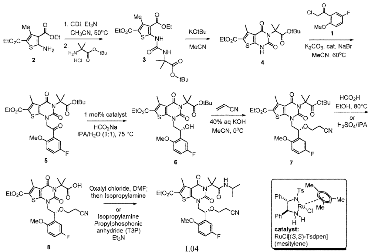
Scheme 1: Synthetic route to I.04
