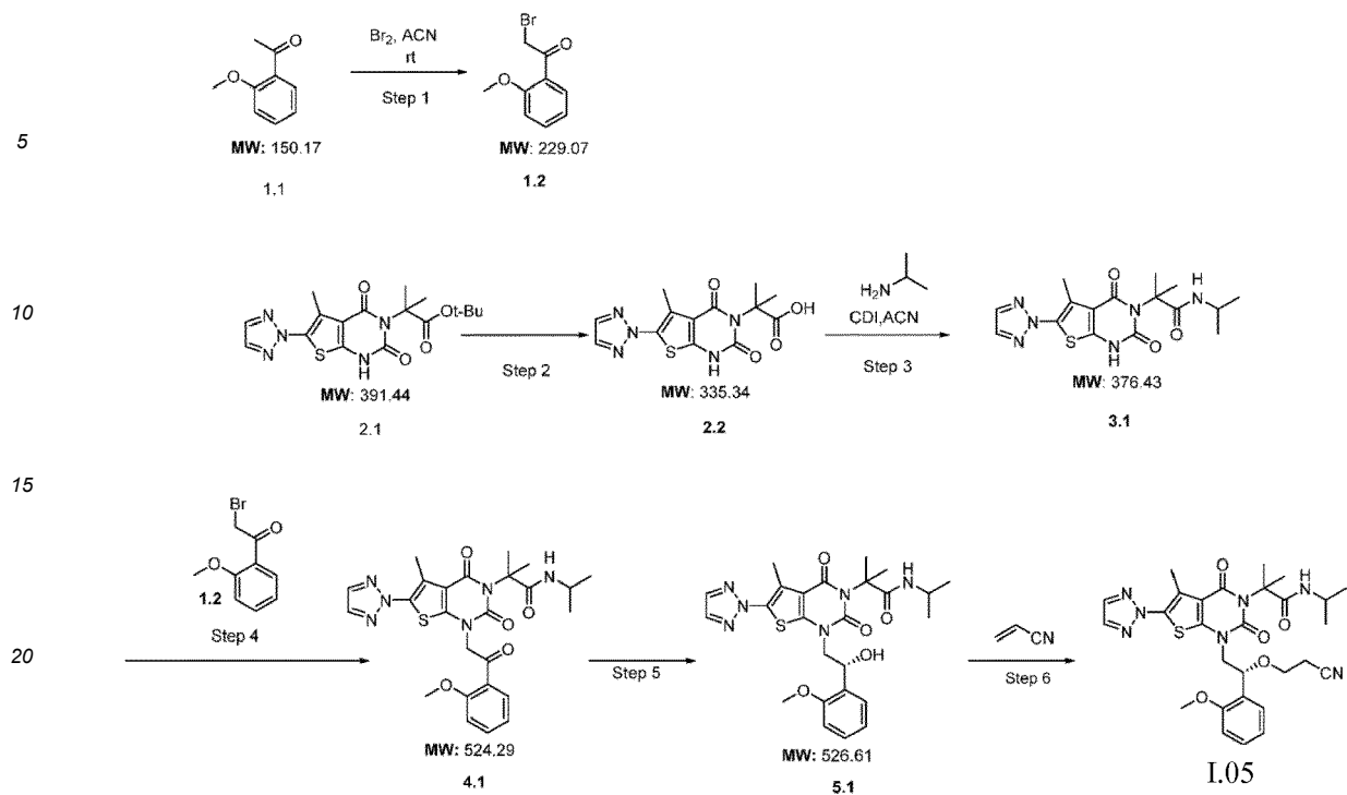
Scheme 2: Synthetic route to I.05
