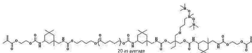
Silicone-pendant type urethane (meth)acrylate 2-8
