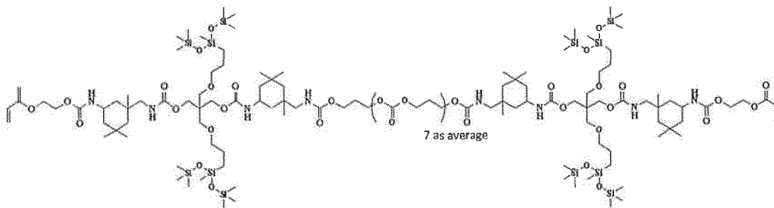
Silicone-pendant type urethane (meth)acrylate 2-4
