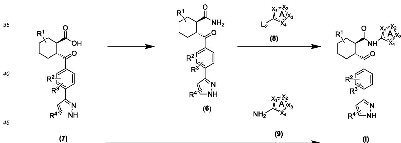
Scheme 2
