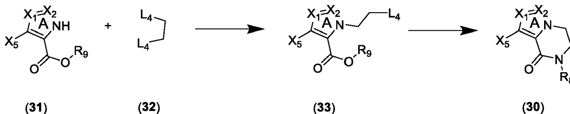
Scheme 10
