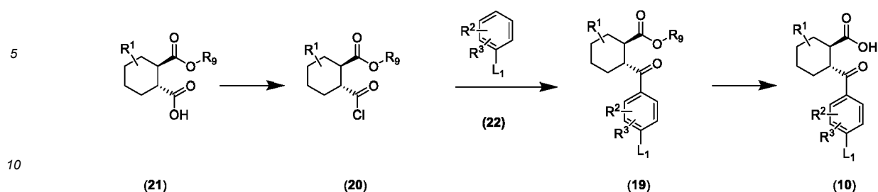
Scheme 7
