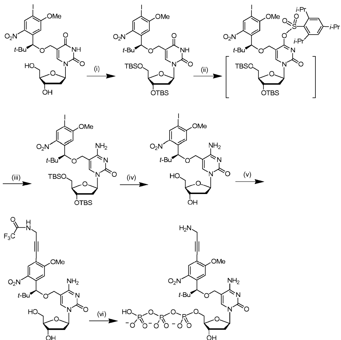
Scheme 5a. Synthesis of dye labeled 5-[( S )-1-(5-methoxy-2-nitrophenyl)-2,2-dimethyl-propyloxy]methyl-2'-deoxycytidine-5'-triphosphate. Reagents and conditions: (i) TBSCl, imidazole, DMF, room temperature; (ii) 2,4,6-triisopropylbenzenesulfonyl chloride, DMAP, Et 3 N, CH 2 Cl 2 , room temperature; (iii) NH 3 , 1,4-dioxane, 90°C; (iv) n -Bu 4 NF, THF, room temperature, 82%; (v) N -propargyltrifluoroacetamide, Pd(PPh 3 ) 4 (0), CuI, Et 3 N, DMF; (vi) POCl 3 , proton sponge, (MeO) 3 PO, 0°C; («-Bu 3 NH) 2 H 2 P 2 O 7 , «-Bu 3 N, DMF; 1 M HNEt 3 HC0 3 .
