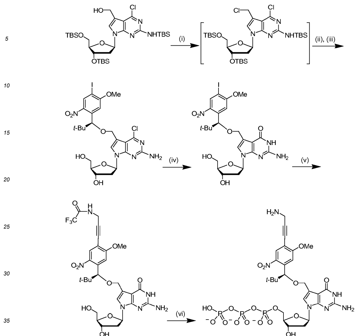
Scheme 4a. Synthesis of dye labeled 7-[(S)-1-(5-methoxy-2-nitrophenyl)-2,2-dimethyl-propyloxy]methyl-7-deaza-2'-deoxyguanosine-5'-triphosphate. Reagents and conditions: (i) \text{MsCl} , DMAP, \text{CH}_2\text{Cl}_2 , 0^\circ\text{C} ; (ii) (5')-1-(4-iodo-5-methoxy-2-nitrophenyl)-2,2-dimethyl-1-propanol, 115^\circ\text{C} ; (iii) n\text{-Bu}_4\text{NF} , THF, room temperature; (iv) syn-pyridine-2-aldoxime, 1,1,3,3-tetramethyl guanidine, 1,4-dioxane/DMF, 70^\circ\text{C} ; (v) N -propargyltrifluoroacetamide, \text{Pd}(\text{PPh}_3)_4(0) , CuI, \text{Et}_3\text{N} , DMF; (vi) \text{POCl}_3 , proton sponge, (\text{MeO})_3\text{PO} , 0^\circ\text{C} ; (n\text{-Bu}_3\text{NH})_2\text{H}_2\text{P}_2\text{O}_7 , n\text{-Bu}_3\text{N} , DMF; 1 M \text{HNEt}_3\text{HCO}_3 .
