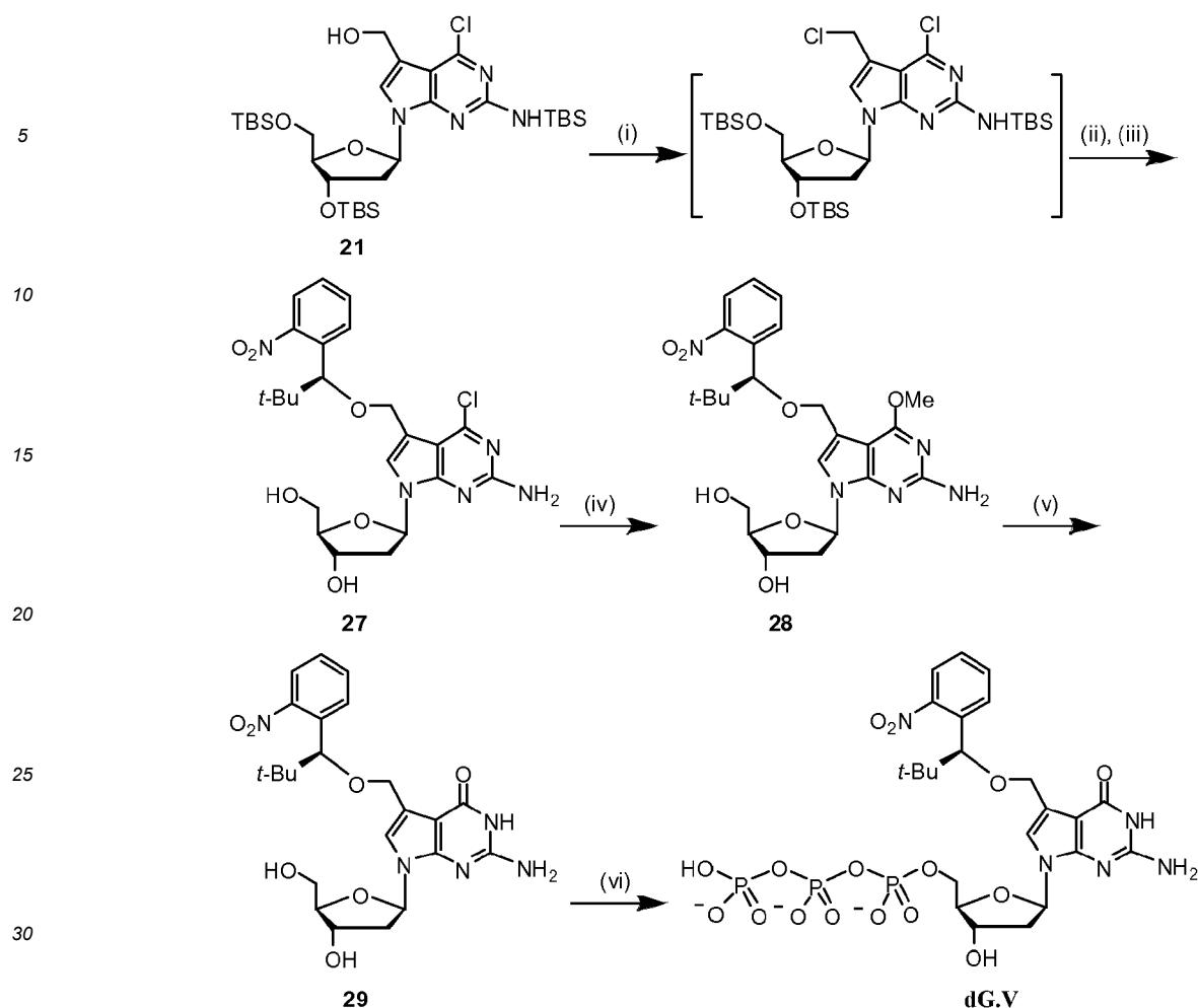
Scheme S14. Synthesis of 7-[(S)-1-(2-nitrophenyl)-2,2-dimethyl-propyloxy]methyl-7-deaza-2'-deoxy-guanosine-5'-triphosphate. Reagents and conditions: (i) MsCl, DMAP, CH 2 Cl 2 , 0°C; (ii) (5'-1-(2-nitrophenyl)-2,2-dimethyl-1-propanol, 115°C; (iii) n -Bu 4 NF, THF, room temperature, 35% for three steps; (iv) NaOMe, MeOH, reflux, 74%; (v) 1,4-dioxane, 2 M NaOH, reflux, 33%; (vi) POCl 3 , proton sponge, (MeO) 3 PO, 0°C; ( n -Bu 3 NH) 2 H 2 P 2 O 7 , n -Bu 3 N, DMF; 1 M HNE i 3 H 2 O 3 .
