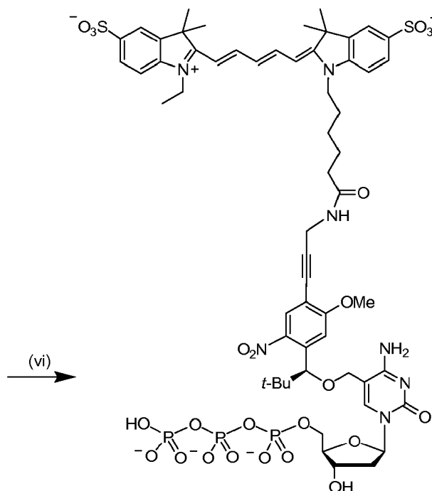
Scheme 5b. (vi) Cy5 NHS, 0.1 M \text{Na}_2\text{CO}_3/\text{NaHCO}_3 buffer (pH 9.2).
