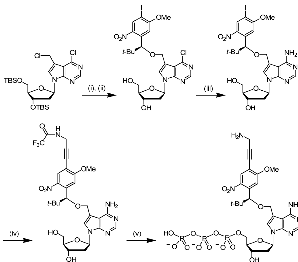
Scheme 2a. Synthesis of dye labeled 7-[(5)-l-(5-methoxy-2-nitrophenyl)-2,2-dimethyl-propyloxy]methyl-7-deaza-2'-deoxyadenosine-5'-triphosphate. Reagents and conditions: (i) 1-(5-methoxy-2-nitrophenyl)-2,2-dimethyl-1-propanol, 110°C; (ii) t -Bu 4 NF, THF, room temperature; (iii) NH 3 , 1,4-dioxane/MeOH, 100°C; (iv) N -propargyltrifluoroacetamide, Pd(PPh 3 ) 4 (0), CuI, Et 3 N, DMF; (v) POCl 3 , (MeO) 3 PO, 0°C; (n -Bu 3 NH) 2 H 2 P 2 O 7 , t -Bu 3 N, DMF; 1 M HNEt 3 HC0 3 .
