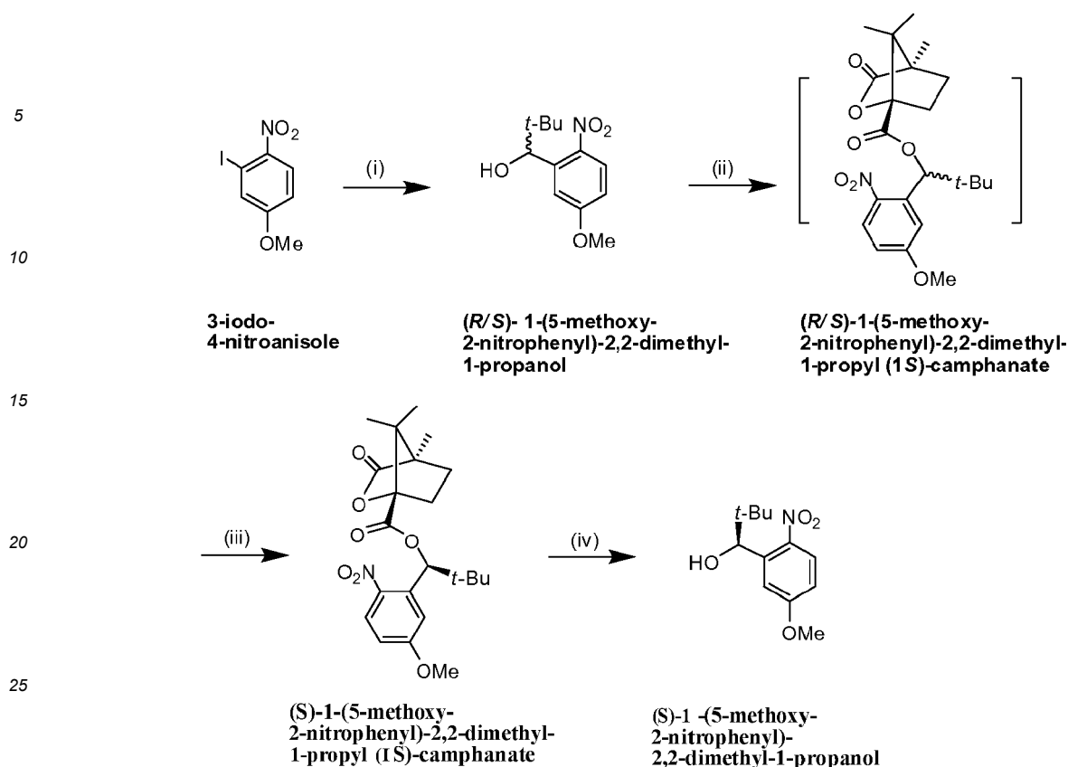
Scheme S4. Synthesis of (R/S)-1-(5-methoxy-2-nitrophenyl)-2,2-dimethyl-1-propanol and (S)-1-(5-methoxy-2-nitrophenyl)-2,2-dimethyl-1-propanol.
