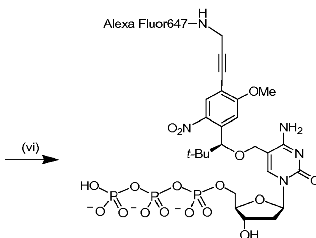
Scheme 5c. (vi) Alexa Fluor 647 NHS, 0.1 M \text{Na}_2\text{CO}_3/\text{NaHCO}_3 buffer (pH 9.2).
