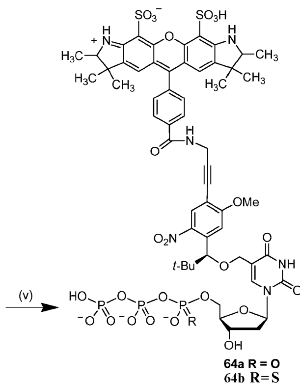
Scheme S27b. (v) Alexa Fluor 532 NHS, 0.1 M \text{NaHCO}_3/\text{Na}_2\text{CO}_3 buffer (pH 9.2).
