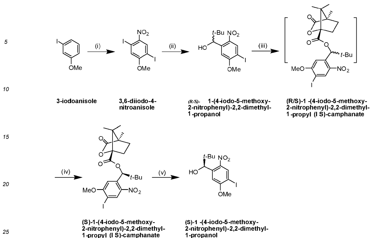
Scheme S23. Synthesis of (R/S) -1-(4-iodo-5-methoxy-2-nitrophenyl)-2,2-dimethyl-1-propanol and (S) -1-(4-iodo-5-methoxy-2-nitrophenyl)-2,2-dimethyl-1-propanol. (i) \text{NaNO}_2 , \text{CH}_3\text{COOH} , \text{HNO}_3 , room temperature; \text{I}_2 , 60^\circ\text{C} , 25% for two steps (80% pure); (ii) \text{PhMgCl} , (\text{CH}_3)_3\text{CCHO} , THF, minus 40^\circ\text{C} to room temperature, 72%; (iii) (T5)-camphanic acid chloride, DMAP, \text{CH}_2\text{Cl}_2 , room temperature, 80%; (iii) fractional crystallization from ethanol, 63%; (iv) \text{K}_2\text{CO}_3 , MeOH, reflux.
