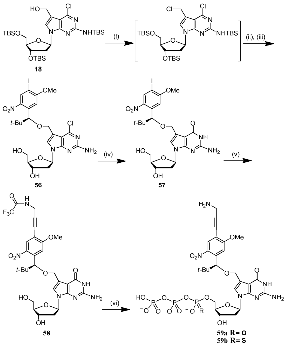
Scheme S26a. Synthesis of dye labeled 7-((S)-1-[4-(3-amino-1-propynyl)-5-methoxy-2-nitrophenyl]-2,2-dimethyl-propyloxy)methyl-7-deaza-2'-deoxyguanosine-5'-triphosphate and 5'-a-thiotriphosphate. Reagents and conditions: (i) MsCl, DMAP, \text{CH}_2\text{Cl}_2 , 0^\circ\text{C} ; (ii) (5)-1-(4-iodo-5-methoxy-2-nitrophenyl)-2,2-dimethyl-1-propanol, 115^\circ\text{C} ; (iii) \text{t-Bu}_4\text{NF} , THF, room temperature; 18% for three steps; (iv) syn-pyridine-2-aldoxime, 1,1,3,3-tetramethyl guanidine, 1,4-dioxane/DMF, 70^\circ\text{C} , 72%; (v) N -propargyltrifluoroacetamide, \text{Pd}(\text{PPh}_3)_4(0) , CuI, \text{Et}_3\text{N} , DMF, 96%; (vi) For 59a : \text{POCl}_3 ,
