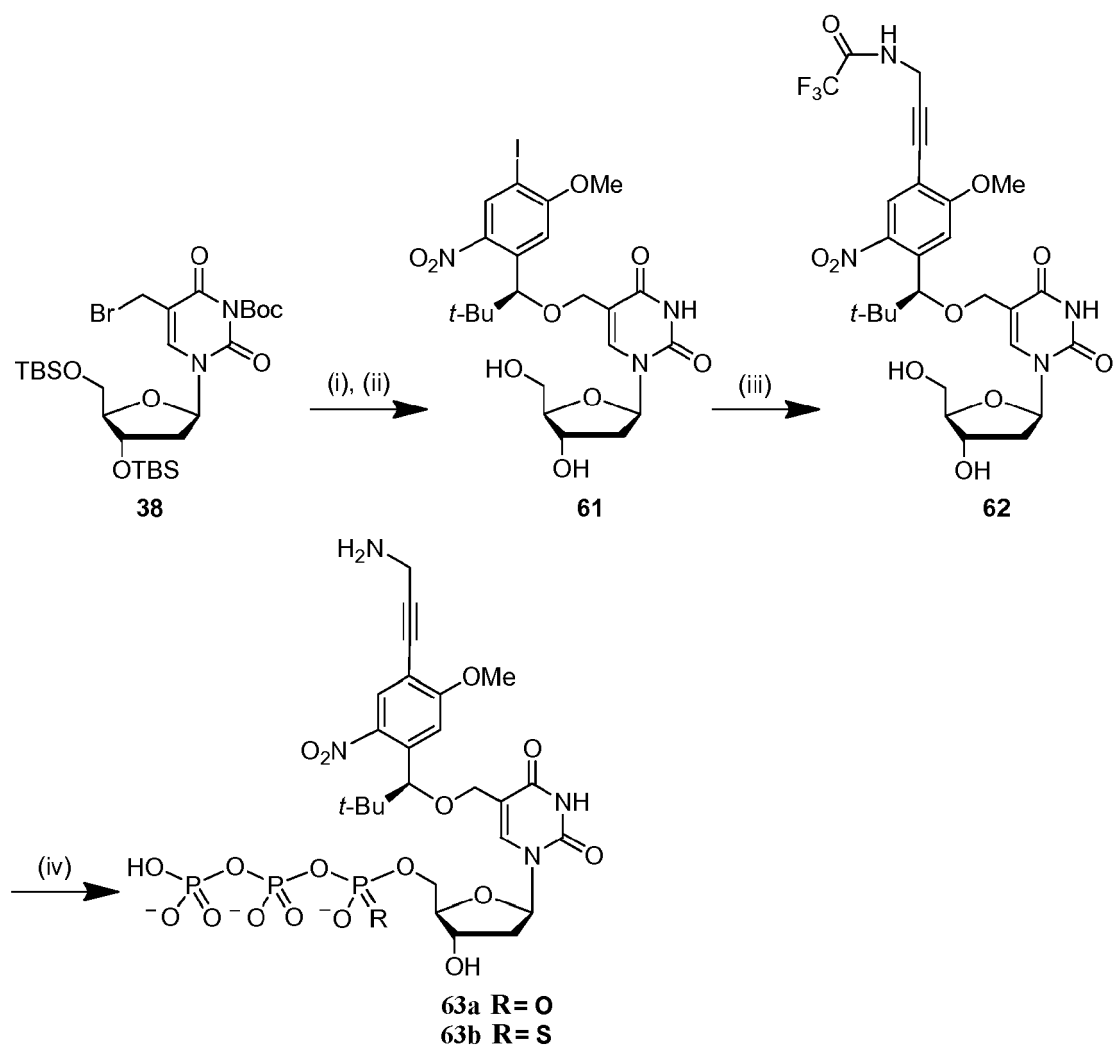
Scheme S27a. Synthesis of dye labeled 5-((S)-1-[4-(3-amino-1-propynyl)-5-methoxy-2-nitrophenyl]-2,2-dimethyl-propoxy)methyl-2'-deoxyuridine-5'-triphosphate. Reagents and conditions: (i) (5)-1-(4-iodo-5-methoxy-2-nitrophenyl)-2,2-dimethyl-1-propanol, 110°C; (ii) \text{NH}_4\text{F} , MeOH, 50°C, 28% for two steps; (iii) N -propargyltrifluoroacetamide, \text{Pd}(\text{PPh}_3)_4(0) , CuI, \text{Et}_3\text{N} , DMF, 90%; (iv) For 63a : \text{POCl}_3 , proton sponge, (\text{MeO})_3\text{PO} , 0°C; (\text{t-Bu}_3\text{NH})_2\text{H}_2\text{P}_2\text{O}_7 , \text{t-Bu}_3\text{N} , DMF; 1 M \text{HNEt}_3\text{HCl} ; \text{NH}_4\text{OH} . For 63b : \text{PSCl}_3 , 2,6-lutidine, (\text{EtO})_3\text{PO} , 0°C to room temperature; (\text{t-Bu}_3\text{NH})_2\text{H}_2\text{P}_2\text{O}_7 , \text{t-Bu}_3\text{N} , DMF; 1 M \text{HNEt}_3\text{HCl} ; \text{NH}_4\text{OH} .
