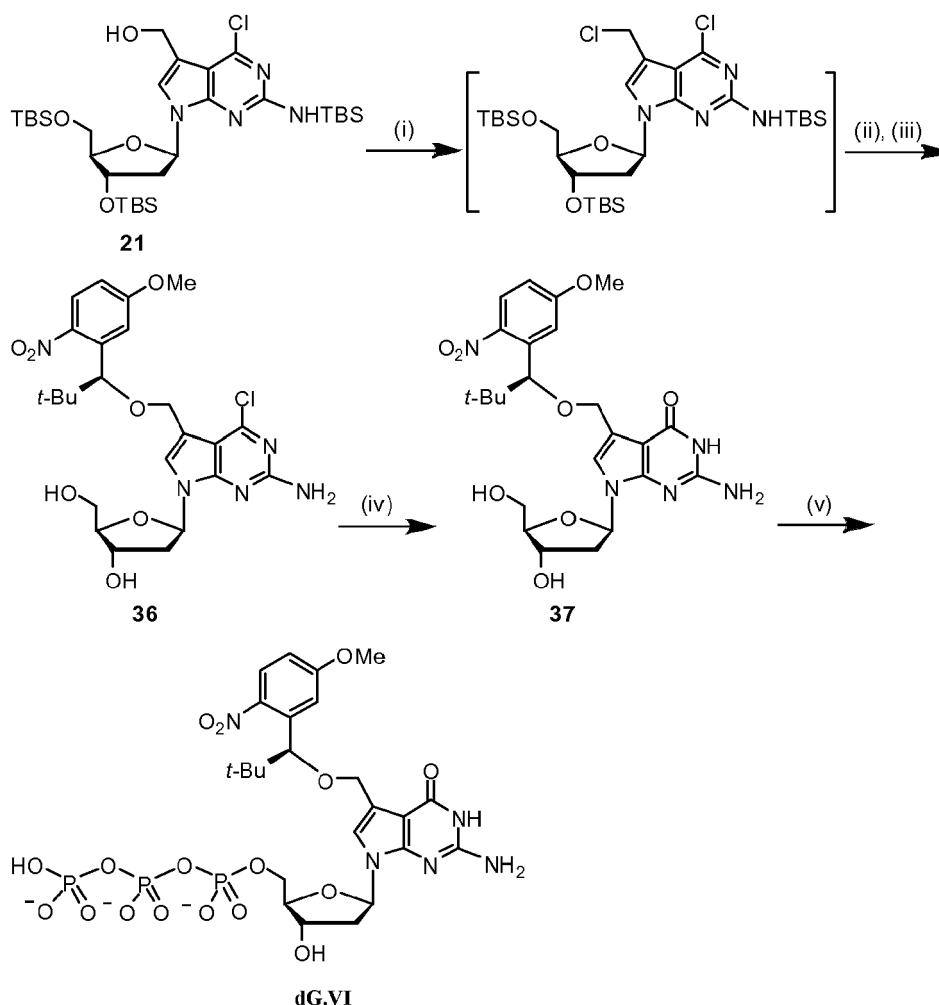
Scheme S18. Synthesis of 7-[(S)-1-(5-methoxy-2-nitrophenyl)-2,2-dimethyl-propoxy]methyl-7-deaza-2'-deoxyguanosine-5'-triphosphate. Reagents and conditions: (i) MsCl, DMAP, CH 2 Cl 2 , 0°C; (ii) (5)-1-(5-methoxy-2-nitrophenyl)-2,2-dimethyl-1-propanol, 115°C; (iii) n -Bu 4 NF, THF, room temperature, 27% for three steps; (iv) syn-pyrimidine-2-aldoxime, 1,1,3,3-tetramethyl guanidine, 1,4-dioxane/DMF, 70°C, 76%; (v) POCl 3 , proton sponge, (MeO) 3 PO, 0°C; («-Bu 3 NH) 2 H 2 P 2 O 7 , «-Bu 3 N, DMF; 1 M HNEt 3 HCO 3 .
