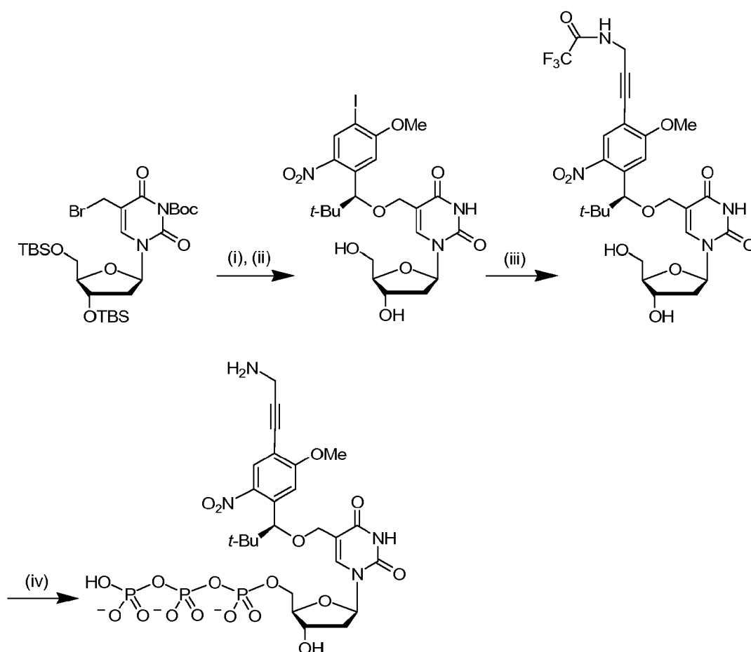
Scheme 3a. Synthesis of dye labeled 5-[(S)-1-(5-methoxy-2-nitrophenyl)-2,2-dimethyl-propyloxy]methyl-2'-deoxyuridine-5'-triphosphate. Reagents and conditions: (i) (5)-1-(4-iodo-5-methoxy-2-nitrophenyl)-2,2-dimethyl-1-propanol, 110°C; (ii) NH 4 F, MeOH, 50°C;
