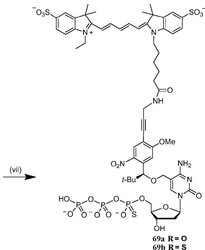
Scheme S28b. (vii) Cy5 NHS, 0.1 M \text{Na}_2\text{CO}_3/\text{NaHCO}_3 buffer (pH 9.2).
