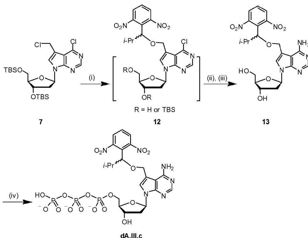
Scheme S9. Synthesis of 7-[1-(2,6-dinitrophenyl)-2-methyl-propyloxy]methyl-7-deaza-2'-deoxy-adenosine-5'-triphosphate. Reagents and conditions: (i) racemic ( R / S )-1-(2,6-dinitrophenyl)-2-methyl-1-propanol, 108°C; (ii) n -Bu 4 NF, THF, 0°C to room temperature; (iii) «0 NH 3 , 1,4-dioxane/MeOH, 100°C, 38% for three steps; (iv) POCl 3 , (MeO) 3 PO, 0°C; ( n -Bu 3 NH) 2 H 2 P 2 O 7 , «-Bu 3 N, DMF; 1 M HNEt 3 HClO 3 .
