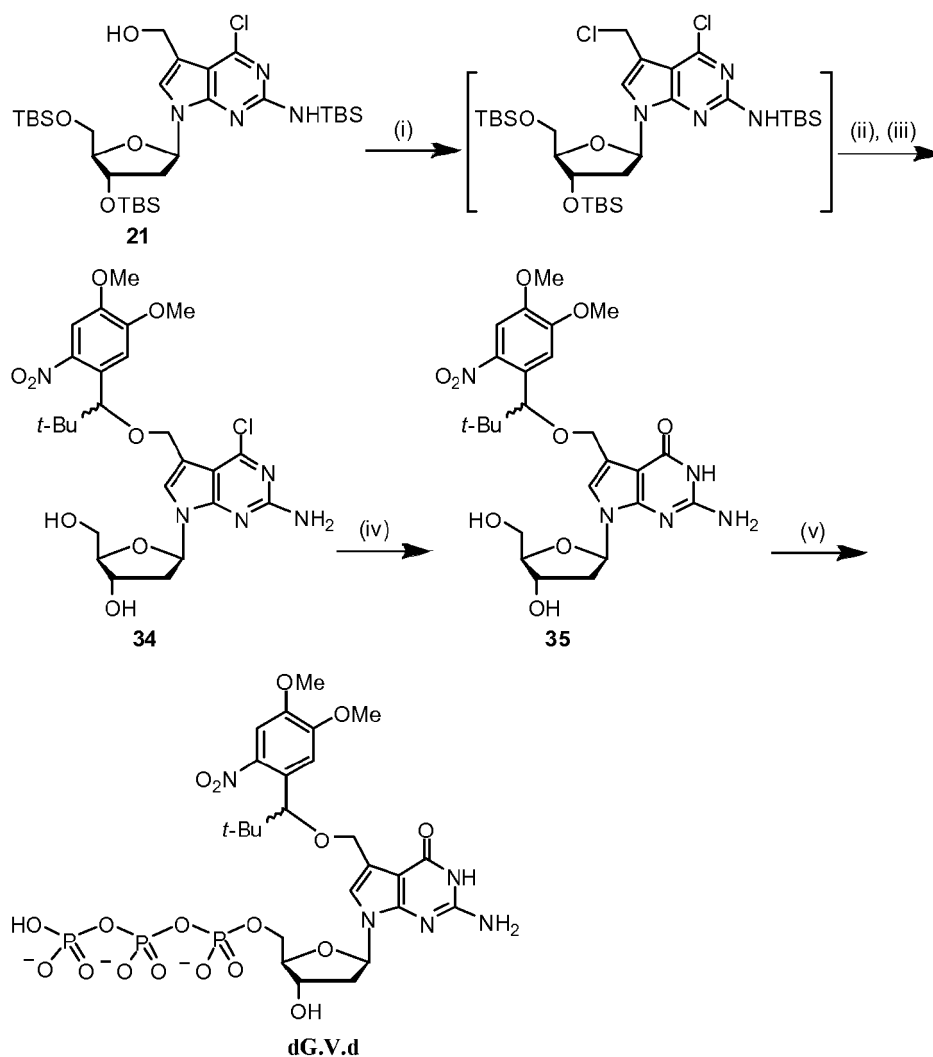
Scheme S17. Synthesis of 7-[1-(4,5-dimethoxy-2-nitrophenyl)-2,2-dimethyl-propyloxy]methyl-7-deaza-2'-deoxyguanosine-5'-triphosphate. Reagents and conditions: (i) MsCl, DMAP, CH 2 Cl 2 , 0°C; (ii) racemic (R/S)-1-(4,5-dimethoxy-2-nitrophenyl)-2,2-dimethyl-1-propanol, 115°C; (iii) n -Bu 4 NF, THF, room temperature, 23% for three steps; (iv) syn-pyridine-2-aldoxime, 1,1,3,3-tetramethyl guanidine, dioxane/DMF, 70°C, 68%; (v) POCl 3 , proton sponge, (MeO) 3 PO, 0°C; ( n -B 3/4 NH) 2 H 2 P 207, «-Bu 3 N, DMF; 1 M HNEt 3 HCO 3 .
