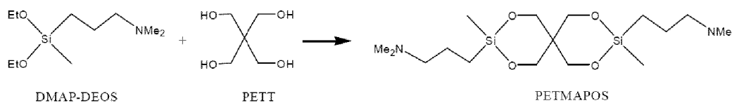
Figure 3. Synthesis of PETMAPOS
