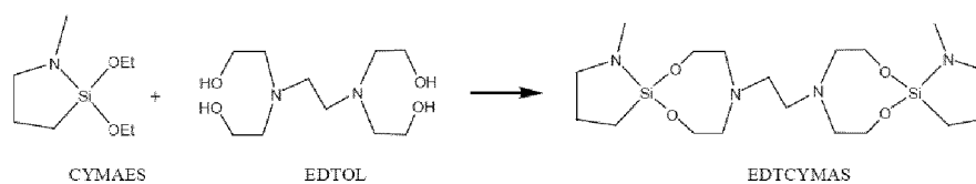
Figure 4. Synthesis of EDTCYMAS
