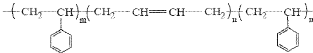
Molecular structure of SBS
