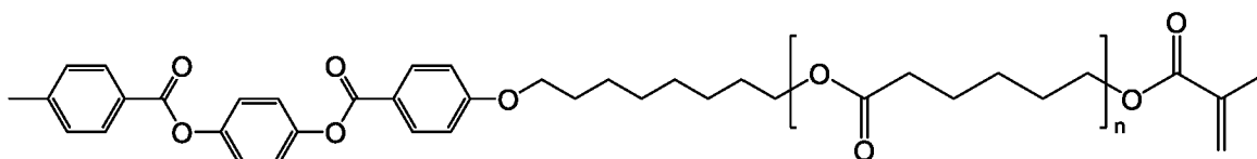
4-((4-((8-((6-(methacryloyloxy)hexanoyl)oxy)octyl)oxy)benzoyl)oxy)phenyl 4-methylbenzoate with n=8 (Compound (4));
