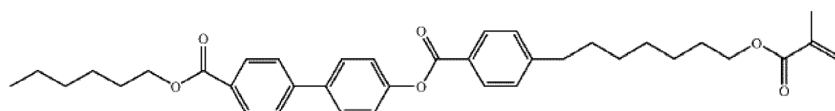
1-{3-(4-(3-(4-(6-(4-(4-(6-methacryloyloxy)hexyloxy)benzoyloxy)phenyl)benzoyloxy)hexyloxy)- 4-oxobutyl)oxy}propyl)benzoyloxy}butane-1,4-dione
