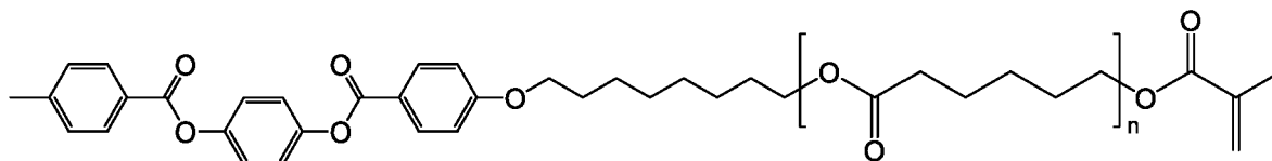
4-((4-((8-((6-(methacryloyloxy)hexanoyl)oxy)octyl)oxy)benzoyl)oxy)phenyl 4-methylbenzoate
