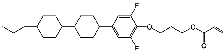
3-(2,6-difluoro-4-(4'-propyl-[1,1'-bi(cyclohexan)]-4-yl)phenoxy)propyl acrylate
