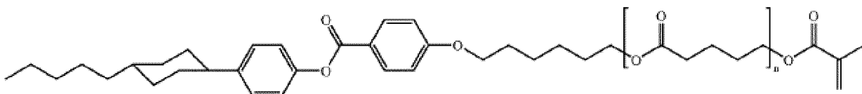
1-(5-(5-(5-(5-(6-(4-(4-(trans-4-pentylcyclohexyl)phenoxy)carbonyl)phenoxy)hexyloxy)-5-oxopentylloxy)-5-oxopentylloxy)-5-oxopentylloxy)-5-oxopentylloxy)-2-methylprop-2-en-1-one
