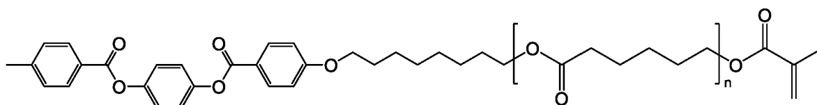
4-((4-((8-((6-(methacryloyloxy)hexanoyl)oxy)octyl)oxy)benzoyl)oxy)phenyl 4-methylbenzoate
