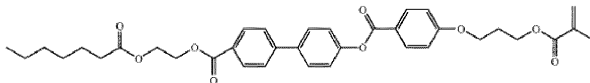
1,12-bis[2-(4-(4-(3-(methacryloyloxy)propyloxy)benzoyloxy)phenyl)benzoyloxy]ethoxy dodecyl-1,12-dione
