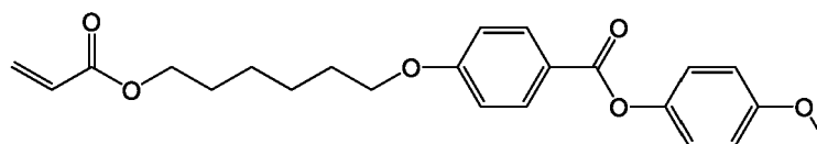
4-methoxyphenyl 4-((6-(acryloyloxy)hexyl)oxy)benzoate
