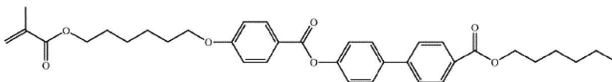
1,12-bis(6-(4-(4-(4-(6-methacryloyloxy)hexyloxy)benzoyloxy)phenyl)benzoyloxy)hexyloxy) dodecyl-1,12-dione
