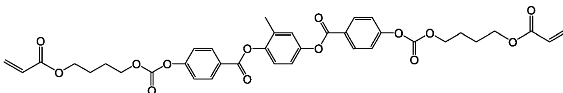
2-methyl-1,4-phenylene bis(4-(((4-(acryloyloxy)butoxy)carbonyl)oxy)benzoate)
