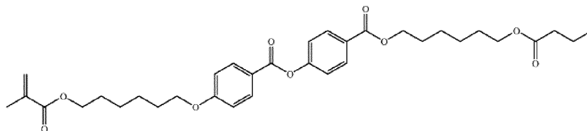
1,10-bis(6-(4-(4-(4-(6-methacryloyloxy)hexyloxy)benzoyloxy)phenyl)benzoyloxy)hexyloxy) 2,2,3,3,4,4,5,5,6,6,7,7,8,8,9,9-hexadecafluorodecyl-1,10-dione
