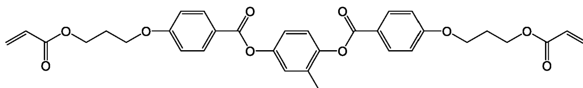
2-methyl-1,4-phenylene bis(4-(3-(acryloyloxy)propoxy)benzoate)
