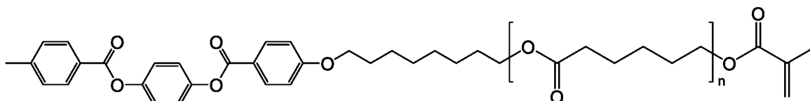
4-((4-((8-((6-(methacryloyloxy)hexanoyl)oxy)octyl)oxy)benzoyl)oxy)phenyl 4-methylbenzoate with n=3 (Compound (5)); 4-((4-pentylcyclohexane-1-carbonyl)oxy)phenyl 4-((6-(acryloyloxy)hexyl)oxy)benzoate (Compound (6)); 3-(3,6-difluoro-4-(4'-propyl-[1,1'-bi(cyclohexan)])-4-yl)phenoxy)propyl acrylate (Compound (7)); or a combination of any of the foregoing.
