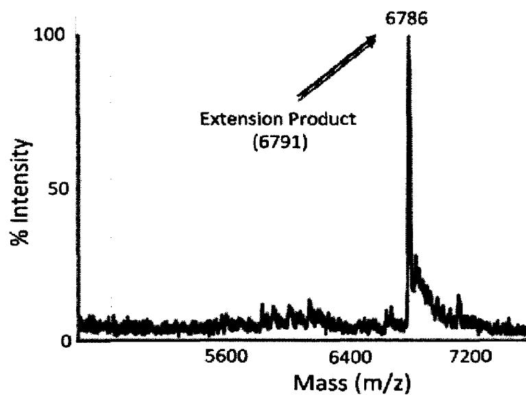
Extension Reaction with dG4P-PEG24
