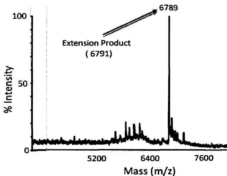
Extension Reaction with dG4P-PEG37
