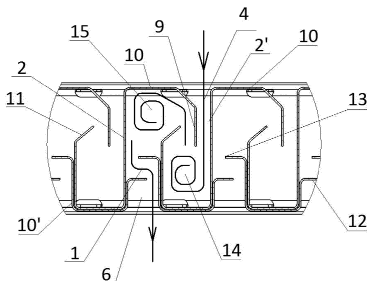
DETAIL C
