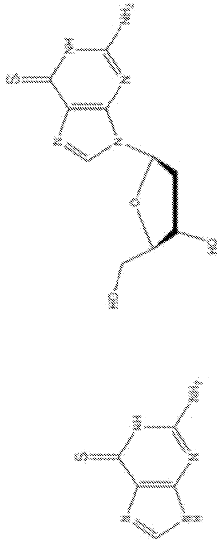
6-thio-2'-deoxyguanosine
