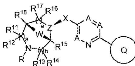
Formula (V)
