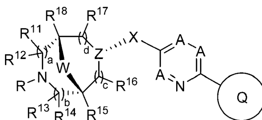
Formula (IV)
