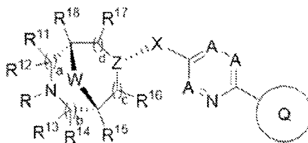
Formula (IV)
