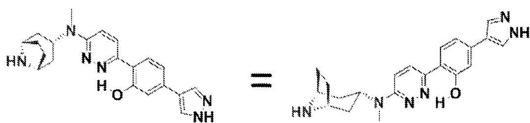
Compound 1
