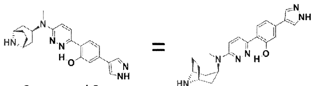
Compound 2
