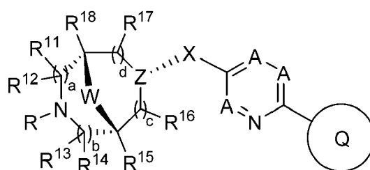
Formula (IV)
