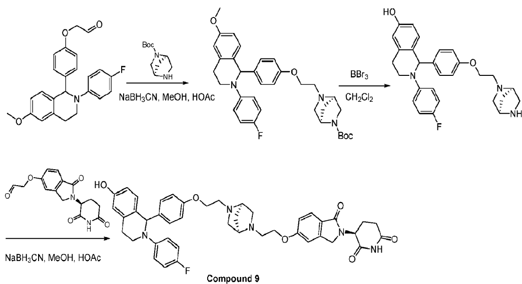
General synthetic scheme 3-7.
