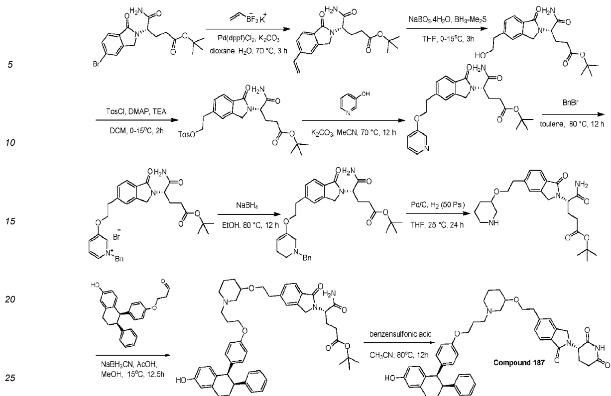
General synthetic scheme 3-35.
