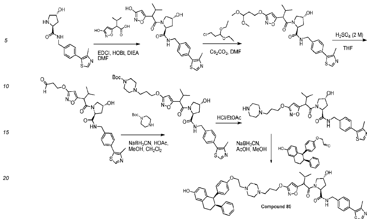
General synthetic scheme 3-19.
