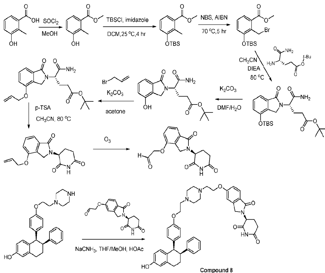
General synthetic scheme 3-6.
