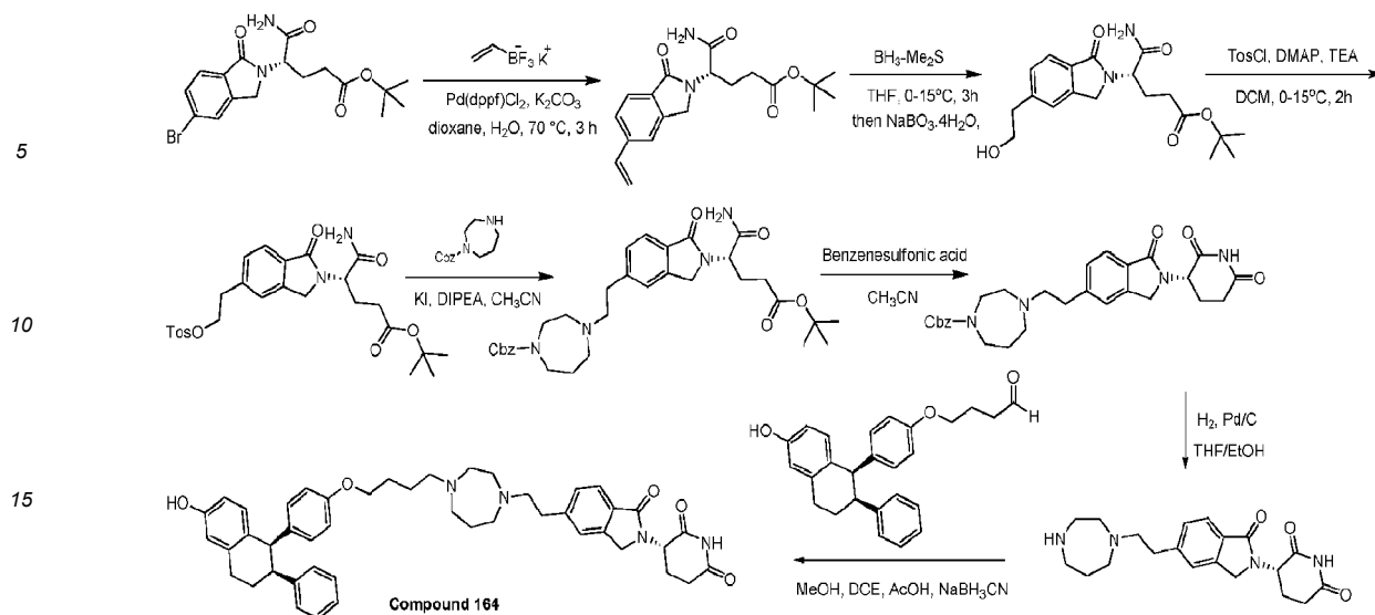
General synthetic scheme 3-30.
