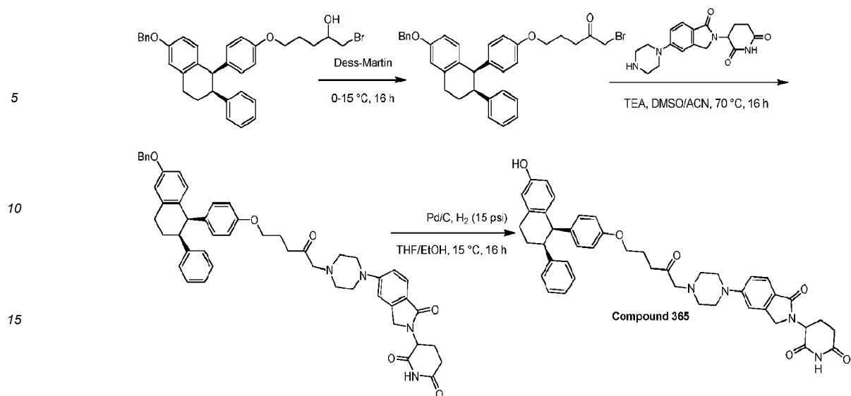
20 General synthetic scheme 3-63.
