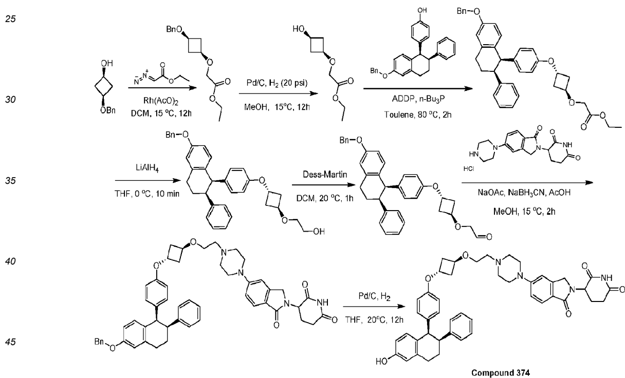
50 General synthetic scheme 3-64.
