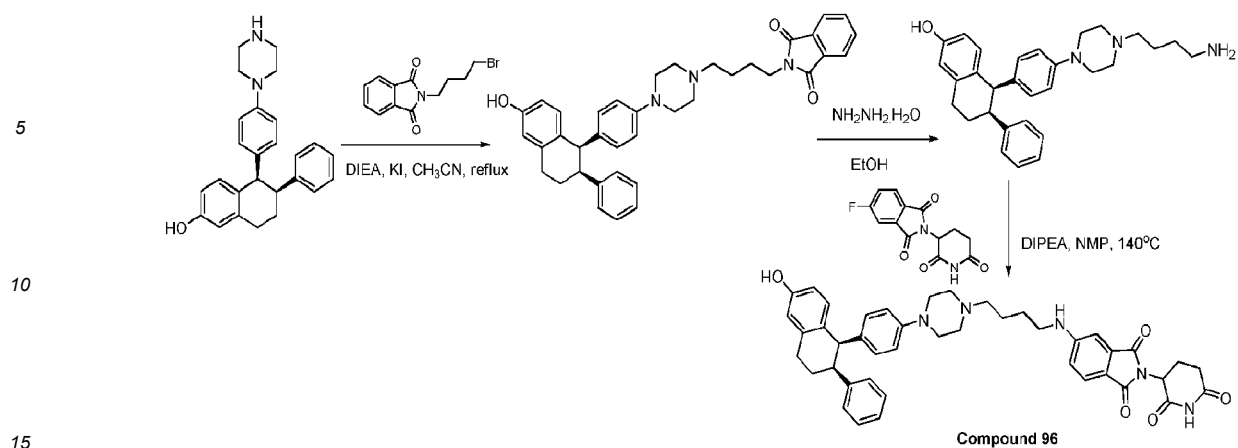
General synthetic scheme 3-21.
