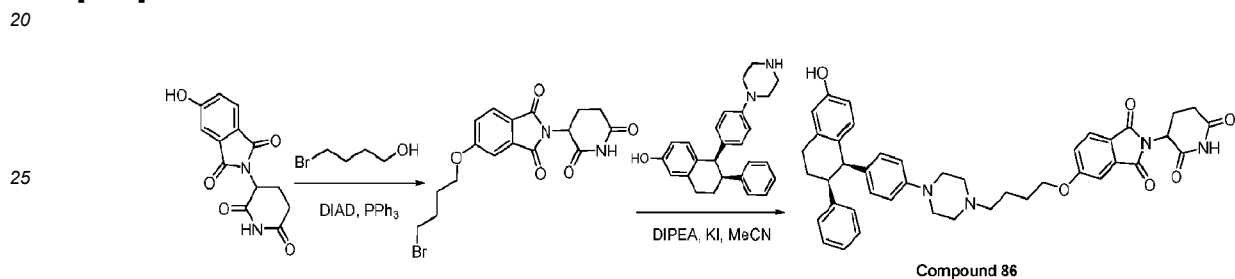
General synthetic scheme 3-22.
