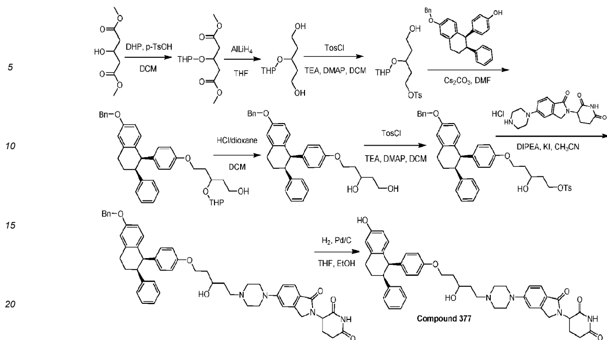
General synthetic scheme 3-65.
