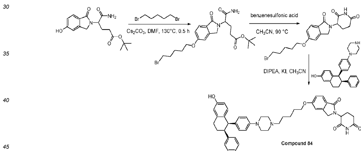
General synthetic scheme 3-20.
