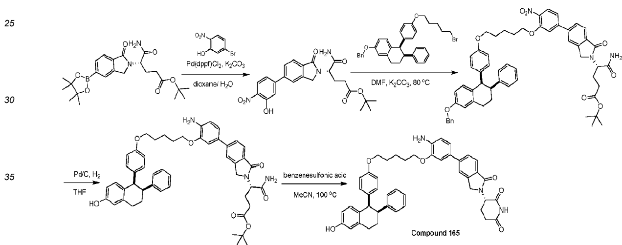
General synthetic scheme 3-31.
