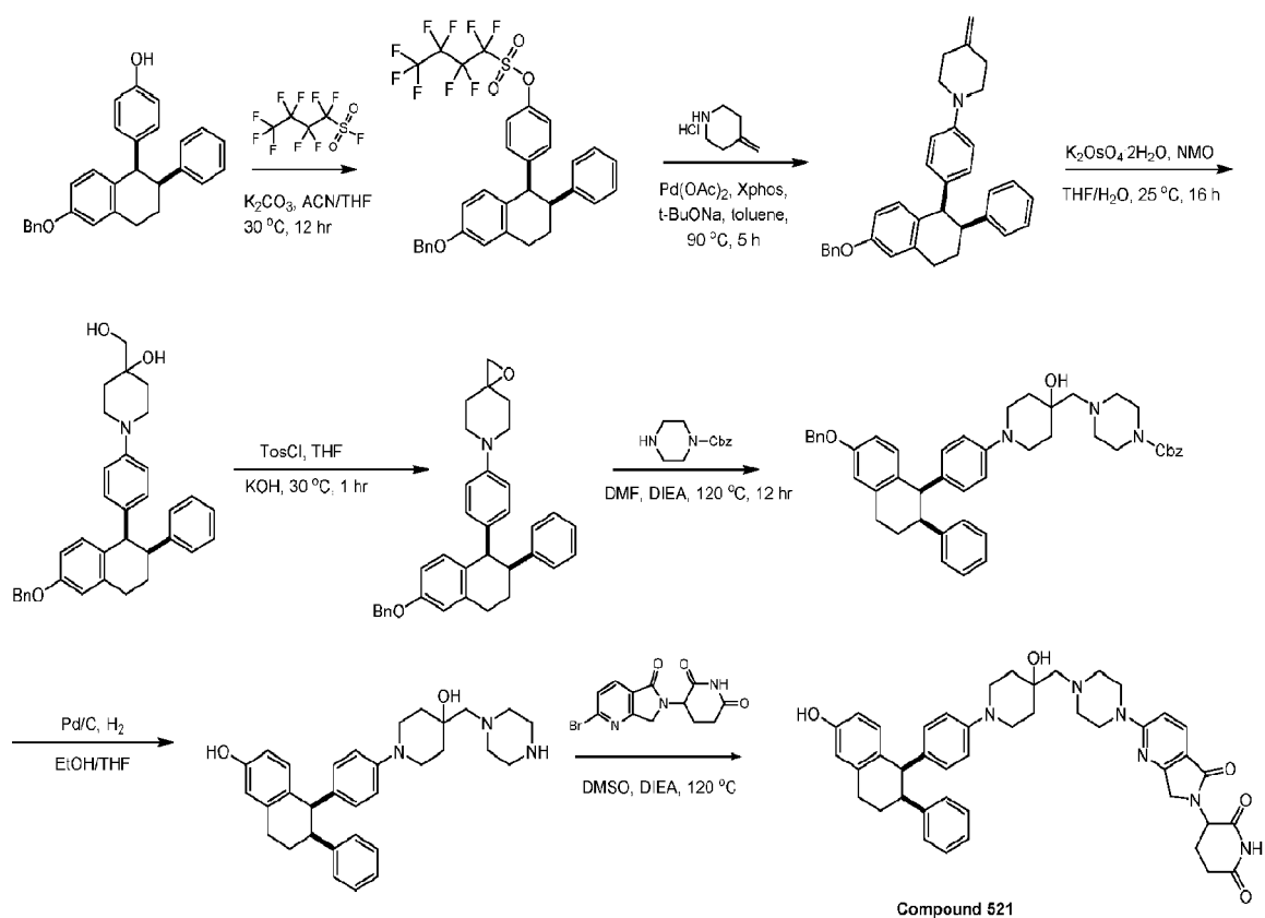
General synthetic scheme 3-82.
