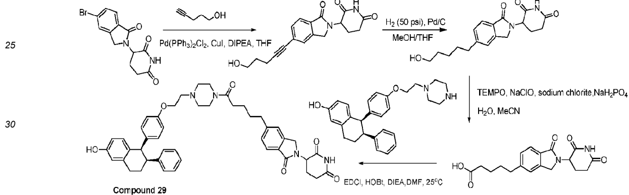
General synthetic scheme 3-13.
