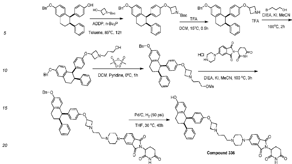
General synthetic scheme 3-58.
