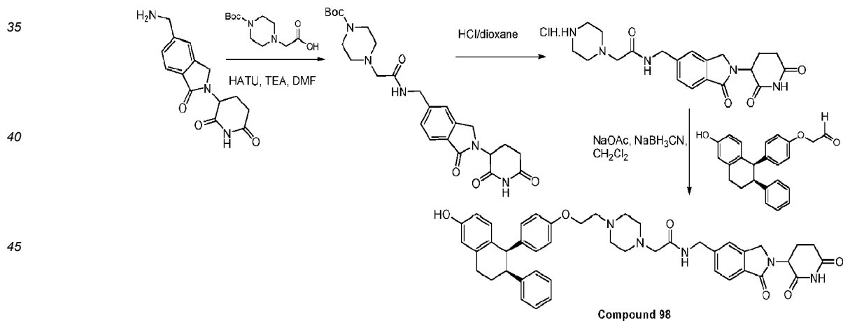
General synthetic scheme 3-23.
