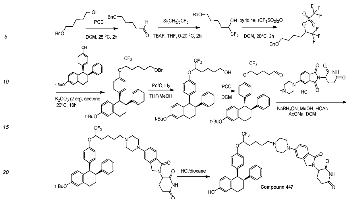
General synthetic scheme 3-71.
