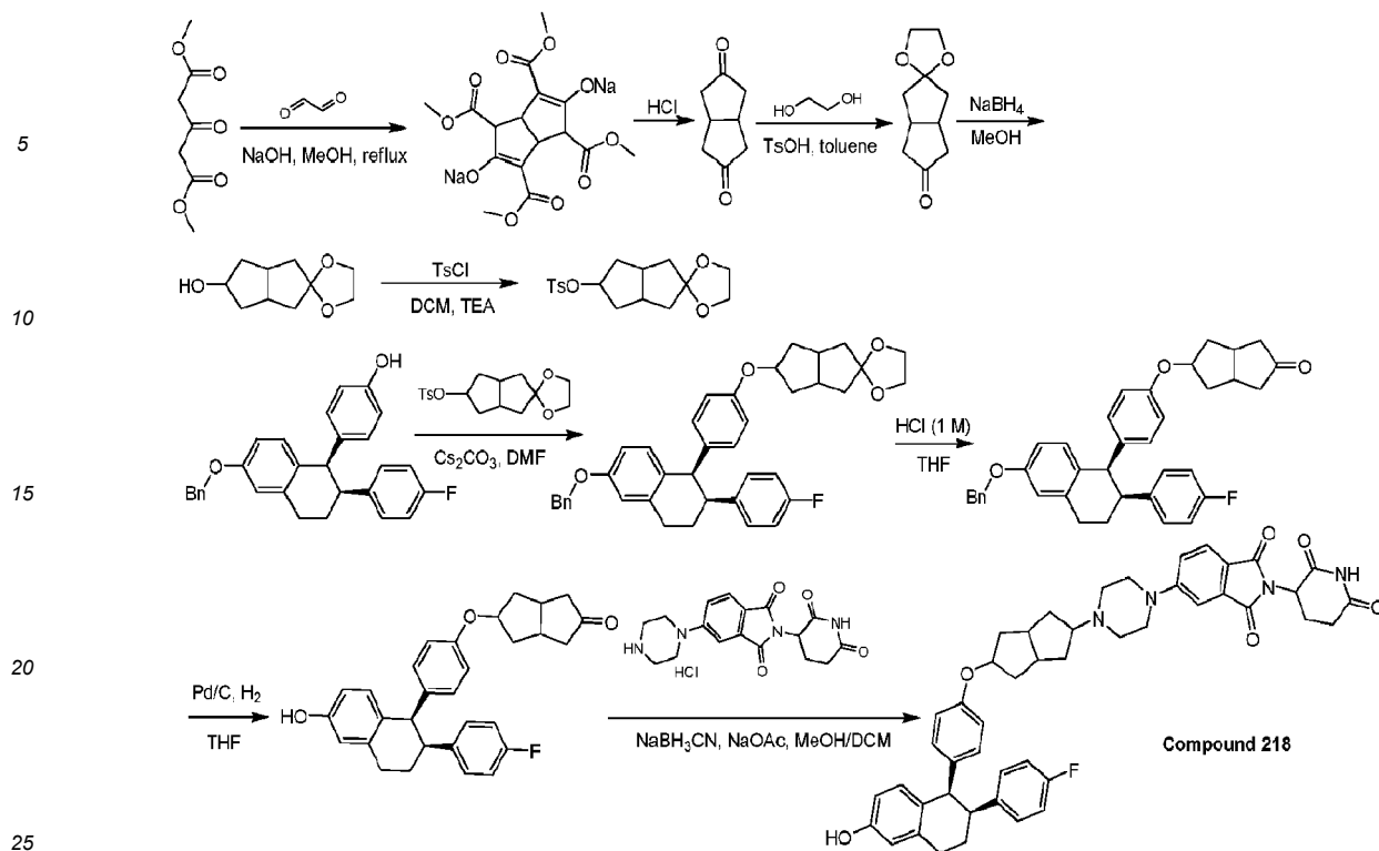
General synthetic scheme 3-42.
