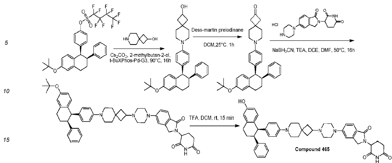
General synthetic scheme 3-74.
