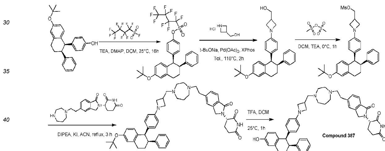
General synthetic scheme 3-66.
