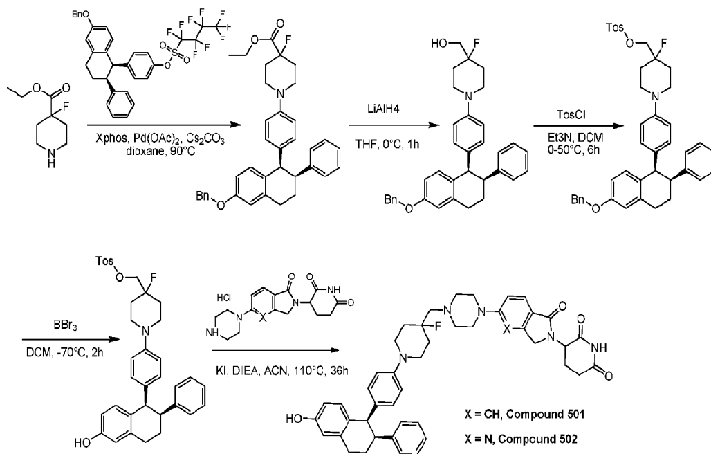
General synthetic scheme 3-78.
