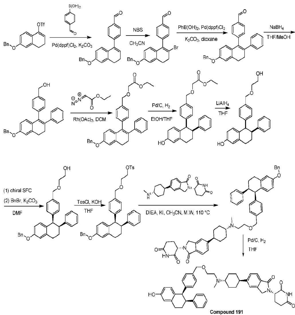
General synthetic scheme 3-36.
