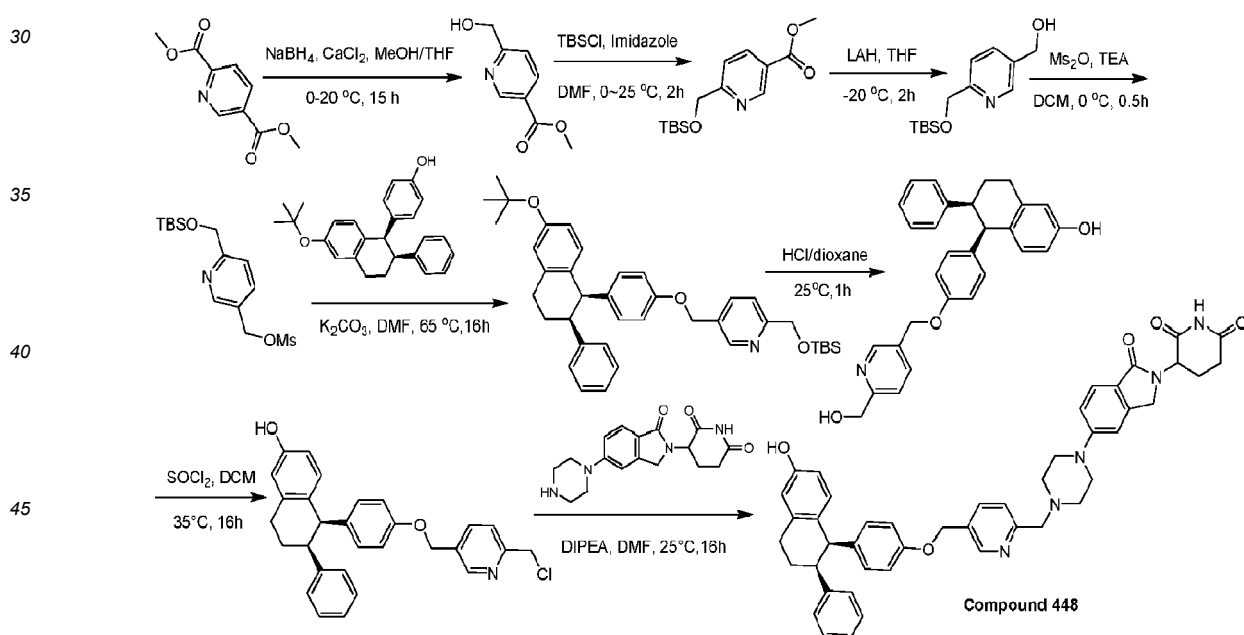
General synthetic scheme 3-73.
