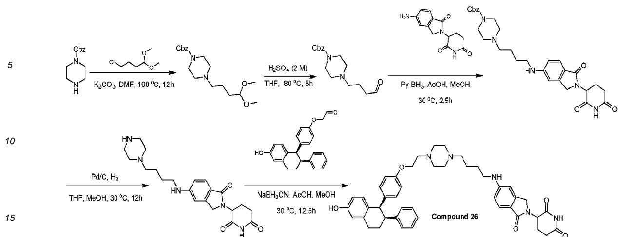
General synthetic scheme 3-12.
