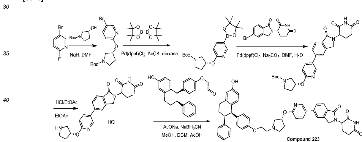
General synthetic scheme 3-43.
