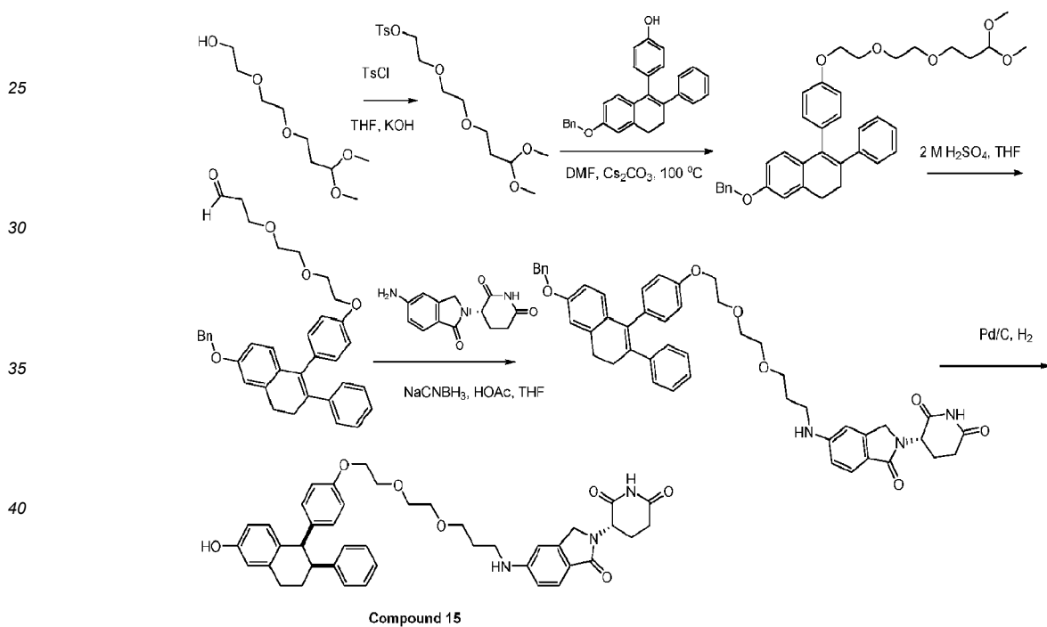
General synthetic scheme 3-9.
