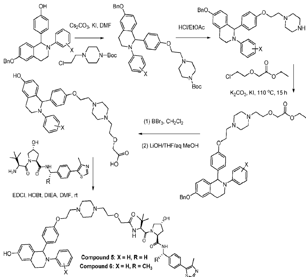
General synthetic scheme 3-5.
