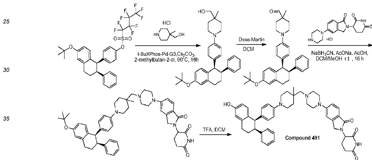
General synthetic scheme 3-75.
