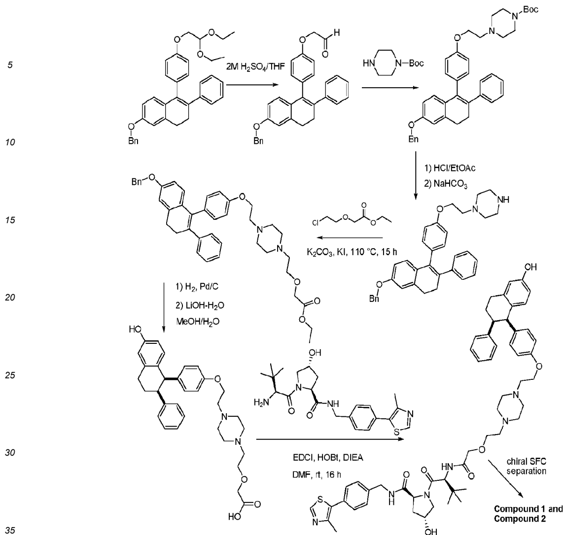
General synthetic scheme 3-3.
