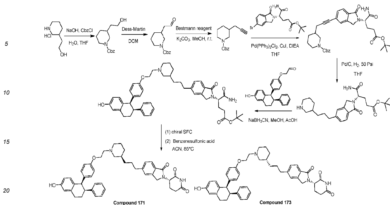
General synthetic scheme 3-32.
