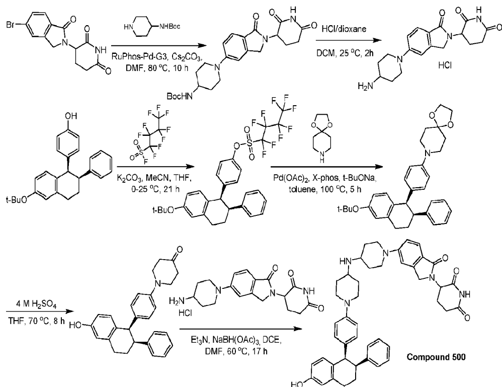
General synthetic scheme 3-77.
