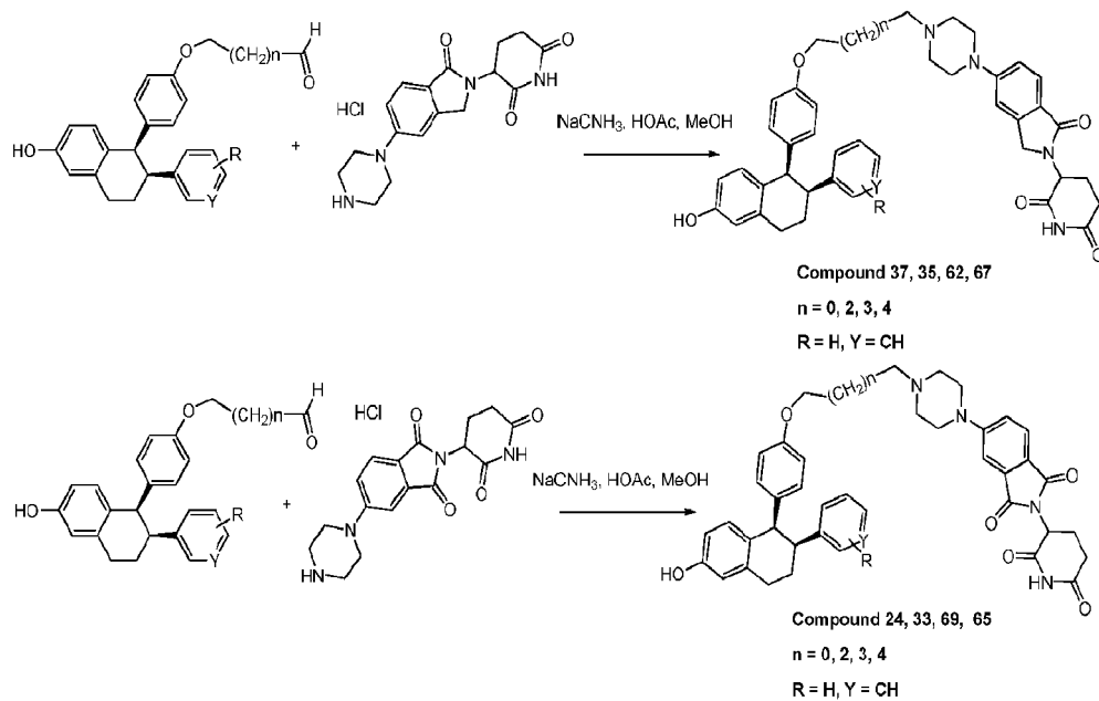
General synthetic scheme 3-11.
