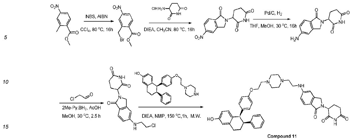
General synthetic scheme 3-8.
