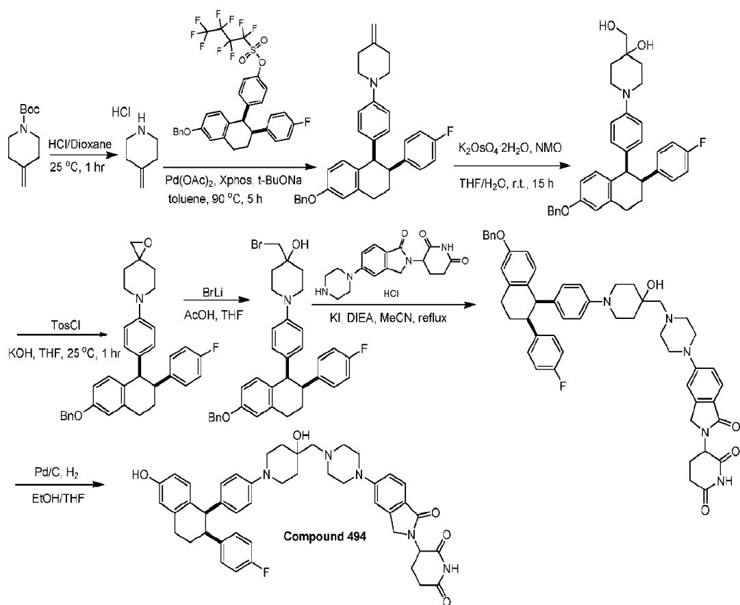
General synthetic scheme 3-76.
