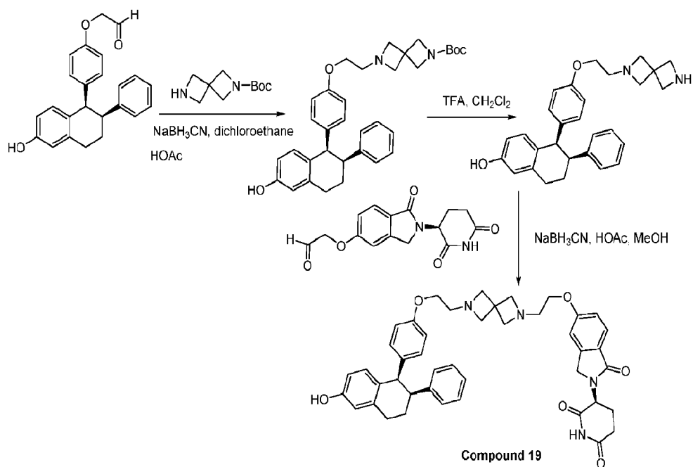
General synthetic scheme 3-10.
