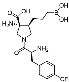
Trifluoromethyl phenylalanine AUC = 5783
