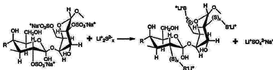
[Reaction Scheme 1]
