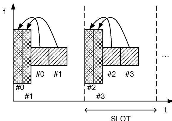
FIG. 4A CORESET CONFIGURATION BIT = 00
