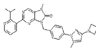
1-109. 9-(4-(3-azetidin-1-yl)-5-methyl-1H-pyrazol-1-yl)benzyl)-2-(2-isopropylpyridin-3-yl)-7-methyl-7,8-dihydro-8H-purin-6-one
