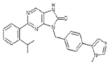
1-251. 2-(2-isopropylphenyl)-9-(4-(1-methyl-1H-imidazol-5-yl)benzyl)-7,8-dihydro-8H-purin-6-one
