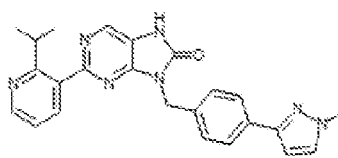
1-46. 2-(2-isopropylpyridin-3-yl)-9-(4-(1-methyl-1H-pyrazol-3-yl)benzyl)-7,8-dihydro-8H-purin-8-one
