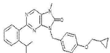
I-228. 9-(1-(cyclopropylmethoxy)benzyl)-2-(2-isopropylphenyl)-7,8-dihydro-8H-purin-6-one
