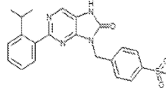
1-183. 2-(2-isopropylphenyl)-9-(4-(methylsulfonyl)benzyl)-7,8-dihydro-8H-purin-6-one
