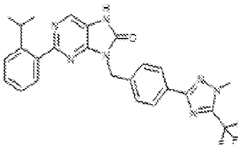
1-293. 2-(2-isopropylphenyl)-5-(4-(1-methyl-5-(trifluoromethyl)-1H-1,2,4-triazol-3-yl)benzyl)-7,8-dihydro-8H-purin-6-one
