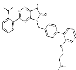
I-258. 9-((2'-(2-(dimethylamino)ethoxy)-[1,1'-biphenyl]-4-yl)methyl)-2-(2-isopropylphenyl)-7-methyl-7,8-dihydro-8H-purin-6-one
