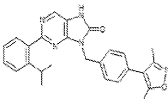
1-253. 9-(4-(3,5-dimethylisoxazol-4-yl)benzyl)-2-(2-isopropylphenyl)-7,8-dihydro-8H-purin-6-one
