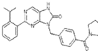
1-390. 2-(2-isopropylphenyl)-3-(4-(2-methylpiperidine-1-carbonyl)benzyl)-7,8-dihydro-8H-purin-6-one
