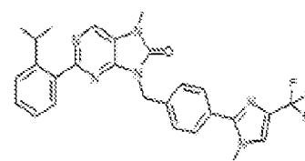
1-63. 2-(2-isopropylphenyl)-7-methyl-9-(4-(1-methyl-4-(trifluoromethyl)-1H-imidazol-2-yl)benzyl)-7,9-dihydro-8H-purin-8-one
