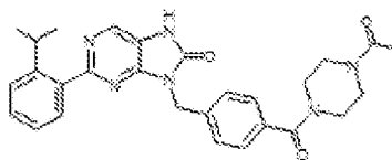
1-383. 5-(4-(4-acetyl)piperazine-1-carbonyl)benzyl)-2-(2-isopropylphenyl)-7,8-dihydro-8H-purin-6-one
