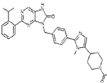
I-473: 9-(4-(5-(1-acetylpiperidin-4-yl)-1-methyl-1H-imidazol-2-yl)benzyl)-2-(2-isopropylphenyl)-7,9-dihydro-8H-purin-6-one
