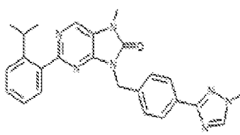
1-272. 2-(2-isopropylphenyl)-7-methyl-9-(4-(1-methyl-1H-1,2,4-triazol-3-yl)benzyl)-7,8-dihydro-8H-purin-6-one
