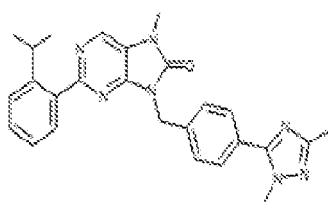
1-283. 5-(4-(1,3-dimethyl-1H-1,2,4-triazol-5-yl)benzyl)-2-(2-isopropylphenyl)-7-methyl-7,8-dihydro-8H-purin-6-one
