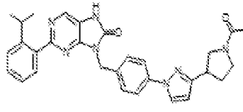
I-467: 9-(4-(3-(1-acetylpiperidin-3-yl)-1H-pyrazol-1-yl)benzyl)-2-(2-isopropylphenyl)-7,9-dihydro-8H-purin-6-one
