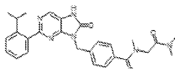
1-380. N-(2-(dimethylamino)-2-oxoethyl)-4-((2-(2-isopropylphenyl)-8-oxo-7,8-dihydro-8H-purin-9-yl)methyl)-N-methylbenzamide
