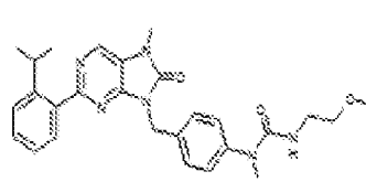
1-485. 1-(4-(2-(2-isopropylphenyl)-7-methyl-8-oxo-7,8-dihydro-6H-purin-5-yl)methylphenyl)-3-(2-methoxyethyl)-1-methylurea
