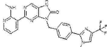
1-311, 9-(4-(1-methyl-4-(trifluoromethyl)-1H-imidazol-2-yl)benzyl)-2-(2-(methylamino)pyridin-3-yl)-7,8-dihydro-8H-purin-6-one
