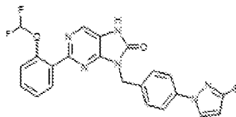
1-89. 2-(2-(difluoromethoxy)phenyl)-9-(4-(3-fluoro-1H-pyrazol-1-yl)benzyl)-7,8-dihydro-8H-purin-6-one
