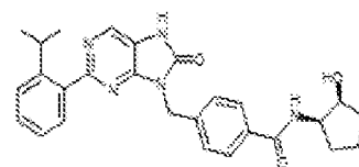
1-387. N-((1R,2S)-2-hydroxycyclopentyl)-4-(2-(2-isopropylphenyl)-5-oxo-7,8-dihydro-8H-purin-8-yl)methylbenzamide
