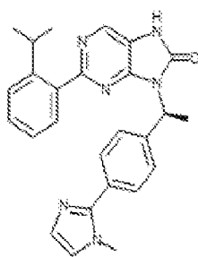
1-310, (S)-2-(2-isopropylphenyl)-9-(1-(4-(1-methyl-1H-imidazol-2-yl)phenyl)ethyl)-7,8-dihydro-8H-purin-6-one
