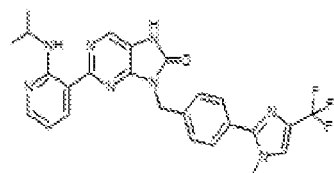
1-313. 2-(2-(isopropylamino)pyridin-3-yl)-9-(4-(1-methyl-4-(trifluoromethyl)-1H-imidazol-2-yl)benzyl)-7,8-dihydro-8H-purin-6-one
