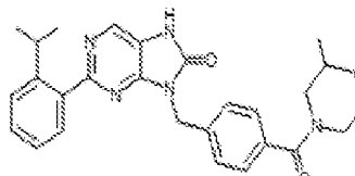
1-399. 2-(2-isopropylphenyl)-8-(4-{3-methylpiperidine-1-carbonyl}benzyl)-7,8-dihydro-8H-purin-6-one
