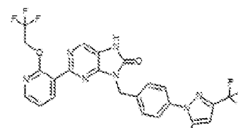
1-42 8-(4-(5-methyl-3-(trifluoromethyl)-1H-pyrazol-1-yl)benzyl)-2-(2,2,2-trifluoroethoxy)pyridin-3-yl)-7,8-dihydro-8H-purin-8-one
