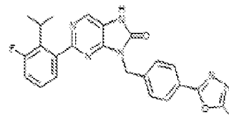
1-189. 2-(3-fluoro-2-isopropylphenyl)-9-(4-(5-methyl-1,3,4-oxadiazol-2-yl)benzyl)-7,8-dihydro-8H-purin-6-one
