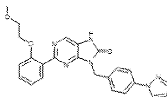
1-20. 9-(4-(1H-pyrazol-1-yl)benzyl)-2-(2-(2-methoxyethoxy)phenyl)-7,8-dihydro-8H-purin-6-one
