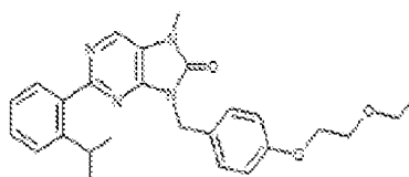
1-236. 9-(4-(2-ethoxyethoxy)benzyl)-2-(2-isopropylphenyl)-7-methyl-7,8-dihydro-8H-purin-6-one
