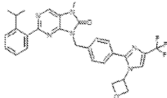
1-110. 2-(2-isopropylphenyl)-7-methyl-9-(4-(1-(oxetan-3-yl)-4-(trifluoromethyl)-1H-imidazol-2-yl)benzyl)-7,8-dihydro-8H-purin-6-one
