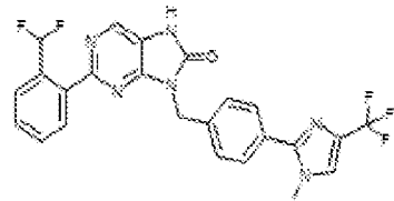
1-31. 2-(2-(difluoromethyl)phenyl)-8-(4-(1-methyl-4-(trifluoromethyl)-1H-imidazol-2-yl)benzyl)-7,9-dihydro-8H-purin-6-one
