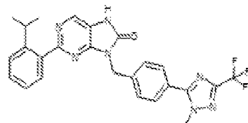
1-289. 2-(2-isopropylphenyl)-9-(4-(1-methyl-3-(trifluoromethyl)-1H-1,2,4-triazol-5-yl)benzyl)-7,8-dihydro-8H-purin-6-one
