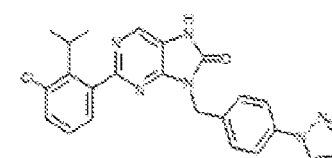
1-93. 9-(4-(1H-pyrazol-1-yl)benzyl)-2-(3-chloro-2-isopropylphenyl)-7,8-dihydro-8H-purin-6-one
