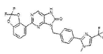
1-36 2-(2,2-difluorobenzos[d][1,3]dioxol-4-yl)-8-(4-(1-methyl-4-(trifluoromethyl)-1H-imidazol-2-yl)benzyl)-7,8-dihydro-8H-purin-8-one
