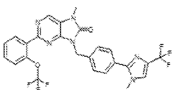
1-49. 7-methyl-9-(4-(1-methyl-4-(trifluoromethyl)-1H-imidazol-2-yl)benzyl)-2-(2-(trifluoromethoxy)phenyl)-7,8-dihydro-8H-purin-8-one
