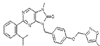
1-235. 2-(2-isopropylphenyl)-7-methyl-9-(4-((5-methylisoxazol-3-yl)methoxy)benzyl)-7,8-dihydro-8H-purin-6-one
