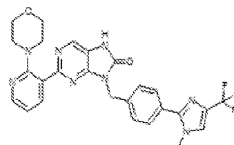
1-333. 9-(4-(1-methyl-4-(trifluoromethyl)-1H-imidazol-2-yl)benzyl)-2-(2-morpholinopyridin-3-yl)-7,9-dihydro-8H-purin-6-one
