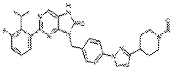
I-464. 5-(4-(3-(1-acetylpiperidin-4-yl)-1H-pyrazol-1-yl)benzyl)-2-(2-fluoro-2-isopropylphenyl)-7,8-dihydro-5H-purin-8-one
