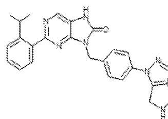
I-102. 8-(4-(5,5-dihydropyrrolo[3,4-c]pyrazol-1(4H)-yl)benzyl)-2-(2-isopropylphenyl)-7,9-dihydro-8H-purin-6-one
