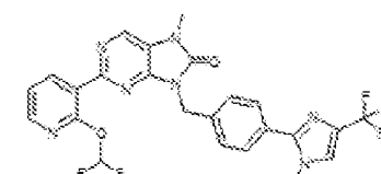
1-48. 2-(2-(difluoromethoxy)pyridin-3-yl)-7-methyl-9-(4-(1-methyl-4-(trifluoromethyl)-1H-imidazol-2-yl)benzyl)-7,8-dihydro-8H-purin-8-one
