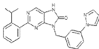
I-197 1-(3-(1H-pyrazol-1-yl)benzyl)-2-(2-isopropylphenyl)-7,8-dihydro-8H-purin-6-one
