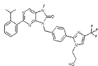
1-106. 9-(4-(1-(2-hydroxyethyl)-4-(trifluoromethyl)-1H-imidazol-2-yl)benzyl)-2-(2-isopropylphenyl)-7-methyl-7,8-dihydro-8H-purin-6-one
