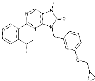
1-239. 9-(3-(3-(cyclopropylmethyl)oxy)benzyl)-2-(2-isopropylphenyl)-7-methyl-7,8-dihydro-8H-purin-6-one
