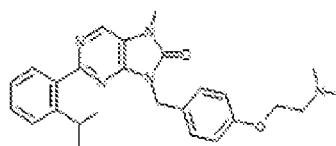
1-233. 9-(4-(2-(dimethylamino)ethoxy)benzyl)-2-(2-isopropylphenyl)-7-methyl-7,8-dihydro-8H-purin-6-one
