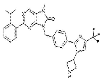
I-436. 9-(4-(1-azetidin-3-yl)-4-(trifluoromethyl)-1H-imidazol-2-yl)benzyl-2-(2-isopropylphenyl)-7-methyl-7,8-dihydro-8H-purin-6-one
