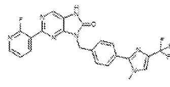
1-57. 2-(2-fluoropyridin-3-yl)-9-(4-(1-methyl-1,4-(trifluoromethyl)-1H-imidazol-2-yl)benzyl)-7,9-dihydro-8H-purin-6-one
