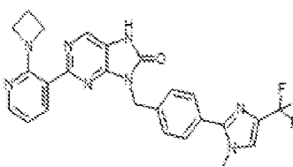
1-335. 2-(2-(azetidin-1-yl)pyridin-3-yl)-8-(4-(1-methyl-4-(trifluoromethyl)-1H-imidazol-2-yl)benzyl)-7,9-dihydro-8H-purin-6-one
