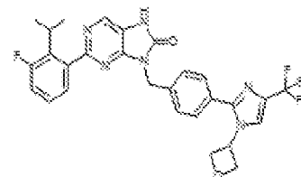
I-201 1-(2-(3-fluoro-2-isopropylphenyl)-9-(4-(1-oxetan-3-yl)-4-(trifluoromethyl)-1H-imidazol-2-yl)benzyl)-7,8-dihydro-8H-purin-6-one
