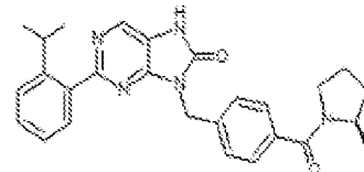
I-369. (R)-2-(2-isopropylphenyl)-8-(4-(2-methylpyrrolidine-1-carbonyl)benzyl)-7,8-dihydro-8H-purin-5-one
