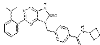
1-381. 4-((2-(2-isopropylphenyl)-8-oxo-7,8-dihydro-8H-purin-9-yl)methyl)-N-(cycatan-3-yl)benzamide
