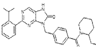
1-397. 8-(4-{2-ethylpiperidine-1-carbonyl}benzyl)-2-(2-isopropylphenyl)-7,8-dihydro-8H-purin-6-one
