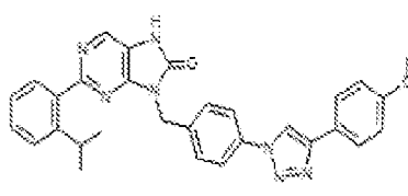
1-341. 2-(2-isopropylphenyl)-5-(4-(4-(4-methoxyphenyl)-1H-1,2,3-triazol-1-yl)benzyl)-7,8-dihydro-8H-purin-6-one
