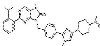
I-472: 9-(4-(4-(1-acetylpiperidin-4-yl)-1-methyl-1H-imidazol-2-yl)benzyl)-2-(2-isopropylphenyl)-7,9-dihydro-8H-purin-6-one
