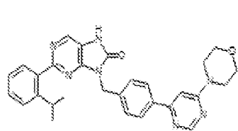
1-250. 2-(2-isopropylphenyl)-9-(4-(8-morpholinopyrimidin-4-yl)benzyl)-7,8-dihydro-8H-purin-6-one
