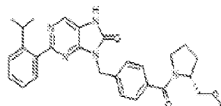
I-403. (R)-2-(2-isopropylphenyl)-6-(4-(2-methoxymethyl)pyrrolidin-1-yl)benzyl-7,8-dihydro-8H-purin-6-one
