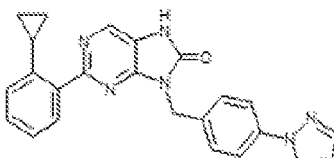
1-94. 9-(4-(1H-pyrazol-1-yl)benzyl)-2-(2-cyclopropylphenyl)-7,8-dihydro-8H-purin-6-one
