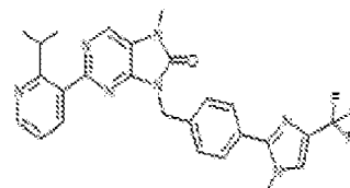
I-105. 2-(2-isopropylpyridin-3-yl)-7-methyl-8-(4-(1-methyl-4-(trifluoromethyl)-1H-imidazol-2-yl)benzyl)-7,9-dihydro-8H-purin-6-one
