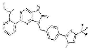
1-331. 2-(2-(ethyl(methylamino)pyridin-3-yl)-8-(4-(1-methyl-4-(trifluoromethyl)-1H-imidazol-2-yl)benzyl)-7,9-dihydro-8H-purin-6-one
