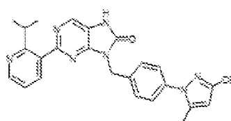
1-52. 9-(4-(3-chloro-5-methyl-1H-pyrazol-1-yl)benzyl)-2-(2-isopropylpyridin-3-yl)-7,9-dihydro-8H-purin-6-one
