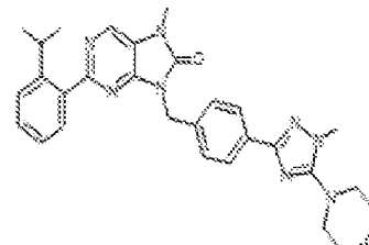
1-282. 2-(2-isopropylphenyl)-7-methyl-5-(4-(1-methyl-5-morpholino-1H-1,2,4-triazol-3-yl)benzyl)-7,8-dihydro-8H-purin-6-one
