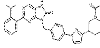
I-468: 9-(4-(3-(1-acetylpiperidin-3-yl)-1H-pyrazol-1-yl)benzyl)-2-(2-isopropylphenyl)-7,9-dihydro-8H-purin-6-one
