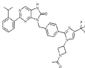
1-476. 9-(4-(1-(1-acetylzetidin-3-yl)-4-(trifluoroethyl)-1H-imidazol-2-yl)benzyl)-2-(2-isopropylphenyl)-7,8-dihydro-8H-purin-6-one
