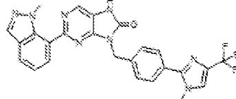
1-44. 2-(1-methyl-1H-indazol-7-yl)-9-(4-(1-methyl-4-(trifluoromethyl)-1H-imidazol-2-yl)benzyl)-7,8-dihydro-8H-purin-8-one
