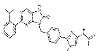
1-538. N-(2-(4-(2-(2-isopropylphenyl)-8-oxo-7,8-dihydro-5H-purin-3-yl)methyl)phenyl)-1-methyl-1H-imidazo[4,5-b]pyridine-4-carboxamide
