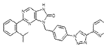
I-348. 2-(2-isopropylphenyl)-3-(4-(4-pyridin-2-yl)-1H-1,2,3-triazol-1-yl)benzyl-7,8-dihydro-5H-purin-8-one
