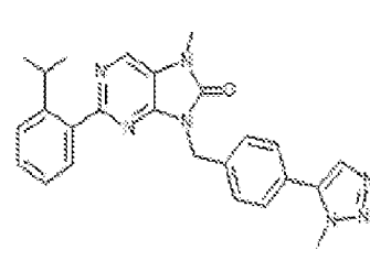
1-285. 2-(2-isopropylphenyl)-7-methyl-5-(4-(1-methyl-1H-1,2,3-triazol-5-yl)benzyl)-7,8-dihydro-8H-purin-6-one
