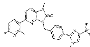
1-66. 2-(5-fluoro-2-methylpyridin-3-yl)-7-methyl-9-(4-(1-methyl-4-(trifluoromethyl)-1H-imidazol-2-yl)benzyl)-7,9-dihydro-8H-purin-8-one
