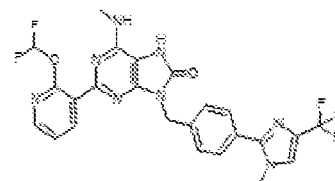
1-531. 2-(2-(difluoromethoxy)pyridin-3-yl)-9-(4-(1-methyl-4-(trifluoromethyl)-1H-imidazol-2-yl)benzyl)-6-(methylamino)-7,5-dihydro-8H-purin-8-one
