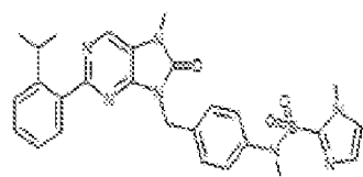
I-457. N-(4-((2-(2-isopropylphenyl)-7-methyl-8-oxo-7,8-dihydro-5H-purin-9-yl)methyl)phenyl)-N,1,6-dimethyl-1H-imidazole-2-sulfonamide
