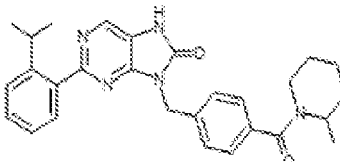
1-398. 2-(2-isopropylphenyl)-8-(4-{2-methylpiperidine-1-carbonyl}benzyl)-7,8-dihydro-8H-purin-6-one
