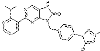
1-53. 9-(4-(5-chloro-3-methyl-1H-pyrazol-1-yl)benzyl)-2-(2-isopropylpyridin-3-yl)-7,9-dihydro-8H-purin-6-one
