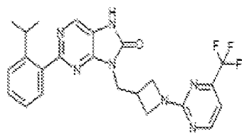
I-502, 2-(2-isopropylphenyl)-9-((1-(4-(trifluoromethyl)pyrimidin-2-yl)azetidin-3-yl)methyl)-7,8-dihydro-5H-purin-8-one
