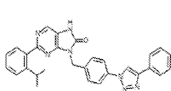
1-343. 2-(2-isopropylphenyl)-5-(4-(4-phenyl-1H-1,2,3-triazol-1-yl)benzyl)-7,8-dihydro-8H-purin-6-one
