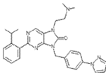
1-107. 9-(4-(1H-pyrazol-1-yl)benzyl)-7-(2-(dimethylamino)ethyl)-2-(2-isopropylphenyl)-7,8-dihydro-8H-purin-6-one
