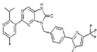
1-67. 2-(5-fluoro-2-isopropylpyridin-3-yl)-9-(4-(1-methyl-4-(trifluoromethyl)-1H-imidazol-2-yl)benzyl)-7,9-dihydro-8H-purin-8-one
