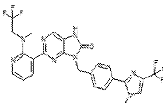
1-332. 2-(2-(methyl(2,2,2-trifluoroethyl)amino)pyridin-3-yl)-8-(4-(1-methyl-4-(trifluoromethyl)-1H-imidazol-2-yl)benzyl)-7,9-dihydro-8H-purin-6-one
