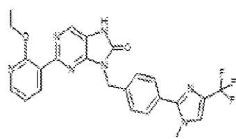
I-421. 2-(2-ethoxypyridin-3-yl)-9-(4-(1-methyl-4-(trifluoromethyl)-1H-imidazol-2-yl)benzyl)-7,8-dihydro-8H-purin-6-one
