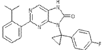
I-227. 9-(1-(4-fluorophenyl)cyclopropyl)-2-(2-isopropylphenyl)-7,8-dihydro-8H-purin-6-one
