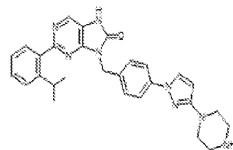
I-432. 2-(2-isopropylphenyl)-9-(4-(3-piperazin-1-yl)-1H-pyrazol-1-yl)benzyl-7,8-dihydro-8H-purin-6-one
