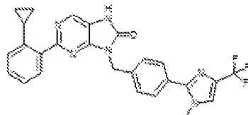
I-98. 2-(2-cyclopropylphenyl)-5-(4-(1-methyl-4-(trifluoromethyl)-1H-imidazol-2-yl)benzyl)-7,9-dihydro-8H-purin-6-one
