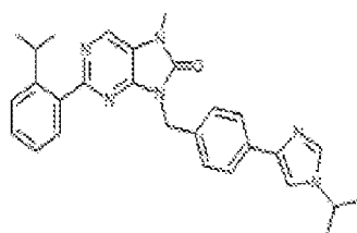
1-277. 5-(4-(1-isopropyl-1H-imidazol-4-yl)benzyl)-2-(2-isopropylphenyl)-7-methyl-7,8-dihydro-8H-purin-6-one
