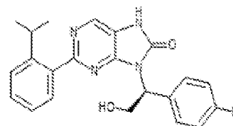
1-180. (S)-3-(1-(4-fluorophenyl)-2-hydroxyethyl)-2-(2-isopropylphenyl)-7,8-dihydro-8H-purin-6-one
