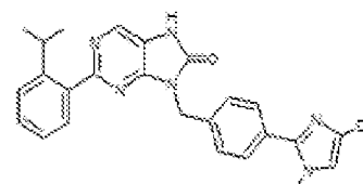
I-198 1-(4-(4-chloro-1-methyl-1H-imidazol-2-yl)benzyl)-2-(2-isopropylphenyl)-7,8-dihydro-8H-purin-6-one
