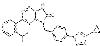
1-343. 5-(4-(4-cyclopropyl-1H-1,2,3-triazol-1-yl)benzyl)-2-(2-isopropylphenyl)-7,8-dihydro-8H-purin-6-one
