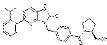
1-382. (S)-5-(4-(2-(hydroxymethyl)pyrrolidine-1-carbonyl)benzyl)-2-(2-isopropylphenyl)-7,8-dihydro-8H-purin-6-one
