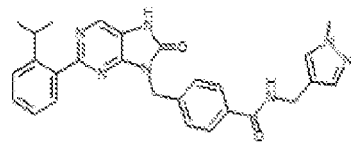
I-361. 4-((2-(2-isopropylphenyl)-8-oxo-7,8-dihydro-5H-purin-9-yl)methyl)-N-((1-methyl-1H-pyrazol-4-yl)methyl)benzamide
