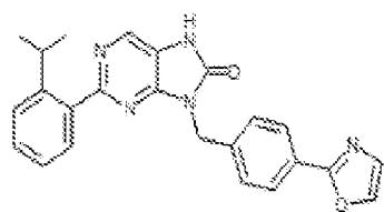
I-169. 2-(2-isopropylphenyl)-9-(4-(oxazol-2-yl)benzyl)-7,8-dihydro-8H-purin-6-one
