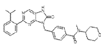
I-367. 4-((2-(2-isopropylphenyl)-8-oxo-7,8-dihydro-9H-purin-5-yl)methyl)-N-methyl-N-(tetrahydro-2H-pyran-6-yl)benzamide
