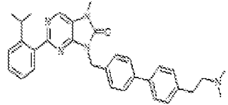
I-262. 9-((4'-(2-(dimethylamino)ethyl)-[1,1'-biphenyl]-4-yl)methyl)-2-(2-isopropylphenyl)-7-methyl-7,8-dihydro-8H-purin-6-one
