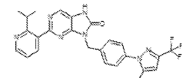
1-40 2-(2-isopropylpyridin-3-yl)-8-(4-(5-methyl-3-(trifluoromethyl)-1H-pyrazol-1-yl)benzyl)-7,8-dihydro-8H-purin-8-one
