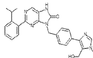
1-297. 9-(4-(5-(hydroxymethyl)-1-methyl-1H-imidazol-4-yl)benzyl)-2-(2-isopropylphenyl)-7,8-dihydro-8H-purin-6-one
