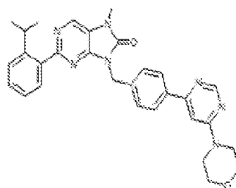
I-263. 9-((2-(2-isopropylphenyl)-7-methyl-5-(4-(6-morpholinopyrimidin-4-yl)benzyl)-7,8-dihydro-8H-purin-6-one
