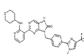
1-321. 9-(4-(1-methyl-4-(trifluoromethyl)-1H-imidazol-2-yl)benzyl)-2-(2-(2-(tetrahydro-2H-pyran-4-ylamino)pyridin-3-yl)-7,8-dihydro-8H-purin-6-one
