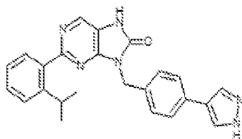
1-539. 8-(4-(1H-pyrazol-4-yl)benzyl)-2-(2-isopropylphenyl)-7,8-dihydro-5H-purin-2-one
