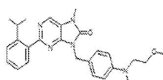
1-491. 2-(2-isopropylphenyl)-6-(4-(2-methoxyethyl(methylamino)benzyl)-7-methyl-7,8-dihydro-6H-purin-6-one
