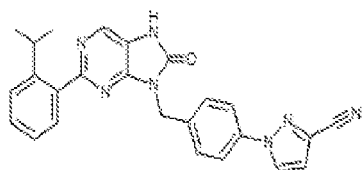
I-196 1-(4-(2-(2-isopropylphenyl)-8-oxo-7,8-dihydro-2H-purin-6-yl)methylphenyl)-1H-pyrazole-3-carbonitrile
