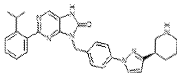
I-224. (R)-2-(2-isopropylphenyl)-9-(4-(3-(piperidin-3-yl)-1H-pyrazol-1-yl)benzyl)-7,8-dihydro-8H-purin-6-one
