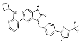
1-316. 2-(2-(cyclobutylamino)pyridin-3-yl)-9-(4-(1-methyl-4-(trifluoromethyl)-1H-imidazol-2-yl)benzyl)-7,8-dihydro-8H-purin-6-one
