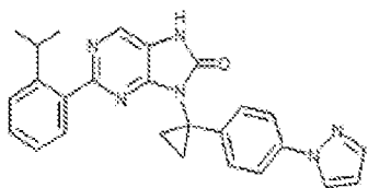
I-226. 9-(1-(4-(1H-pyrazol-1-yl)phenyl)cyclopropyl)-2-(2-isopropylphenyl)-7,8-dihydro-8H-purin-6-one
