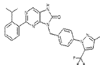
1-195. 2-(2-isopropylphenyl)-9-(4-(5-methyl-5-(trifluoromethyl)-1H-pyrazol-1-yl)benzyl)-7,8-dihydro-8H-purin-6-one
