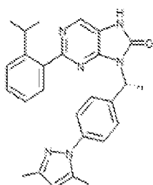
1-190. (R)-9-(1-(4-(3,5-dimethyl-1H-pyrazol-1-yl)phenylethyl)-2-(2-isopropylphenyl)-7,8-dihydro-8H-purin-6-one
