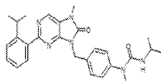
1-484. 3-isopropyl-1-(4-(2-(2-isopropylphenyl)-7-methyl-8-oxo-7,8-dihydro-6H-purin-5-yl)methylphenyl)-1-methylurea
