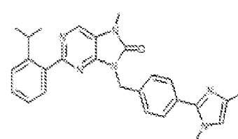
1-258. 9-(4-(1,4-dimethyl-1H-imidazol-2-yl)benzyl)-2-(2-isopropylphenyl)-7-methyl-7,8-dihydro-8H-purin-6-one
