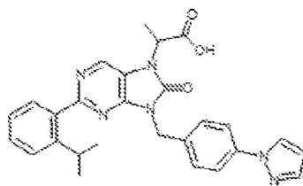
1-530. 2-(3-(4-(1H-pyrazol-1-yl)benzyl)-2-(2-isopropylphenyl)-8-oxo-8,5-dihydro-7H-purin-1-yl)propanoic acid
