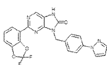
1-25. 8-(4-(1H-pyrazol-1-yl)benzyl)-2-(2,2-difluorobenzofuran-5-yl)-7,9-dihydro-8H-purin-6-one
