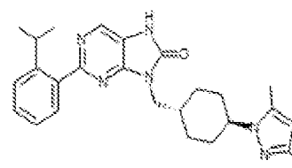
1-213. 9-((((1s,4s)-4-(3,5-dimethyl-1H-pyrazol-1-yl)pyrrolhexyl)methyl)-2-(2-isopropylphenyl)-7,8-dihydro-8H-purin-6-one
