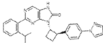
1-164. 8-((1S,2R)-2-(4-(1H-pyrazol-1-yl)phenyl)cyclobutyl)-2-(2-isopropylphenyl)-7,8-dihydro-8H-purin-6-one
