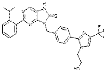
I-506, 3-((4-((1-(2-hydroxyethyl)-4-(trifluoromethyl)-1H-midazol-2-yl)benzyl)-2-(2-isopropylphenyl)-7,8-dihydro-5H-purin-8-one
