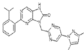
1-511. 8-((5-(3,5-dimethyl-1H-pyrazol-1-yl)pyrimidin-2-yl)methyl)-2-(2-isopropylphenyl)-7,9-dihydro-8H-purin-6-one
