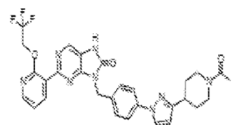
I-466: 9-(4-(2-(1-acetylpiperidin-4-yl)-1H-pyrazol-1-yl)benzyl)-2-(2-(2,2,2-trifluoroethoxy)pyridin-3-yl)-7,9-dihydro-8H-purin-6-one
