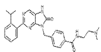
I-408. N-(2-(dimethylamino)ethyl)-4-((2-(2-isopropylphenyl)-5-oxo-7,8-dihydro-6H-purin-9-yl)methyl)benzamide
