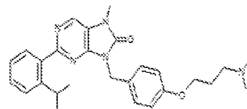
1-234. 9-(4-(3-(dimethylamino)propoxy)benzyl)-2-(2-isopropylphenyl)-7-methyl-7,8-dihydro-8H-purin-6-one
