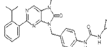
1-483. 1-isopropyl-3-(4-(2-(2-isopropylphenyl)-7-methyl-8-oxo-7,8-dihydro-6H-purin-9-yl)methyl)phenyl)urea
