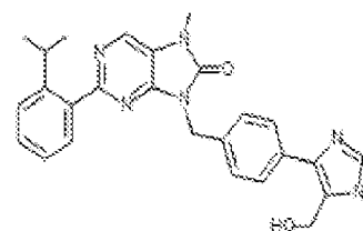
1-288. 9-(4-(5-hydroxymethyl)-1-methyl-1H-imidazol-4-yl)benzyl)-2-(2-isopropylphenyl)-7-methyl-7,8-dihydro-8H-purin-6-one
