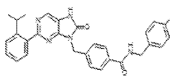
I-354. N-(4-fluorobenzyl)-4-(2-(2-isopropylphenyl)-8-oxo-7,8-dihydro-5H-purin-9-yl)methylbenzamide
