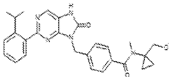
1-391. 4-((2-(2-isopropylphenyl)-5-oxo-7,8-dihydro-8H-purin-8-yl)methyl)-N-((1-methoxymethyl)piperidin-4-yl)methylbenzamide
