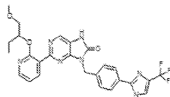
I-428. 2-(2-(1-methoxybutan-2-yl)oxy)pyridin-3-yl)-9-(4-(1-methyl-4-(trifluoromethyl)-1H-imidazol-2-yl)benzyl)-7,8-dihydro-8H-purin-6-one
