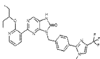
I-427. 9-(4-(1-methyl-4-(trifluoromethyl)-1H-imidazol-2-yl)benzyl)-2-(2-(pentan-3-yloxy)pyridin-3-yl)-7,8-dihydro-8H-purin-6-one
