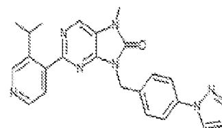
1-516. 8-((4-(1H-pyrazol-1-yl)benzyl)-2-(2-isopropylphenyl)-4-yl)-7-methyl-7,9-dihydro-8H-purin-6-one
