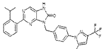
1-194. 2-(2-isopropylphenyl)-9-(4-(5-methyl-3-(trifluoromethyl)-1H-pyrazol-1-yl)benzyl)-7,8-dihydro-8H-purin-6-one
