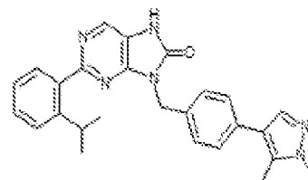
1-252. 9-(4-(1,5-dimethyl-1H-pyrazol-4-yl)benzyl)-2-(2-isopropylphenyl)-7,8-dihydro-8H-purin-6-one
