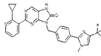
1-30. 2-(2-cyclopropylpyridin-3-yl)-8-(4-(1-methyl-4-(trifluoromethyl)-1H-imidazol-2-yl)benzyl)-7,9-dihydro-8H-purin-6-one
