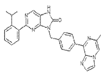
1-306, 2-(2-isopropylphenyl)-9-(4-(5-methylimidazol-2-yl)pyrazin-3-yl)benzyl)-7,8-dihydro-8H-purin-6-one
