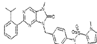
I-454, N-(4-(2-(2-isopropylphenyl)-7-methyl-8-oxo-7,8-dihydro-8H-purin-9-yl)methyl)phenyl)-1-methyl-1H-imidazole-2-sulfonamide
