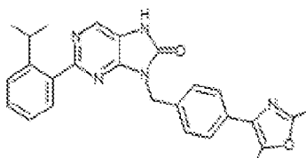
I-200 1-(3-(4-(2,5-dimethyloxazol-4-yl)benzyl)-2-(2-isopropylphenyl)-7,8-dihydro-8H-purin-6-one
