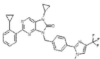
I-100. 7-cyclopropyl-2-(2-cyclopropylphenyl)-8-(4-(1-methyl-4-(trifluoromethyl)-1H-imidazol-2-yl)benzyl)-7,9-dihydro-8H-purin-6-one
