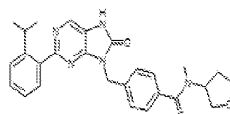
1-402. 4-(2-(2-isopropylphenyl)-8-oxo-7,8-dihydro-8H-purin-3-yl(methyl)-N-methyl-N-(tetrahydrofuran-3-yl)benzamide
