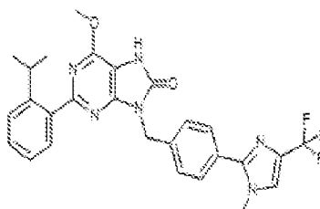
1-535. 2-(2-isopropylphenyl)-6-methoxy-9-(4-(1-methyl-4-(trifluoromethyl)-1H-imidazol-2-yl)benzyl)-7,5-dihydro-8H-purin-8-one
