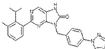
1-91. 9-(4-(1H-pyrazol-1-yl)benzyl)-2-(2-isopropyl-3-methylphenyl)-7,8-dihydro-8H-purin-6-one
