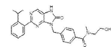
1-376. N-(2-hydroxyethyl)-4-((2-(2-isopropylphenyl)-8-oxo-7,8-dihydro-5H-purin-9-yl)methyl)-N-methylbenzamide
