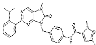
I-469: N-(4-(2-(2-isopropylphenyl)-7-methyl-8-oxo-7,9-dihydro-8H-purin-8-yl)methyl)phenyl)-1,3-dimethyl-1H-pyrazole-5-carboxamide
