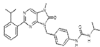
1-481. 1-isopropyl-3-(4-(2-(2-isopropylphenyl)-7-methyl-8-oxo-7,8-dihydro-6H-purin-9-yl)methyl)phenyl)urea
