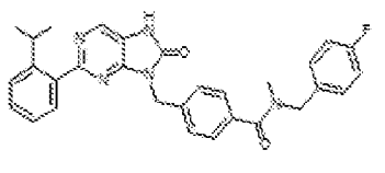
I-365. N-(4-fluorobenzyl)-4-((2-(2-isopropylphenyl)-8-oxo-7,8-dihydro-5H-purin-9-yl)methyl)-N-methylbenzamide
