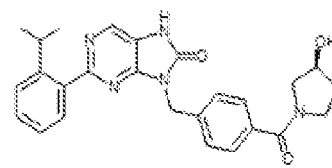
1-378. (S)-5-(4-(3-hydroxypyrrolidine-1-carbonyl)benzyl)-2-(2-isopropylphenyl)-7,8-dihydro-8H-purin-6-one
