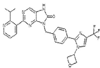
1-32. 2-(2-isopropylpyridin-3-yl)-8-(4-(1-(oxetan-3-yl)-4-(trifluoromethyl)-1H-imidazol-2-yl)benzyl)-7,9-dihydro-8H-purin-6-one
