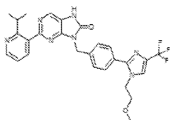
1-43. 2-(2-isopropylpyridin-3-yl)-9-(4-(1-(2-methoxyethyl)-4-(trifluoromethyl)-1H-imidazol-2-yl)benzyl)-7,8-dihydro-8H-purin-8-one
