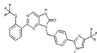
1-37 9-(4-(1-methyl-4-(trifluoromethyl)-1H-imidazol-2-yl)benzyl)-2-(2-(trifluoromethoxy)phenyl)-7,8-dihydro-8H-purin-8-one
