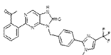
1-38 2-(2-acetylphenyl)-8-(4-(1-methyl-4-(trifluoromethyl)-1H-imidazol-2-yl)benzyl)-7,8-dihydro-8H-purin-8-one
