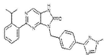
1-274. 2-(2-isopropylphenyl)-9-(4-(1-methyl-1H-1,2,4-triazol-3-yl)benzyl)-7,8-dihydro-8H-purin-6-one
