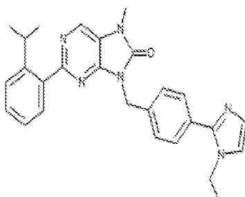
1-496. 9-(4-(1-ethyl-1H-imidazol-2-yl)benzyl)-2-(2-isopropylphenyl)-7-methyl-7,8-dihydro-8H-purin-6-one
