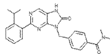
I-355. 4-(2-(2-isopropylphenyl)-8-oxo-7,8-dihydro-5H-purin-9-yl)methyl-N,N-dimethylbenzamide
