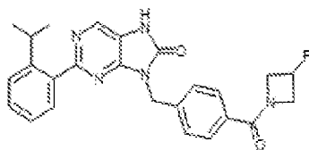
1-386. 3-(4-(3-fluoroazetidine-1-carbonyl)benzyl)-2-(2-isopropylphenyl)-7,8-dihydro-8H-purin-6-one
