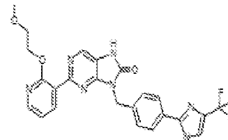
I-423. 2-(2-(2-methoxyethoxy)pyridin-3-yl)-9-(4-(1-methyl-4-(trifluoromethyl)-1H-imidazol-2-yl)benzyl)-7,8-dihydro-8H-purin-6-one
