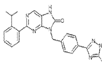
1-294. 9-(4-(1,5-dimethyl-1H-1,2,4-triazol-3-yl)benzyl)-2-(2-isopropylphenyl)-7,8-dihydro-8H-purin-6-one
