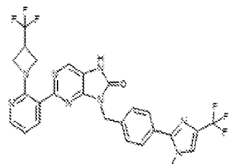
1-337. 9-(4-(1-methyl-4-(trifluoromethyl)-1H-imidazol-2-yl)benzyl)-2-(2-(3-(trifluoromethyl)azetidin-1-yl)pyridin-3-yl)-7,9-dihydro-8H-purin-6-one
