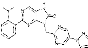
I-509, 9-((5-(1H-pyrazol-1-yl)pyrimidin-2-yl)methyl)-2-(2-isopropylphenyl)-7,8-dihydro-5H-purin-8-one
