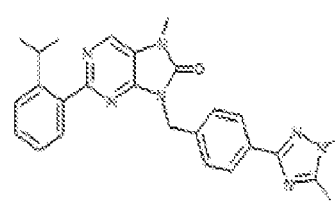
1-279. 5-(4-(1,5-dimethyl-1H-1,2,4-triazol-3-yl)benzyl)-2-(2-isopropylphenyl)-7-methyl-7,8-dihydro-8H-purin-6-one
