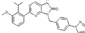
1-92. 9-(4-(1H-pyrazol-1-yl)benzyl)-2-(2-isopropyl-3-methoxyphenyl)-7,8-dihydro-8H-purin-6-one
