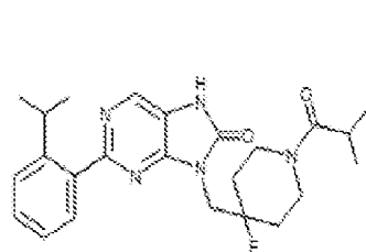
1-475. 5-(4-fluoro-1-isobutylpiperidin-4-yl)methyl-2-(2-isopropylphenyl)-7,8-dihydro-8H-purin-6-one
