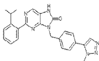
1-298. 9-(4-(2-isopropylphenyl)-5-(4-(1-methyl-1H-1,2,3-triazol-5-yl)benzyl)-7,8-dihydro-8H-purin-6-one
