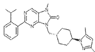
1-112. 5-(((1r,4r)-4-(3,5-dimethyl-1H-pyrazol-1-yl)cyclohexyl)methyl)-2-(2-isopropylphenyl)-7-methyl-7,8-dihydro-8H-purin-6-one
