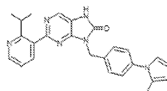
1-54. 2-(2-isopropylpyridin-3-yl)-9-(4-(2-methyl-1H-pyrazol-1-yl)benzyl)-7,9-dihydro-8H-purin-6-one
