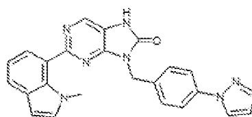
1-29. 8-(4-(1H-pyrazol-1-yl)benzyl)-2-(4-(1-methyl-1H-indazol-7-yl)-7,9-dihydro-8H-purin-6-one
