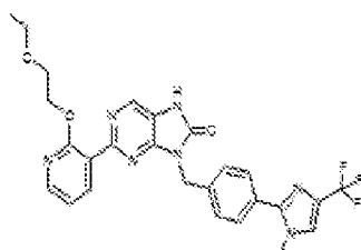
I-415, 2-(2-(2-ethoxyethoxy)pyridin-3-yl)-5-(4-(1-methyl-4-(trifluoromethyl)-1H-imidazol-2-yl)benzyl)-7,8-dihydro-2H-purin-6-one
