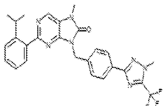
1-280. 2-(2-isopropylphenyl)-7-methyl-5-(4-(1-methyl-5-(trifluoromethyl)-1H-1,2,4-triazol-3-yl)benzyl)-7,8-dihydro-8H-purin-6-one
