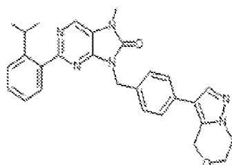
I-255. 9-((4-(5,7-dihydro-4H-pyrazolo[5,1-c][1,4]oxazin-3-yl)benzyl)-2-(2-isopropylphenyl)-7-methyl-7,8-dihydro-8H-purin-6-one
