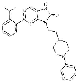
1-161. 2-(2-isopropylphenyl)-8-(2-(1-(pyridin-3-yl)pyrrolidin-4-yl)ethyl)-7,8-dihydro-8H-purin-6-one
