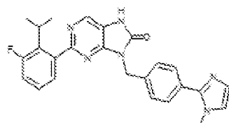
I-172. 2-(3-fluoro-2-isopropylphenyl)-9-(4-(1-methyl-1H-imidazol-2-yl)benzyl)-7,8-dihydro-8H-purin-6-one
