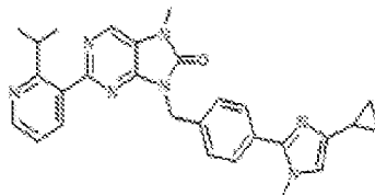
1-515. 8-((4-(4-cyclopropyl-1-methyl-1H-imidazol-2-yl)benzyl)-2-(2-isopropylphenyl)-7-methyl-7,9-dihydro-8H-purin-6-one
