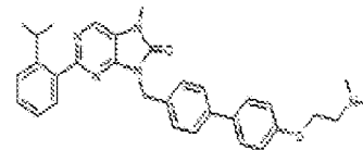
I-261. 9-((4'-(2-(dimethylamino)ethoxy)-[1,1'-biphenyl]-4-yl)methyl)-2-(2-isopropylphenyl)-7-methyl-7,8-dihydro-8H-purin-6-one
