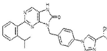
1-347. (R)-5-(4-(4-(1-hydroxyethyl)-1H-1,2,3-triazol-1-yl)benzyl)-2-(2-isopropylphenyl)-7,8-dihydro-8H-purin-6-one
