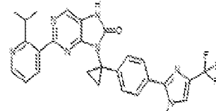
1-51. 2-(2-isopropylpyridin-3-yl)-9-(4-(1-methyl-4-(trifluoromethyl)-1H-imidazol-2-yl)phenyl)cyclopropyl)-7,8-dihydro-8H-purin-8-one
