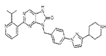
I-435. 2-(2-isopropylpyridin-5-yl)-9-(4-(3-piperidin-4-yl)-1H-pyrazol-1-yl)benzyl-7,8-dihydro-8H-purin-6-one
