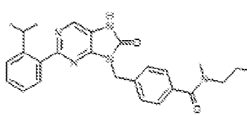
I-374. 4-((2-(2-isopropylphenyl)-8-oxo-7,8-dihydro-9H-purin-5-yl)methyl)-N-methyl-N-propylbenzamide
