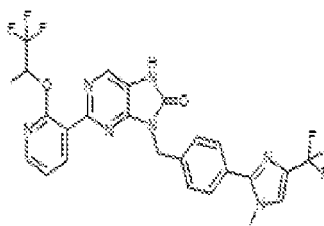
I-418, 5-(4-(1-methyl-4-(trifluoromethyl)-1H-imidazol-2-yl)benzyl)-2-(2-(1,1,1-trifluoropropan-2-yl)oxypyridin-3-yl)-7,8-dihydro-2H-purin-6-one
