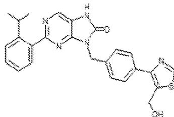
1-302. 9-(4-(5-(hydroxymethyl)thiazol-4-yl)benzyl)-2-(2-isopropylphenyl)-7,8-dihydro-8H-purin-6-one
