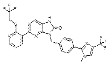
1-26. 8-(4-(1-methyl-4-(trifluoromethyl)-1H-imidazol-2-yl)benzyl)-2-(2,2,2-trifluoroethoxy)pyridin-3-yl)-7,9-dihydro-8H-purin-6-one
