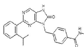
I-361. 4-(2-(2-isopropylphenyl)-8-oxo-7,8-dihydro-5H-purin-9-yl)methyl-N-methylbenzamide
