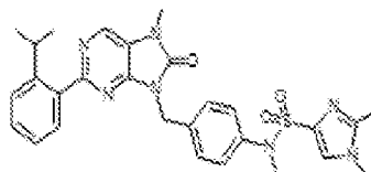
I-458. N-(4-((2-(2-isopropylphenyl)-7-methyl-8-oxo-7,8-dihydro-5H-purin-9-yl)methyl)phenyl)-N,1,2-trimethyl-1H-imidazole-4-sulfonamide
