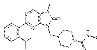
1-479. N-cyclopropyl-4-(2-(2-isopropylphenyl)-7-methyl-8-oxo-7,8-dihydro-6H-purin-9-yl)methylpiperidine-1-carboxamide
