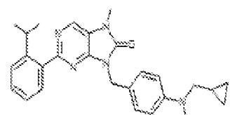
1-490. 3-(4-(cyclopropylmethyl(methylamino)benzyl)-2-(2-isopropylphenyl)-7-methyl-7,8-dihydro-6H-purin-6-one
