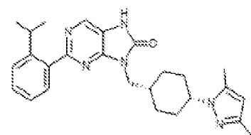
1-212. 9-((((1s,4s)-4-(3,5-dimethyl-1H-pyrazol-1-yl)pyrrolhexyl)methyl)-2-(2-isopropylphenyl)-7,8-dihydro-8H-purin-6-one
