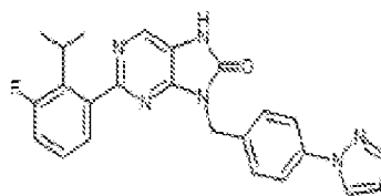
I-170. 9-(4-(1H-pyrazol-1-yl)benzyl)-2-(3-fluoro-2-isopropylphenyl)-7,8-dihydro-8H-purin-6-one
