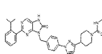
1-480. 4-(1-(4-(2-(2-isopropylphenyl)-8-oxo-7,8-dihydro-6H-purin-9-yl)methyl)phenyl)-1H-pyrazol-3-yl)-N-methylpiperidine-1-carboxamide
