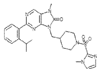
I-451, 2-(2-isopropylphenyl)-7-methyl-8-((1-(1-methyl-1H-imidazol-2-yl)sulfonyl)piperidin-4-yl)methyl)-7,8-dihydro-8H-purin-6-one
