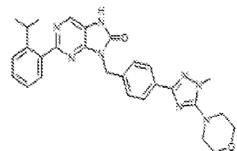
1-292. 2-(2-isopropylphenyl)-5-(4-(1-methyl-5-morpholin-1-yl-1H-1,2,4-triazol-3-yl)benzyl)-7,8-dihydro-8H-purin-6-one
