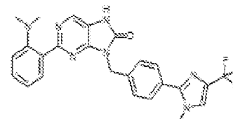
1-90. 2-(2-(dimethylamino)phenyl)-9-(4-(1-methyl-4-trifluoromethyl-1H-imidazol-2-yl)benzyl)-7,8-dihydro-8H-purin-6-one
