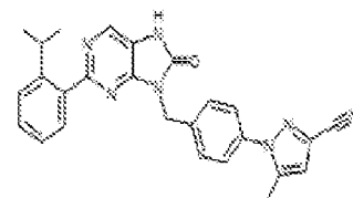
1-297. 1,4-bis(2-isopropylphenyl)-5-oxo-7,8-dihydro-8H-purin-9-ylmethyl(phenyl)-5-methyl-1H-pyrazole-3-carbonitrile
