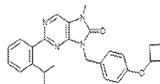
1-237. 9-(4-(cyclobutoxy)benzyl)-2-(2-isopropylphenyl)-7-methyl-7,8-dihydro-8H-purin-6-one
