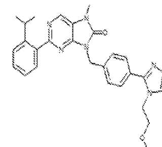
1-498. 2-(2-isopropylphenyl)-9-(4-(1-(2-methoxyethyl)-1H-imidazol-2-yl)benzyl)-7-methyl-7,8-dihydro-8H-purin-6-one
