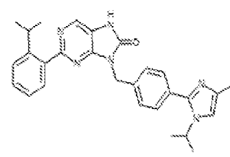
1-537. 9-(4-(1-isopropyl-4-methyl-1H-imidazol-2-yl)benzyl)-2-(2-isopropylphenyl)-7,5-dihydro-8H-purin-8-one
