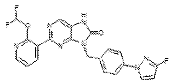
1-88. 2-(2-(difluoromethoxy)pyridin-5-yl)-9-(4-(3-fluoro-1H-pyrazol-1-yl)benzyl)-7,8-dihydro-8H-purin-6-one
