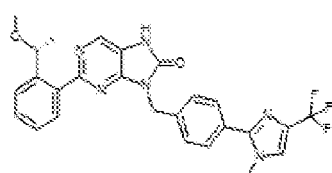
1-55. (R)-2-(2-(1-methoxyethyl)phenyl)-9-(4-(1-methyl-1,4-(trifluoromethyl)-1H-imidazol-2-yl)benzyl)-7,9-dihydro-8H-purin-6-one
