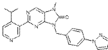
1-17. 9-(4-(1H-pyrazol-1-yl)benzyl)-2-(4-isopropylpyridin-3-yl)-7-methyl-7,8-dihydro-8H-purin-6-one
