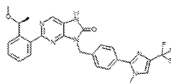
1-56. (S)-2-(2-(1-methoxyethyl)phenyl)-9-(4-(1-methyl-1,4-(trifluoromethyl)-1H-imidazol-2-yl)benzyl)-7,9-dihydro-8H-purin-6-one
