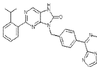
1-291. 9-(4-(imidazo[1,2-a]pyrazin-3-yl)benzyl)-2-(2-isopropylphenyl)-7,8-dihydro-8H-purin-6-one
