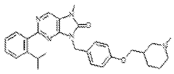
I-230. 2-(2-isopropylphenyl)-7-methyl-9-(4-(3-methylpiperidin-3-yl)methoxy)benzyl-7,8-dihydro-8H-purin-6-one
