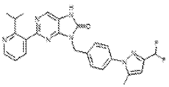
1-58. 9-(4-(2-(difluoromethyl)-5-methyl-1H-pyrazol-1-yl)benzyl)-2-(2-isopropylpyridin-3-yl)-7,9-dihydro-8H-purin-6-one
