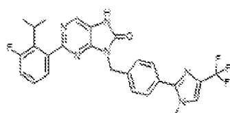
1-193. 2-(3-fluoro-2-isopropylphenyl)-9-(4-(5-methyl-4-(trifluoromethyl)-1H-imidazol-2-yl)benzyl)-7,8-dihydro-8H-purin-6-one
