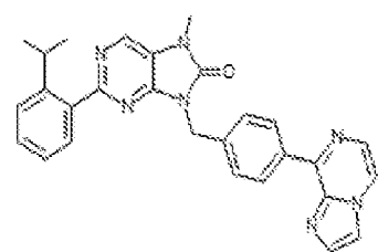
1-289. 5-(4-(imidazo[1,2-a]pyrazin-3-yl)benzyl)-2-(2-isopropylphenyl)-7-methyl-7,8-dihydro-8H-purin-6-one
