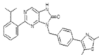
1-301. 9-(4-(2,5-dimethylthiazol-4-yl)benzyl)-2-(2-isopropylphenyl)-7,8-dihydro-8H-purin-6-one
