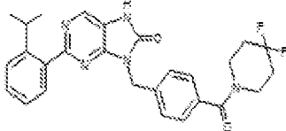
1-388. 3-(4-(4,4-difluoropiperidine-1-carbonyl)benzyl)-2-(2-isopropylphenyl)-7,8-dihydro-8H-purin-6-one
