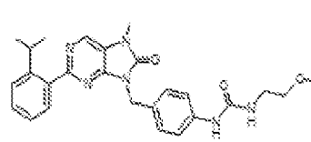
1-482. 1-(4-(2-(2-isopropylphenyl)-7-methyl-8-oxo-7,8-dihydro-6H-purin-9-yl)methyl)phenyl)-3-(2-methoxyethyl)urea
