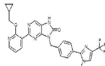
I-414, 2-(2-(cyclopropylmethoxy)pyridin-3-yl)-5-(4-(1-methyl-4-(trifluoromethyl)-1H-imidazol-2-yl)benzyl)-7,8-dihydro-2H-purin-6-one
