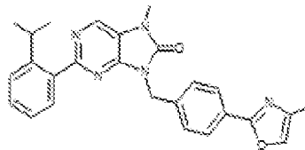
1-290. 2-(2-isopropylphenyl)-7-methyl-5-(4-(4-methyl-oxazol-2-yl)benzyl)-7,8-dihydro-8H-purin-6-one
