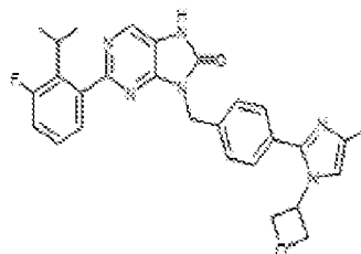
I-202 1-(2-(3-fluoro-2-isopropylphenyl)-9-(4-(4-methyl-1-oxetan-3-yl)-1H-imidazol-2-yl)benzyl)-7,8-dihydro-8H-purin-6-one
