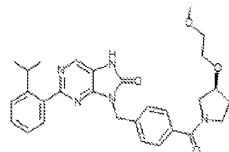
1-384. (S)-2-(2-isopropylphenyl)-5-(4-(3-(2-methoxyethoxy)pyrrolidine-1-carbonyl)benzyl)-7,8-dihydro-8H-purin-6-one
