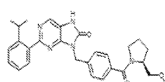
1-396. (5)-2-(2-isopropylphenyl)-8-(4-{2-methoxymethylpyrrolidine-1-carbonyl}benzyl)-7,8-dihydro-8H-purin-6-one
