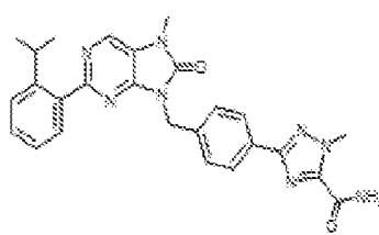
1-278. 3-(4-(2-(2-isopropylphenyl)-7-methyl-8-oxo-7,8-dihydro-8H-purin-9-yl)methyl)phenyl)-1-methyl-1H-1,2,4-triazole-5-carboxamide
