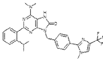
1-533. 6-(dimethylamino)-2-(2-isopropylphenyl)-9-(4-(1-methyl-4-(trifluoromethyl)-1H-imidazol-2-yl)benzyl)-7,5-dihydro-8H-purin-8-one
