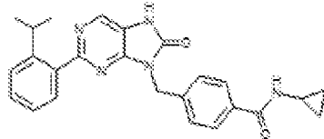
I-353. N-cyclopropyl-4-(2-(2-isopropylphenyl)-8-oxo-7,8-dihydro-5H-purin-9-yl)methylbenzamide
