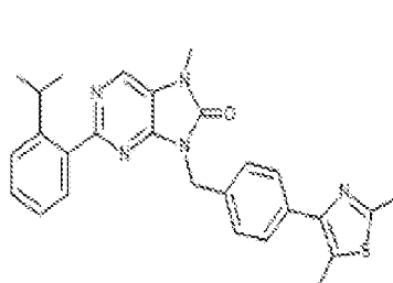
1-304, 9-(4-(2,5-dimethylthiazol-4-yl)benzyl)-2-(2-isopropylphenyl)-7-methyl-7,8-dihydro-8H-purin-6-one
