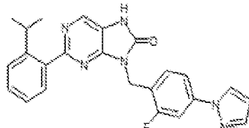
1-167. 8-(2-fluoro-4-(1H-pyrazol-1-yl)benzyl)-2-(2-isopropylphenyl)-7,8-dihydro-8H-purin-6-one
