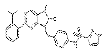
I-456, N-(4-(2-(2-isopropylphenyl)-7-methyl-8-oxo-7,8-dihydro-8H-purin-9-yl)methyl)phenyl)-N,1-dimethyl-1H-pyrazole-3-sulfonamide
