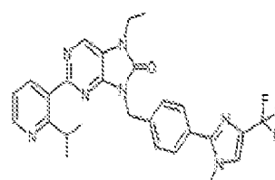
I-507, 7-ethyl-2-(2-isopropylpyridin-3-yl)-8-(4-(1-methyl-4-(trifluoromethyl)-1H-midazol-2-yl)benzyl)-7,8-dihydro-5H-purin-8-one
