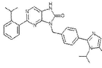
1-536. 9-(4-(1-isopropyl-5-methyl-1H-imidazol-2-yl)benzyl)-2-(2-isopropylphenyl)-7,5-dihydro-8H-purin-8-one
