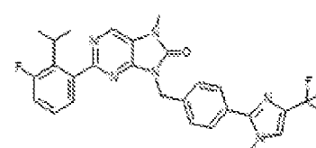
1-65. 2-(3-fluoro-2-isopropylphenyl)-7-methyl-9-(4-(1-methyl-4-(trifluoromethyl)-1H-imidazol-2-yl)benzyl)-7,9-dihydro-8H-purin-8-one
