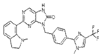
1-34 9-(4-(1-methyl-4-(trifluoromethyl)-1H-imidazol-2-yl)benzyl)-2-(1-methylindolin-7-yl)-7,8-dihydro-8H-purin-8-one
