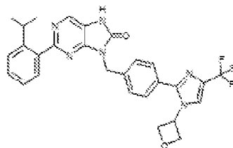
1-192. 2-(2-isopropylphenyl)-9-(4-(1-(oxetan-3-yl)-4-(trifluoromethyl)-1H-imidazol-2-yl)benzyl)-7,8-dihydro-8H-purin-6-one
