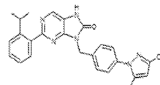
1-210. 9-(4-(3-chloro-5-methyl-1H-pyrazol-1-yl)benzyl)-2-(2-isopropylphenyl)-7,8-dihydro-8H-purin-6-one
