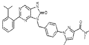
I-503, 1-(4-((2-(2-isopropylphenyl)-8-oxo-7,8-dihydro-5H-purin-3-yl)methyl)phenyl)-N,N,5-trimethyl-1H-pyrazole-3-carboxamide
