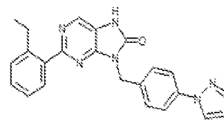
1-27. 8-(4-(1H-pyrazol-1-yl)benzyl)-2-(2-ethylphenyl)-7,9-dihydro-8H-purin-6-one
