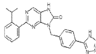
1-513. 8-((4-(1H-tetrazol-5-yl)benzyl)-2-(2-isopropylphenyl)-7,9-dihydro-8H-purin-6-one
