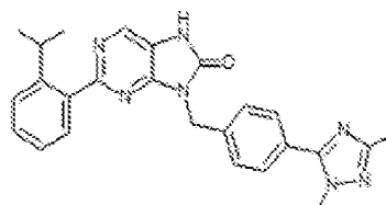
1-296. 9-(4-(1,3-dimethyl-1H-1,2,4-triazol-5-yl)benzyl)-2-(2-isopropylphenyl)-7,8-dihydro-8H-purin-6-one
