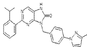
I-204 1-(2-(2-isopropylphenyl)-9-(4-(3-methoxy-1H-pyrazol-1-yl)benzyl)-7,8-dihydro-8H-purin-6-one
