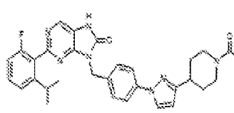
I-474: 9-(4-(3-(1-acetylpiperidin-4-yl)-1H-pyrazol-1-yl)benzyl)-2-(2-fluoro-5-isopropylphenyl)-7,9-dihydro-8H-purin-6-one
