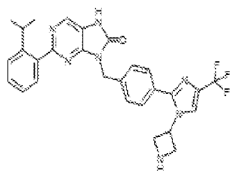
I-430. 9-(4-(1-azetidin-3-yl)-4-(trifluoromethyl)-1H-imidazol-2-yl)benzyl-2-(2-isopropylphenyl)-7,8-dihydro-8H-purin-6-one
