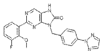
1-16. 9-(4-(2H-1,2,3-triazol-2-yl)benzyl)-2-(3-fluoro-2-methoxyphenyl)-7,8-dihydro-8H-purin-6-one
