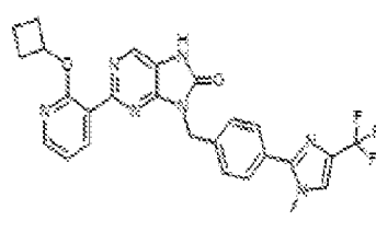
I-419, 2-(2-(oxolanyloxy)pyridin-3-yl)-5-(4-(1-methyl-4-(trifluoromethyl)-1H-imidazol-2-yl)benzyl)-7,8-dihydro-2H-purin-6-one
