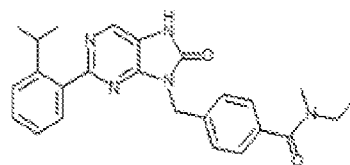
I-373. N-ethyl-4-((2-(2-isopropylphenyl)-8-oxo-7,8-dihydro-9H-purin-5-yl)methyl)-N-methylbenzamide
