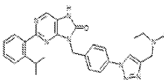
1-346. 5-(4-(4-(diethylamino)methyl)-1H-1,2,3-triazol-1-yl)benzyl)-2-(2-isopropylphenyl)-7,8-dihydro-8H-purin-6-one
