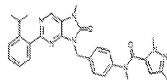
I-471: N-(4-(2-(2-isopropylphenyl)-7-methyl-8-oxo-7,9-dihydro-8H-purin-8-yl)methyl)phenyl)-N,1,3-trimethyl-1H-pyrazole-5-carboxamide
