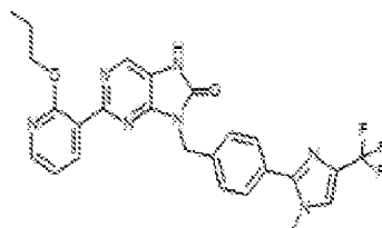
I-413, 5-(4-(1-methyl-4-(trifluoromethyl)-1H-imidazol-2-yl)benzyl)-2-(2-propoxypyridin-3-yl)-7,8-dihydro-2H-purin-6-one
