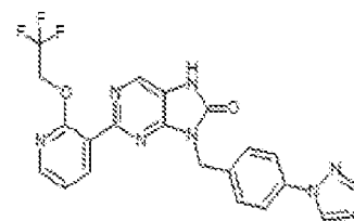
1-18. 9-(4-(1H-pyrazol-1-yl)benzyl)-2-(2,2,2-trifluoroethoxy)pyridin-3-yl)-7,8-dihydro-8H-purin-6-one
