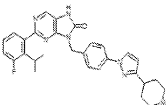
I-434. 2-(3-fluoro-2-isopropylphenyl)-9-(4-(3-piperidin-4-yl)-1H-pyrazol-1-yl)benzyl-7,8-dihydro-8H-purin-6-one
