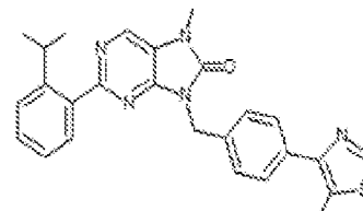
1-303. 9-(4-(2-isopropylphenyl)-7-methyl-5-(4-(5-methylthiazol-4-yl)benzyl)-7,8-dihydro-8H-purin-6-one
