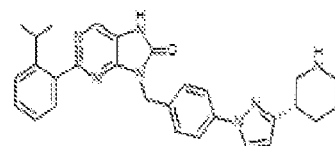
I-225. (S)-2-(2-isopropylphenyl)-9-(4-(3-piperidin-3-yl)-1H-pyrazol-1-yl)benzyl-7,8-dihydro-8H-purin-6-one
