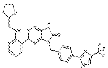
1-320. 9-(4-(1-methyl-4-(trifluoromethyl)-1H-imidazol-2-yl)benzyl)-2-(2-(2-(tetrahydrofuran-2-yl)methylamino)pyridin-3-yl)-7,8-dihydro-8H-purin-6-one
