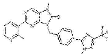
1-62. 7-methyl-9-(4-(1-methyl-4-(trifluoromethyl)-1H-imidazol-2-yl)benzyl)-2-(2-methylpyridin-2-yl)-7,9-dihydro-8H-purin-8-one
