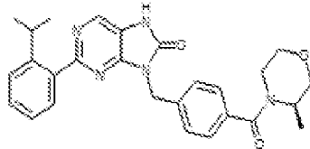
I-404. (R)-2-(2-isopropylphenyl)-6-(4-(3-methylmorpholine-4-carbonyl)benzyl)-7,8-dihydro-8H-purin-6-one
