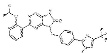
1-35 2-(2-(difluoromethoxy)pyridin-3-yl)-8-(4-(1-methyl-4-(trifluoromethyl)-1H-imidazol-2-yl)benzyl)-7,8-dihydro-8H-purin-8-one
