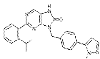
1-256. 2-(2-isopropylphenyl)-9-(4-(1-methyl-1H-pyrazol-5-yl)benzyl)-7,8-dihydro-8H-purin-6-one
