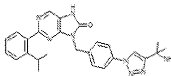
1-338. 9-(4-(4-(2-aminopropan-2-yl)-1H-1,2,3-triazol-1-yl)benzyl)-2-(2-(isopropylphenyl)-7,9-dihydro-8H-purin-6-one
