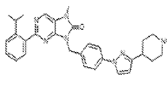
I-433. 2-(2-isopropylphenyl)-7-methyl-9-(4-(3-piperidin-4-yl)-1H-pyrazol-1-yl)benzyl-7,8-dihydro-8H-purin-6-one
