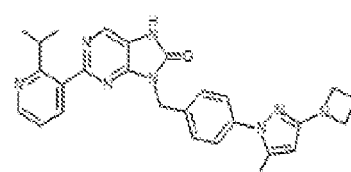
1-68. 9-(4-(3-azetidin-1-yl)-5-methyl-1H-pyrazol-1-yl)benzyl)-2-(2-isopropylpyridin-3-yl)-7,9-dihydro-8H-purin-8-one
