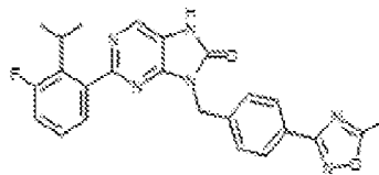
1-188. 2-(3-fluoro-2-isopropylphenyl)-9-(4-(5-methyl-1,2,4-oxadiazol-3-yl)benzyl)-7,8-dihydro-8H-purin-6-one
