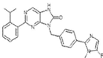
I-176. 9-(4-(5-fluoro-1-methyl-1H-imidazol-2-yl)benzyl)-2-(2-isopropylphenyl)-7,8-dihydro-8H-purin-6-one
