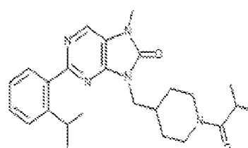
I-462. 5-((1-(2-isopropylpiperidin-4-yl)methyl)-4-(2-isopropylphenyl)-7-methyl-7,8-dihydro-5H-purin-8-one
