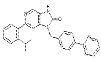
1-255. 2-(2-isopropylphenyl)-9-(4-pyrimidin-2-yl)benzyl)-7,8-dihydro-8H-purin-6-one
