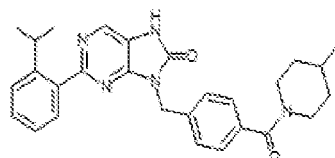
I-366. 2-(2-isopropylphenyl)-5-(4-(4-methylpiperidin-1-yl)carbonylbenzyl)-7,8-dihydro-5H-purin-8-one
