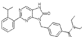
I-362. N,N-diethyl-4-((2-(2-isopropylphenyl)-8-oxo-7,8-dihydro-5H-purin-9-yl)methyl)benzamide
