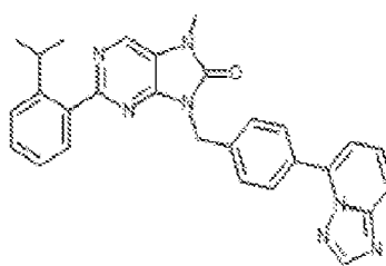
I-266. 9-((4-([1,2,4]triazolo[1,5-a]pyridin-5-yl)benzyl)-2-(2-isopropylphenyl)-7-methyl-7,8-dihydro-8H-purin-6-one
