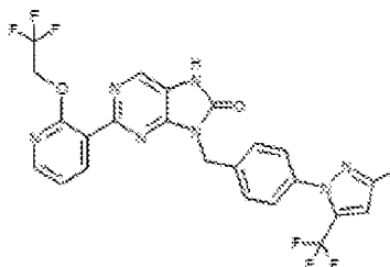
1-41 8-(4-(3-methyl-5-(trifluoromethyl)-1H-pyrazol-1-yl)benzyl)-2-(2,2,2-trifluoroethoxy)pyridin-3-yl)-7,8-dihydro-8H-purin-8-one
