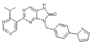
1-28. 8-(4-(1H-pyrazol-1-yl)benzyl)-2-(4-isopropylpyrimidin-5-yl)-7,9-dihydro-8H-purin-6-one
