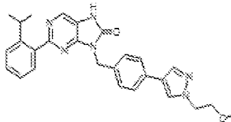
1-518. 2-(2-isopropylphenyl)-8-((1-(2-methoxyethyl)-1H-pyrazol-4-yl)benzyl)-7,9-dihydro-8H-purin-6-one
