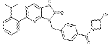
1-377. 5-(4-(3-hydroxyazetidine-1-carbonyl)benzyl)-2-(2-isopropylphenyl)-7,8-dihydro-8H-purin-6-one
