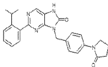
1-512. 2-(2-isopropylphenyl)-8-((2-oxopyrrolidin-1-yl)benzyl)-7,9-dihydro-8H-purin-6-one
