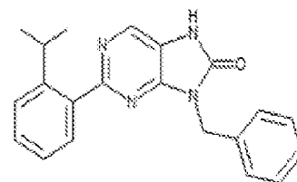
I-171. 5-benzyl-2-(2-isopropylphenyl)-7,8-dihydro-8H-purin-6-one
