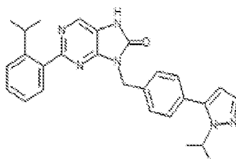
1-299. 9-(4-(1-isopropyl-1H-pyrazol-5-yl)benzyl)-2-(2-isopropylphenyl)-7,8-dihydro-8H-purin-6-one
