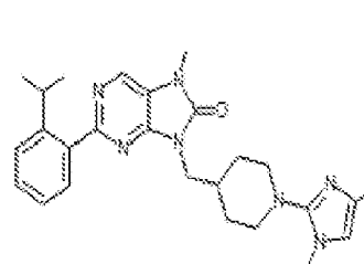
1-501. 9-((1-(1,4-dimethyl-1H-imidazol-2-yl)piperidin-4-yl)methyl)-2-(2-isopropylphenyl)-7-methyl-7,8-dihydro-8H-purin-6-one
