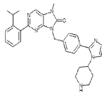
1-499. 2-(2-isopropylphenyl)-7-methyl-9-(4-(1-(piperidin-4-yl)-1H-imidazol-2-yl)benzyl)-7,8-dihydro-8H-purin-6-one
