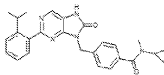
1-379. N-cyclopropyl-4-((2-(2-isopropylphenyl)-8-oxo-7,8-dihydro-8H-purin-9-yl)methyl)-N-methylbenzamide
