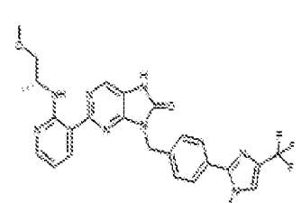
1-319. (R)-2-(2-(1-methoxypropan-2-ylamino)pyridin-3-yl)-9-(4-(1-methyl-4-(trifluoromethyl)-1H-imidazol-2-yl)benzyl)-7,8-dihydro-8H-purin-6-one
