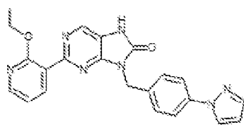
1-19. 9-(4-(1H-pyrazol-1-yl)benzyl)-2-(2-ethoxypyridin-3-yl)-7,8-dihydro-8H-purin-6-one
