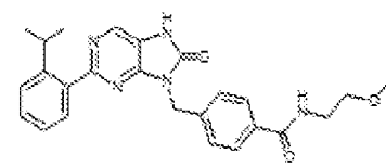
I-352. 4-(2-(2-isopropylphenyl)-8-oxo-7,8-dihydro-5H-purin-9-yl)methyl-N-(2-methoxyethyl)benzamide
