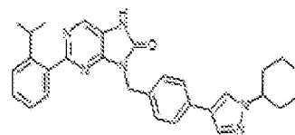
1-519. 2-(2-isopropylphenyl)-8-((4-(1-(tetrahydro-2H-pyran-4-yl)-1H-pyrazol-1-yl)benzyl)-7,9-dihydro-8H-purin-6-one
