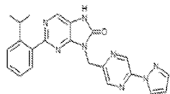
I-508, 9-((5-(1H-pyrazol-1-yl)pyrazin-2-yl)methyl)-2-(2-isopropylphenyl)-7,8-dihydro-5H-purin-8-one
