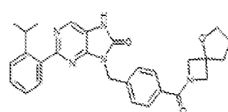
1-393. 3-(4-(5-oxo-2-azaspiro[3.4]octane-2-carbonyl)benzyl)-2-(2-isopropylphenyl)-7,8-dihydro-8H-purin-6-one
