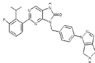
I-103. 8-(4-(5,5-dihydropyrrolo[3,4-c]pyrazol-1(4H)-yl)benzyl)-2-(3-fluoro-2-isopropylphenyl)-7,9-dihydro-8H-purin-6-one
