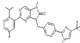
1-69. 2-(5-fluoro-2-isopropylpyridin-3-yl)-7-methyl-9-(4-(1-methyl-4-(trifluoromethyl)-1H-imidazol-2-yl)benzyl)-7,9-dihydro-8H-purin-8-one
