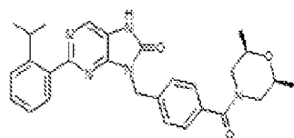
1-385. 3-(4-((2R,5S)-2,5-dimethylmorpholine-4-carbonyl)benzyl)-2-(2-isopropylphenyl)-7,8-dihydro-8H-purin-6-one
