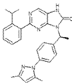
1-191. (S)-9-(1-(4-(3,5-dimethyl-1H-pyrazol-1-yl)phenylethyl)-2-(2-isopropylphenyl)-7,8-dihydro-8H-purin-6-one
