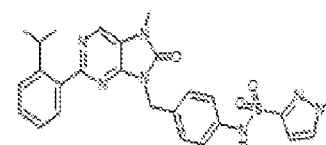
I-453, N-(4-(2-(2-isopropylphenyl)-7-methyl-8-oxo-7,8-dihydro-8H-purin-9-yl)methyl)phenyl)-1-methyl-1H-pyrazole-3-sulfonamide
