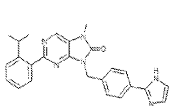
1-529. 5-(4-(1H-imidazol-2-yl)benzyl)-2-(2-isopropylphenyl)-7-methyl-7,5-dihydro-8H-purin-8-one
