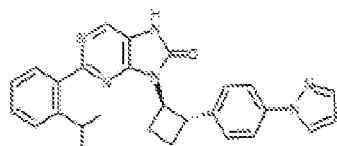
1-163. 9-((1R,2R)-2-(4-(1H-pyrazol-1-yl)phenyl)cyclobutyl)-2-(2-isopropylphenyl)-7,8-dihydro-8H-purin-6-one
