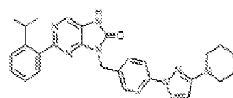
I-174. 2-(2-isopropylphenyl)-9-(4-(3-morpholino-1H-pyrazol-1-yl)benzyl)-7,8-dihydro-8H-purin-6-one
