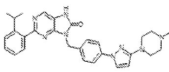
I-173. 2-(2-isopropylphenyl)-9-(4-(3-(4-methylpiperidin-1-yl)-1H-pyrazol-1-yl)benzyl)-7,8-dihydro-8H-purin-6-one
