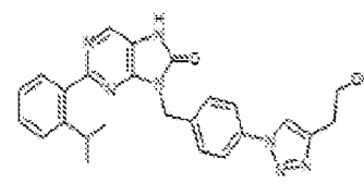
1-342. 5-(4-(4-(2-hydroxyethyl)-1H-1,2,3-triazol-1-yl)benzyl)-2-(2-isopropylphenyl)-7,8-dihydro-8H-purin-6-one
