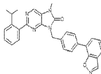
I-267. 9-((4-benzofuran-2-yl)benzyl)-2-(2-isopropylphenyl)-7-methyl-7,8-dihydro-8H-purin-6-one
