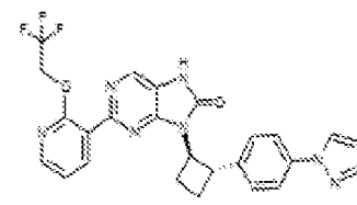
1-24. 9-((1R,2S)-2-(4-(1H-pyrazol-1-yl)phenyl)pyrrolidin-2-yl)-2-(2,2,2-trifluoroethoxy)pyridin-3-yl)-7,8-dihydro-8H-purin-6-one
