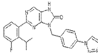
1-165. 9-(4-(1H-1,2,3-triazol-1-yl)benzyl)-2-(3-fluoro-2-isopropylphenyl)-7,8-dihydro-8H-purin-6-one
