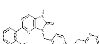
I-231. 2-(2-isopropylphenyl)-7-methyl-9-(4-(pyridin-2-yl)methoxy)benzyl-7,8-dihydro-8H-purin-6-one
