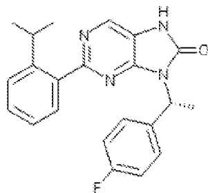
1-178. (R)-3-(1-(4-fluorophenyl)ethyl)-2-(2-isopropylphenyl)-7,8-dihydro-8H-purin-6-one
