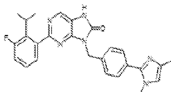
1-307, 9-(4-(1,4-dimethyl-1H-imidazol-2-yl)benzyl)-2-(3-fluoro-2-isopropylphenyl)-7,8-dihydro-8H-purin-6-one
