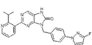
1-59. 9-(4-(3-fluoro-1H-pyrazol-1-yl)benzyl)-2-(2-isopropylpyridin-3-yl)-7,9-dihydro-8H-purin-6-one
