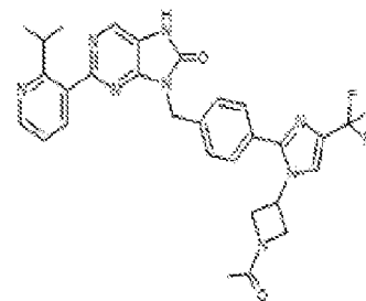
1-477. 9-(4-(1-(1-acetylzetidin-3-yl)-4-(trifluoroethyl)-1H-imidazol-2-yl)benzyl)-2-(2-isopropylphenyl)-7,8-dihydro-8H-purin-6-one
