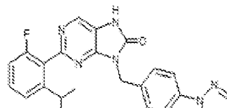
1-96. 9-(4-(1H-pyrazol-1-yl)benzyl)-2-(2-fluoro-3-isopropylphenyl)-7,8-dihydro-8H-purin-6-one
