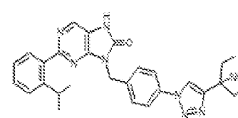
1-348. 5-(4-(4-(3-aminopentan-3-yl)-1H-1,2,3-triazol-1-yl)benzyl)-2-(2-isopropylphenyl)-7,8-dihydro-8H-purin-6-one
