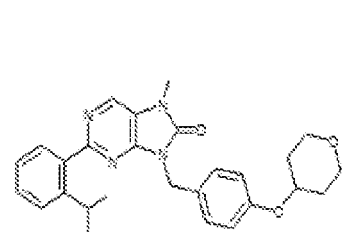
1-238. 2-(2-isopropylphenyl)-7-methyl-9-(4-((tetrahydro-2H-pyran-4-yl)oxy)benzyl)-7,8-dihydro-8H-purin-6-one
