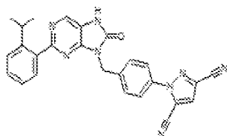
I-199 1-(4-(2-(2-isopropylphenyl)-8-oxo-7,8-dihydro-2H-purin-6-yl)methylphenyl)-1H-pyrazole-3,5-dicarbonitrile
