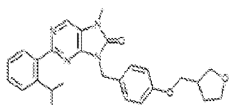
I-229. 2-(2-isopropylphenyl)-7-methyl-9-(4-(1-isotriazofuran-3-yl)methoxy)benzyl-7,8-dihydro-8H-purin-6-one
