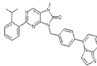
1-270. 9-(4-(imidazo[1,2-a]pyridin-5-yl)benzyl)-2-(2-isopropylphenyl)-7-methyl-7,8-dihydro-8H-purin-6-one
