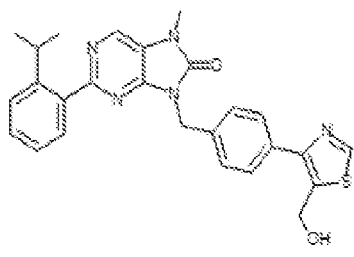
1-305, 9-(4-(5-(hydroxymethyl)thiazol-4-yl)benzyl)-2-(2-isopropylphenyl)-7-methyl-7,8-dihydro-8H-purin-6-one
