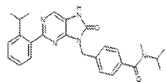
I-375. N-isopropyl-4-((2-(2-isopropylphenyl)-8-oxo-7,8-dihydro-9H-purin-5-yl)methyl)-N-methylbenzamide
