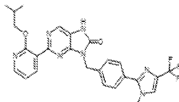
I-422. 2-(2-isobutoxypyridin-3-yl)-9-(4-(1-methyl-4-(trifluoromethyl)-1H-imidazol-2-yl)benzyl)-7,8-dihydro-8H-purin-6-one
