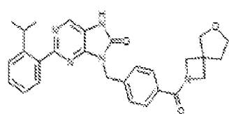
1-394. 8-(4-{8-oxa-2-azaspiro[3.4]octane-2-carbonyl}benzyl)-2-(2-isopropylphenyl)-7,8-dihydro-8H-purin-6-one
