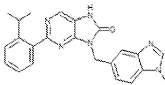
1-182. 2-(2-isopropylphenyl)-5-((1-methyl-1H-benzotriazol-5-yl)methyl)-7,8-dihydro-8H-purin-6-one
