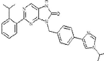
1-275. 9-(4-(1-isopropyl-1H-imidazol-4-yl)benzyl)-2-(2-isopropylphenyl)-7,8-dihydro-8H-purin-6-one
