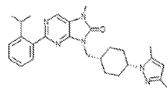
1-111. 5-(((1s,4s)-4-(3,5-dimethyl-1H-pyrazol-1-yl)cyclohexyl)methyl)-2-(2-isopropylphenyl)-7-methyl-7,8-dihydro-8H-purin-6-one
