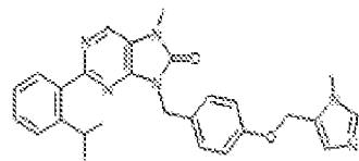
1-232. 2-(2-isopropylphenyl)-7-methyl-9-(4-((1-methyl-1H-imidazol-5-yl)methoxy)benzyl)-7,8-dihydro-8H-purin-6-one
