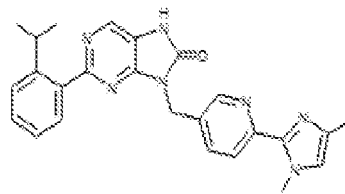
I-203 1-(6-(1,4-dimethyl-1H-imidazol-2-yl)pyridin-3-yl)methyl)-2-(2-isopropylphenyl)-7,8-dihydro-8H-purin-6-one
