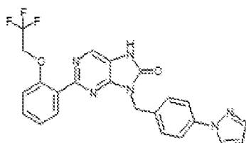
1-22. 9-(4-(1H-pyrazol-1-yl)benzyl)-2-(2-(2,2,2-trifluoroethoxy)phenyl)-7,8-dihydro-8H-purin-6-one
