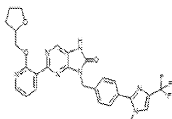
I-424. 9-(4-(1-methyl-4-(trifluoromethyl)-1H-imidazol-2-yl)benzyl)-2-(2-(tetrahydrofuran-2-yl)methoxy)pyridin-3-yl)-7,8-dihydro-8H-purin-6-one
