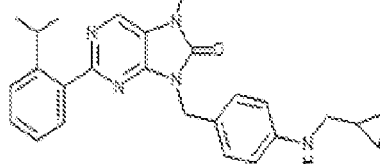
1-488. 9-(4-(cyclopropylmethylamino)benzyl)-2-(2-isopropylphenyl)-7-methyl-7,8-dihydro-6H-purin-6-one
