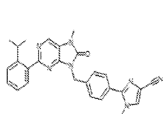
1-541. 2-(4-(2-(2-isopropylphenyl)-7-methyl-8-oxo-7,8-dihydro-5H-purin-3-yl)methyl)phenyl)-1-methyl-1H-imidazole-4-carbonitrile
