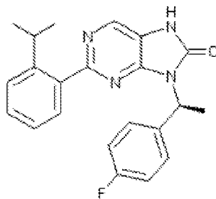
1-179. (S)-3-(1-(4-fluorophenyl)ethyl)-2-(2-isopropylphenyl)-7,8-dihydro-8H-purin-6-one
