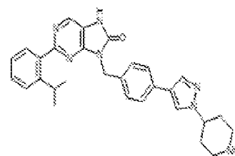
1-540. 2-(2-isopropylphenyl)-9-(4-(1-piperidin-4-yl)-1H-pyrazol-4-yl)benzyl)-7,8-dihydro-5H-purin-8-one
