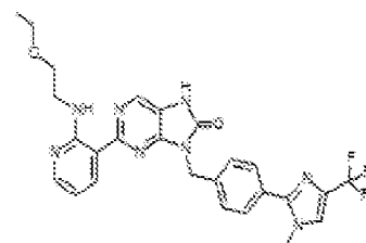
1-315. 2-(2-(2-ethoxyethylamino)pyridin-3-yl)-9-(4-(1-methyl-4-(trifluoromethyl)-1H-imidazol-2-yl)benzyl)-7,8-dihydro-8H-purin-6-one
