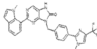
1-45. 2-(1-methyl-1H-indol-7-yl)-9-(4-(1-methyl-4-(trifluoromethyl)-1H-imidazol-2-yl)benzyl)-7,8-dihydro-8H-purin-8-one
