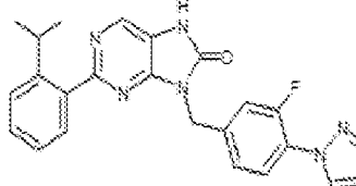
I-177. 9-(3-fluoro-4-(1H-pyrazol-1-yl)benzyl)-2-(2-isopropylphenyl)-7,8-dihydro-8H-purin-6-one
