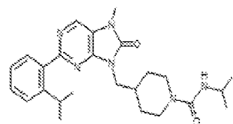
1-478. N-isopropyl-4-(2-(2-isopropylphenyl)-7-methyl-8-oxo-7,8-dihydro-6H-purin-9-yl)methylpiperidine-1-carboxamide
