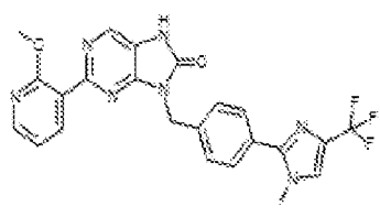
I-412, 2-(2-methoxypyridin-3-yl)-5-(4-(1-methyl-4-(trifluoromethyl)-1H-imidazol-2-yl)benzyl)-7,8-dihydro-2H-purin-6-one
