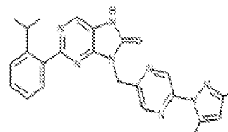
I-510, 9-((5-(3,5-dimethyl-1H-pyrazol-1-yl)pyrazin-2-yl)methyl)-2-(2-isopropylphenyl)-7,8-dihydro-5H-purin-8-one
