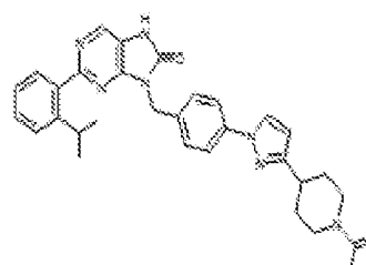
I-463. 5-(4-(3-(1-acetylpiperidin-4-yl)-1H-pyrazol-1-yl)benzyl)-2-(2-isopropylphenyl)-7,8-dihydro-5H-purin-8-one
