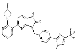
1-334. 2-(2-(3-fluoroazetidin-1-yl)pyridin-3-yl)-8-(4-(1-methyl-4-(trifluoromethyl)-1H-imidazol-2-yl)benzyl)-7,9-dihydro-8H-purin-6-one
