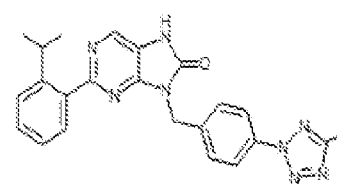
1-168. 2-(2-isopropylphenyl)-8-(4-(5-methyl-2H-tetrazol-2-yl)benzyl)-7,8-dihydro-8H-purin-6-one
