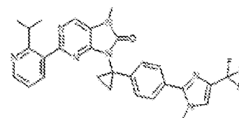
1-108. 2-(2-isopropylpyridin-3-yl)-7-methyl-5-(1-(4-(1-methyl-4-(trifluoromethyl)-1H-imidazol-2-yl)phenyl)cyclopropyl)-7,8-dihydro-8H-purin-6-one
