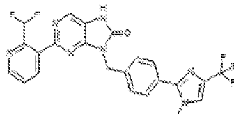
1-64. 2-(2-(difluoromethyl)pyridin-3-yl)-9-(4-(1-methyl-4-(trifluoromethyl)-1H-imidazol-2-yl)benzyl)-7,9-dihydro-8H-purin-8-one
