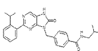
I-357. N-isobutyl-4-(2-(2-isopropylphenyl)-8-oxo-7,8-dihydro-5H-purin-9-yl)methylbenzamide
