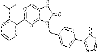
I-437. 9-(4-(1H-imidazol-2-yl)benzyl)-2-(2-isopropylphenyl)-7,8-dihydro-8H-purin-6-one
