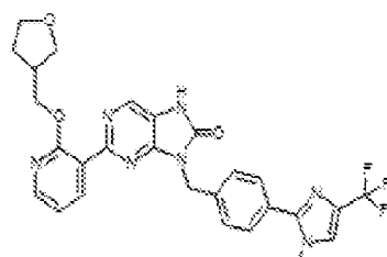
I-425. 9-(4-(1-methyl-4-(trifluoromethyl)-1H-imidazol-2-yl)benzyl)-2-(2-(tetrahydrofuran-3-yl)methoxy)pyridin-3-yl)-7,8-dihydro-8H-purin-6-one
