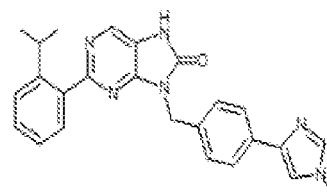
1-273. 2-(2-isopropylphenyl)-9-(4-(1-methyl-1H-imidazol-4-yl)benzyl)-7,8-dihydro-8H-purin-6-one
