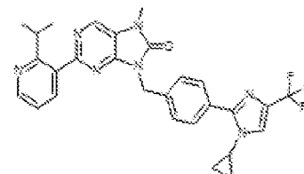
1-114. 9-(4-(1-cyclopropyl-4-(trifluoromethyl)-1H-imidazol-2-yl)benzyl)-2-(2-isopropylpyridin-3-yl)-7-methyl-7,8-dihydro-8H-purin-6-one
