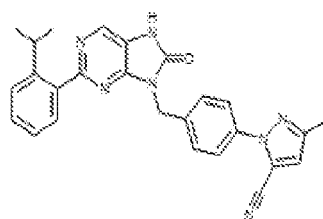
1-288. 1,4-bis(2-isopropylphenyl)-5-oxo-7,8-dihydro-8H-purin-9-ylmethyl(phenyl)-5-methyl-1H-pyrazole-3-carbonitrile
