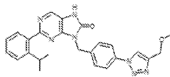
1-344. 2-(2-isopropylphenyl)-5-(4-(4-(methoxymethyl)-1H-1,2,3-triazol-1-yl)benzyl)-7,8-dihydro-8H-purin-6-one
