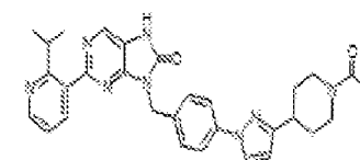
I-465. 5-(4-(3-(1-acetylpiperidin-4-yl)-1H-pyrazol-1-yl)benzyl)-2-(2-isopropylpyridin-3-yl)-7,8-dihydro-5H-purin-8-one
