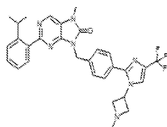
I-448, 2-(2-isopropylphenyl)-7-methyl-8-((1-(1-methylisazefdin-3-yl)-4-(trifluoromethyl)-1H-imidazol-2-yl)methyl)-7,8-dihydro-8H-purin-6-one
