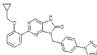
1-23. 9-(4-(1H-pyrazol-1-yl)benzyl)-2-(2-(cyclopropylmethoxy)phenyl)-7,8-dihydro-8H-purin-6-one
