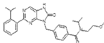
I-370. N-isopropyl-4-((2-(2-isopropylphenyl)-8-oxo-7,8-dihydro-9H-purin-5-yl)methyl)-N-(2-methoxyethyl)benzamide
