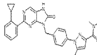
I-504, 1-(4-((2-(2-cyclopropylphenyl)-8-oxo-7,8-dihydro-5H-purin-3-yl)methyl)phenyl)-N,N,5-trimethyl-1H-pyrazole-3-carboxamide
