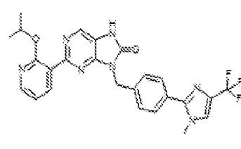
I-416, 2-(2-isopropoxy)pyridin-3-yl)-5-(4-(1-methyl-4-(trifluoromethyl)-1H-imidazol-2-yl)benzyl)-7,8-dihydro-2H-purin-6-one
