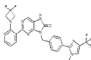
1-336. 2-(2-(3,3-difluoroazetidin-1-yl)pyridin-3-yl)-8-(4-(1-methyl-4-(trifluoromethyl)-1H-imidazol-2-yl)benzyl)-7,9-dihydro-8H-purin-6-one
