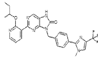
I-417, 2-(2-(sec-butoxy)pyridin-3-yl)-5-(4-(1-methyl-4-(trifluoromethyl)-1H-imidazol-2-yl)benzyl)-7,8-dihydro-2H-purin-6-one
