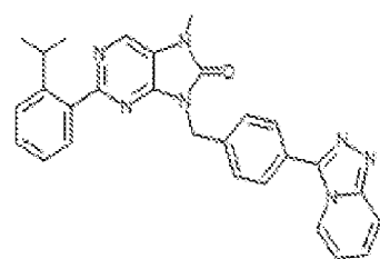
1-286. 5-(4-((1,2,4)imidazo[4,3-a]pyridin-3-yl)benzyl)-2-(2-isopropylphenyl)-7-methyl-7,8-dihydro-8H-purin-6-one
