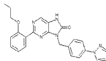
1-21. 9-(4-(1H-pyrazol-1-yl)benzyl)-2-(2-propoxyphenyl)-7,8-dihydro-8H-purin-6-one
