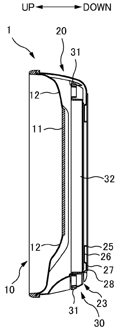
A-A CROSS SECTION FIG. 3B
