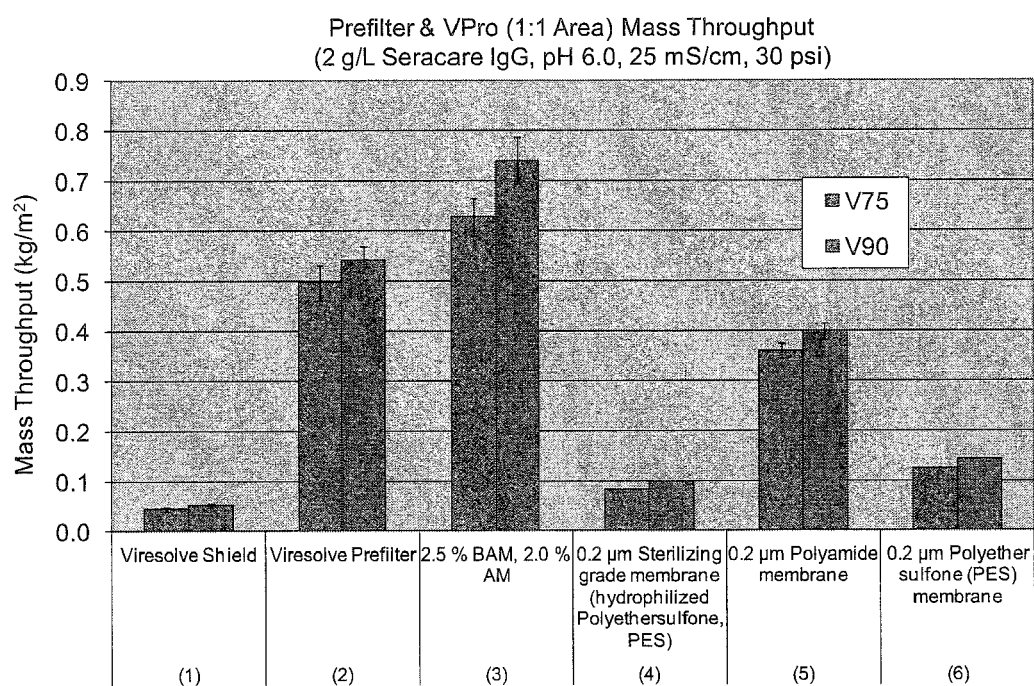
Figure 13. Performance of Acrylamide-containing hydrophobic prefilter in comparison to currently available commercial prefilters and unmodified base membranes at pH 6.0, 25 mS/cm.
