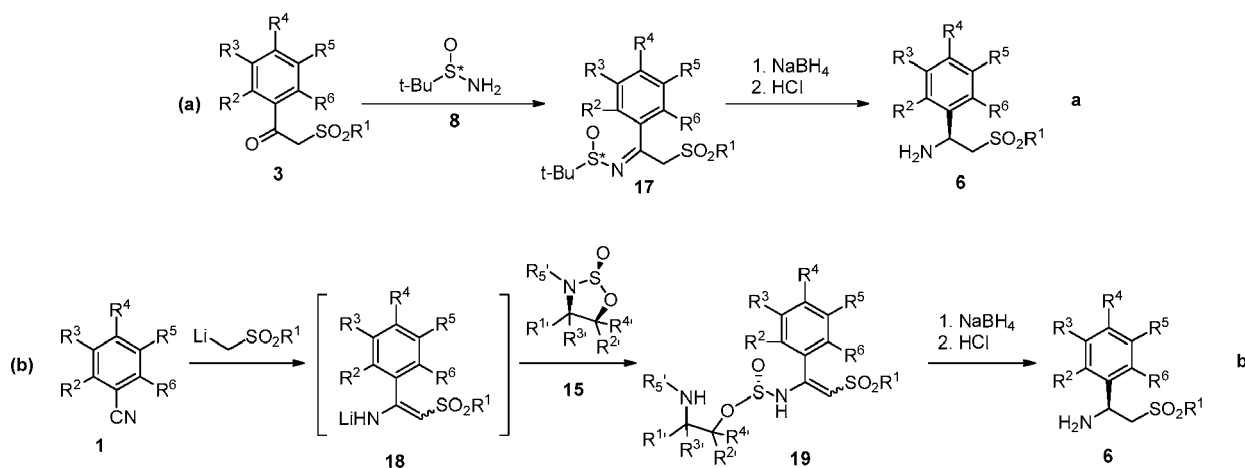
SCHEME 6
