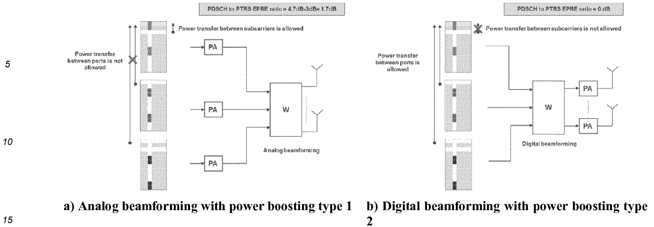
Figure 3. Example of power boosting type 1 and 2 for a transmission with 2 PTRS ports, 3 DMRS ports and 3 PDSCH layers.
