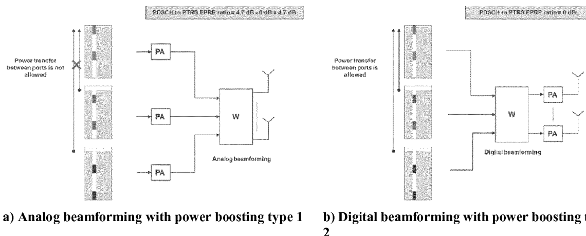
Figure 2. Example of power boosting type 1 and 2 for a transmission with 1 PTRS port, 3 DMRS ports and 3 PDSCH layers.
