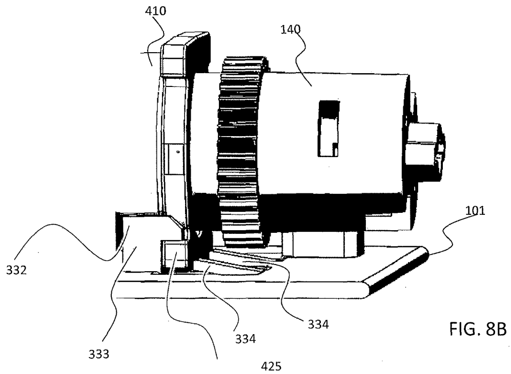
FIGS. 8A-B Exemplary cartridge snap
