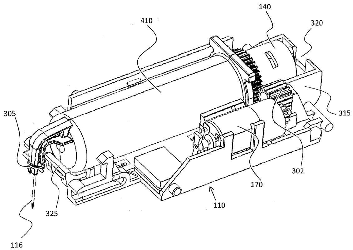
FIG. 3B Exemplary receiving frame components support
