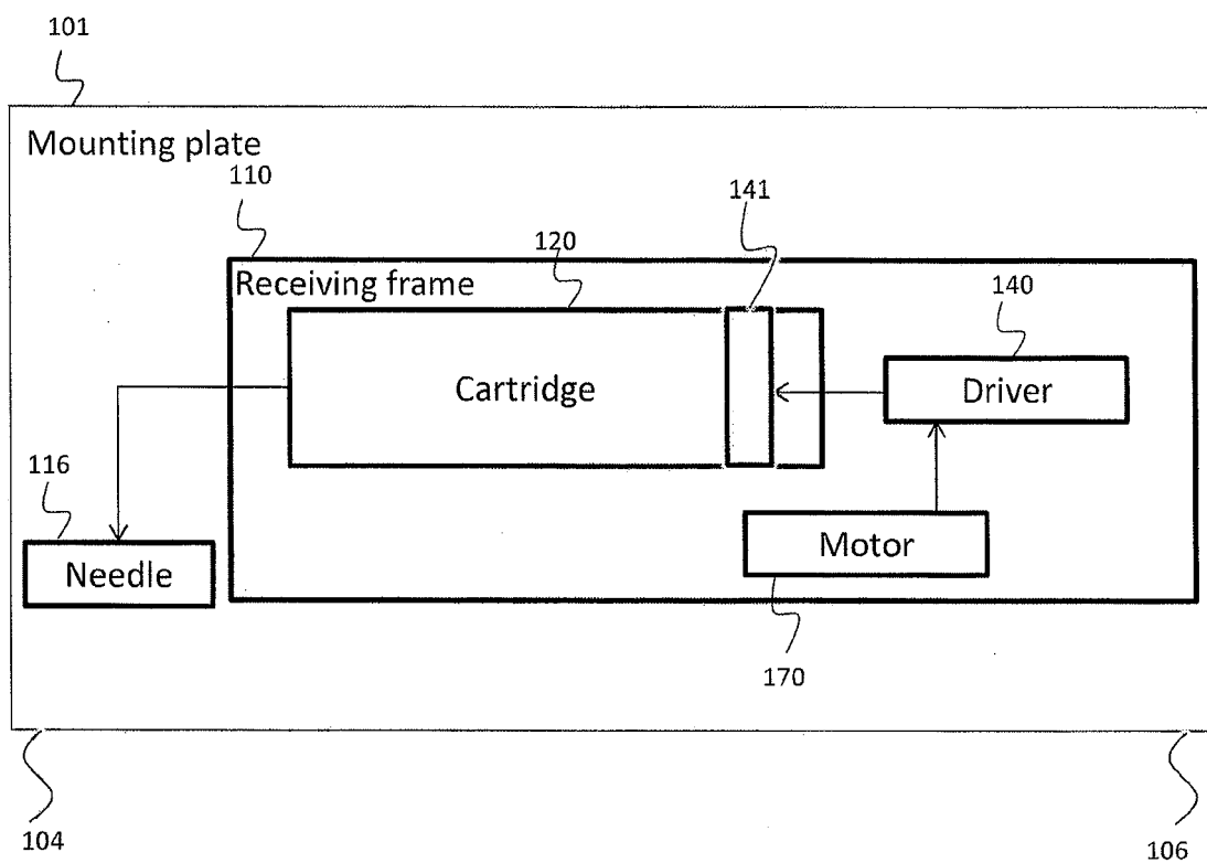
FIG. 1 Block diagram
