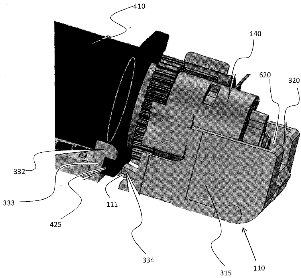
FIG. 6 Exemplary cartridge proximal support
