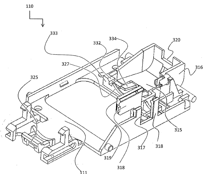
FIG. 3A Receiving frame
