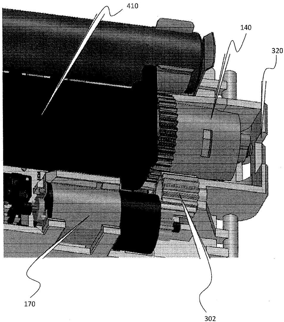
FIG. 7 Exemplary receiving frame components proximal support
