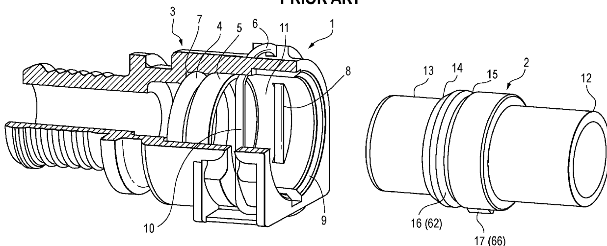
Fig. 1 PRIOR ART
