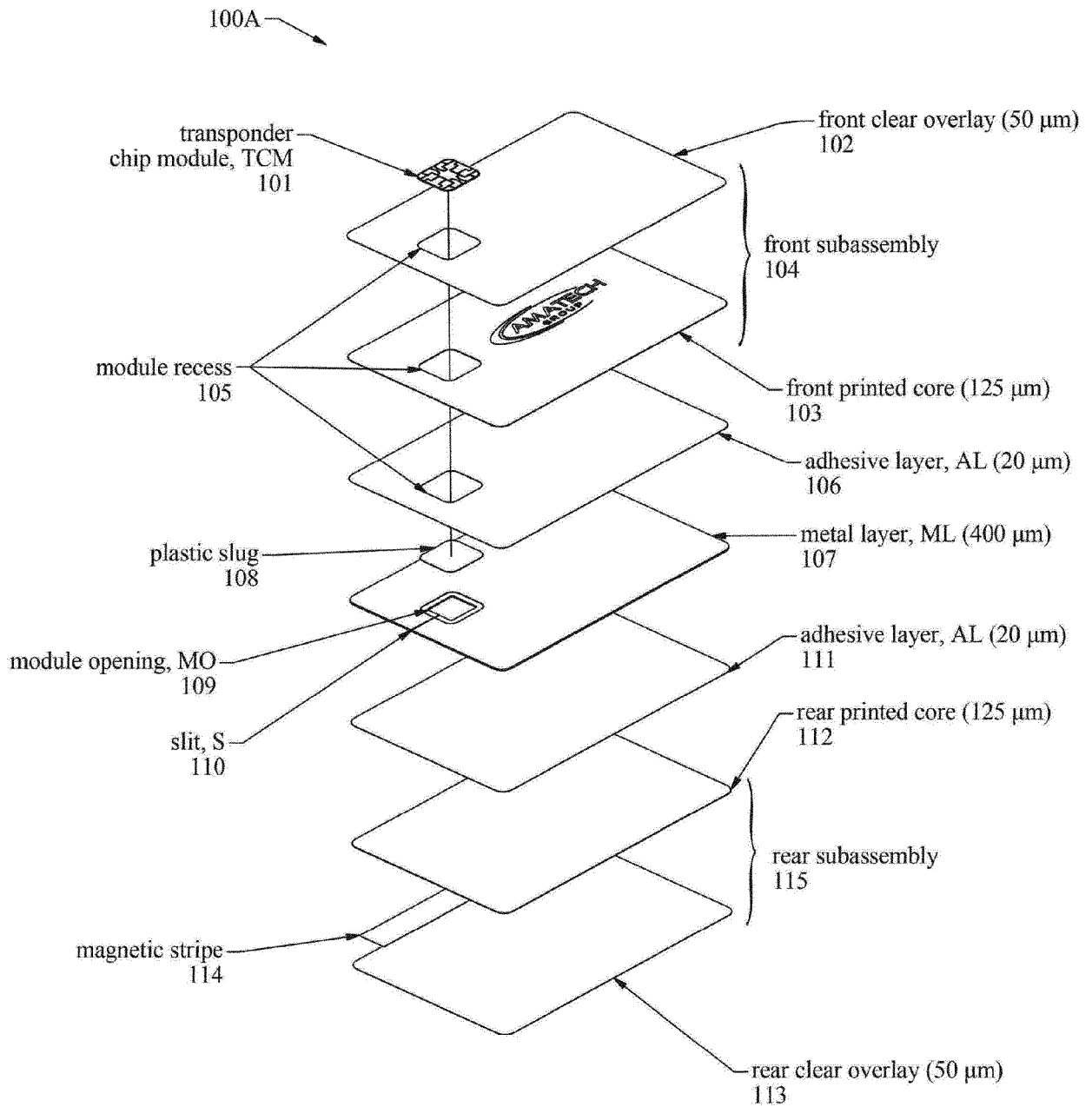
FIG. 1A "Plastic-Metal-Plastic" Hybrid Cards
