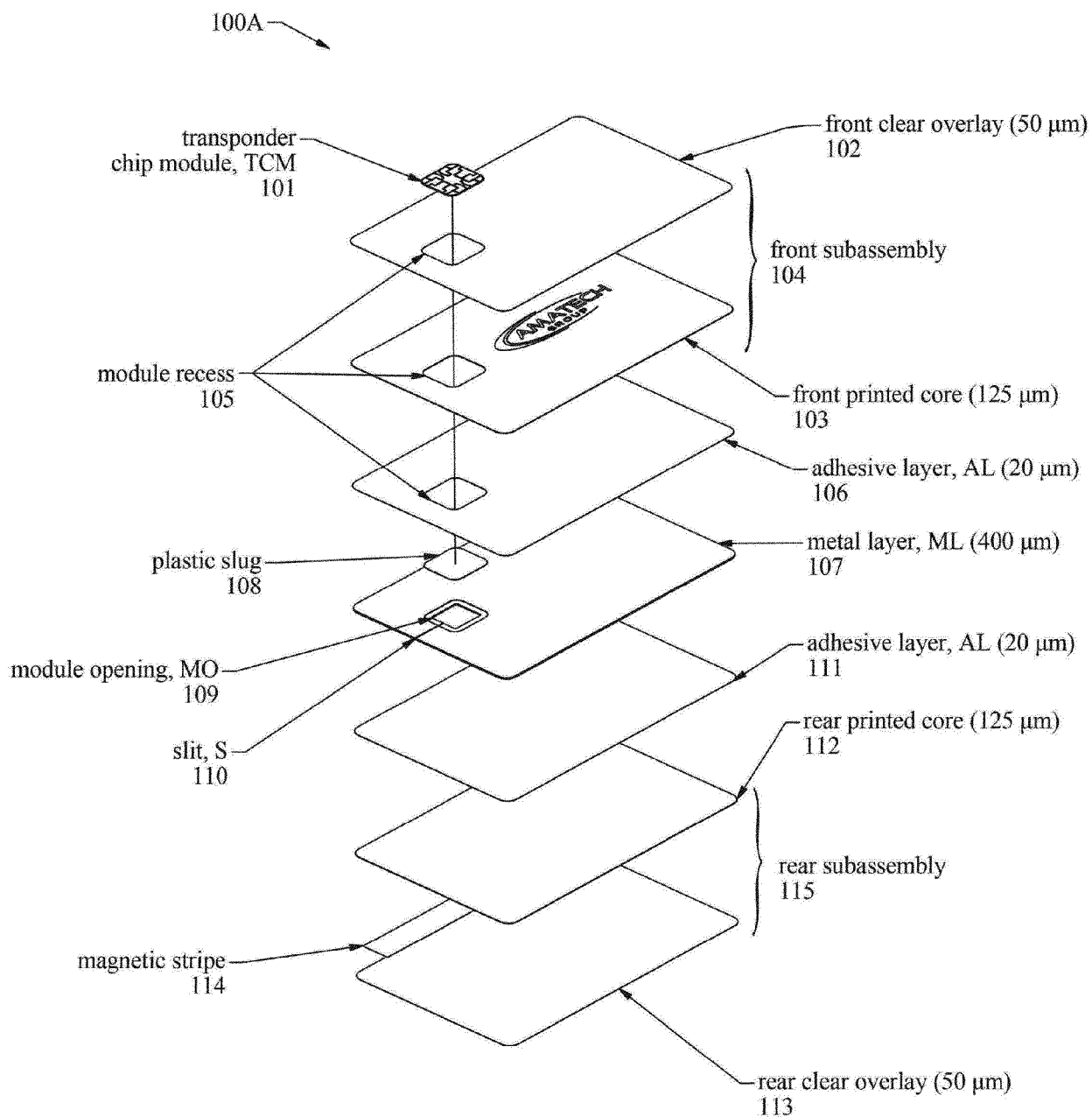
FIG. 1A "Plastic-Metal-Plastic" Hybrid Cards
