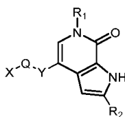
Formula (I)
