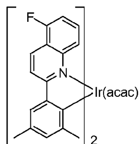
Compound 8
