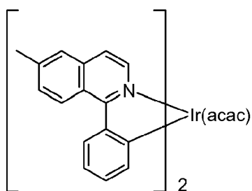
Compound 11
