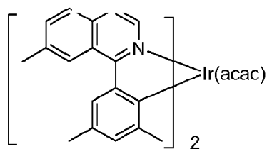
Compound 24
