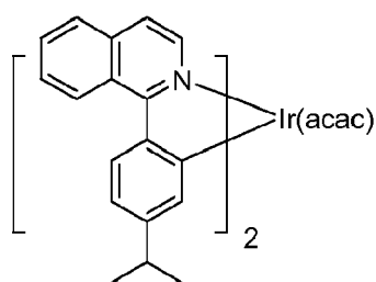
Compound 3
