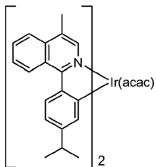
Compound 12
