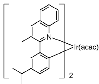
Compound 2
