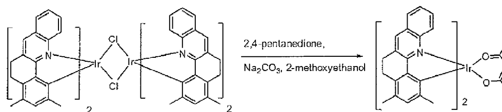
Compound 19
