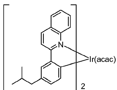
Compound 20
