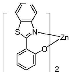
Compound C
