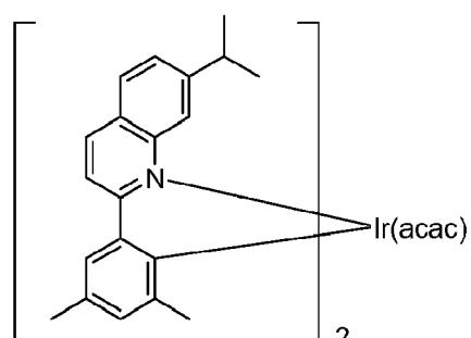
Compound 17
