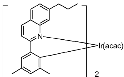
Compound 9
