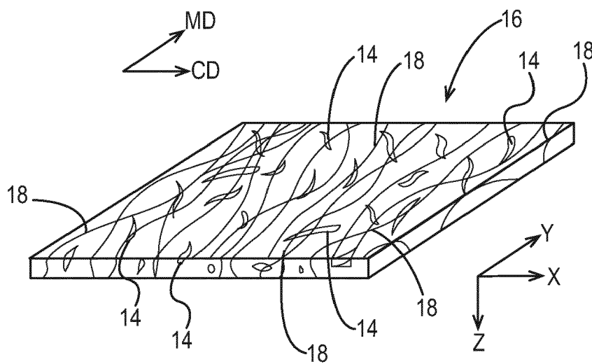
Fig. 2 PRIOR ART
