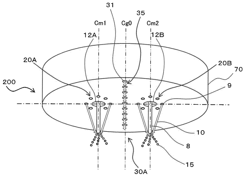
MULTI-HOLE AIR CURTAIN
