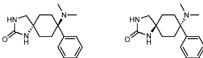
TRANS configuration
