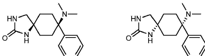
CIS configuration
