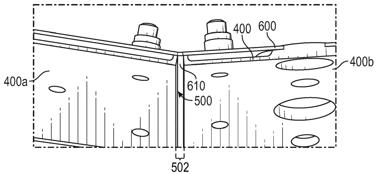
FIG. 3 (Prior Art)
