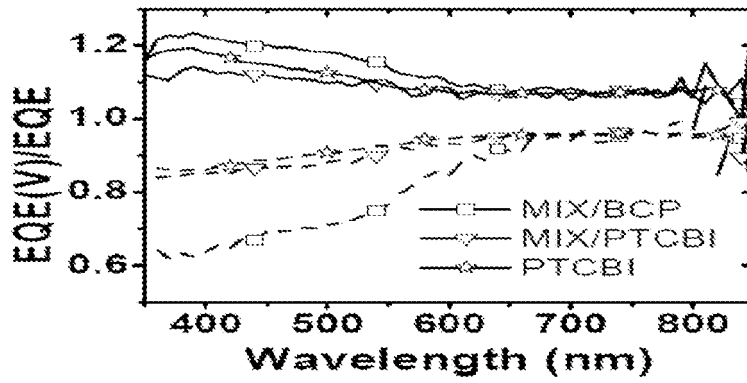
Figure 8: Plot of external quantum efficiency under applied bias ( \sim 0.5 V dashed, \sim 1 V solid) normalized to EQE at zero bias for various buffer layers. These data demonstrate the mixed buffer layer reduces the bias dependence of the device exhibiting a decrease in charge buildup at the active layer/buffer interface, consequently decreasing the amount of exciton-polaron quenching.
