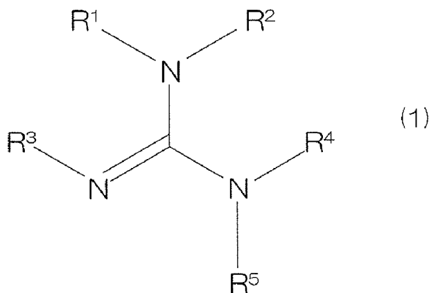
[Chemical Formula 1]
