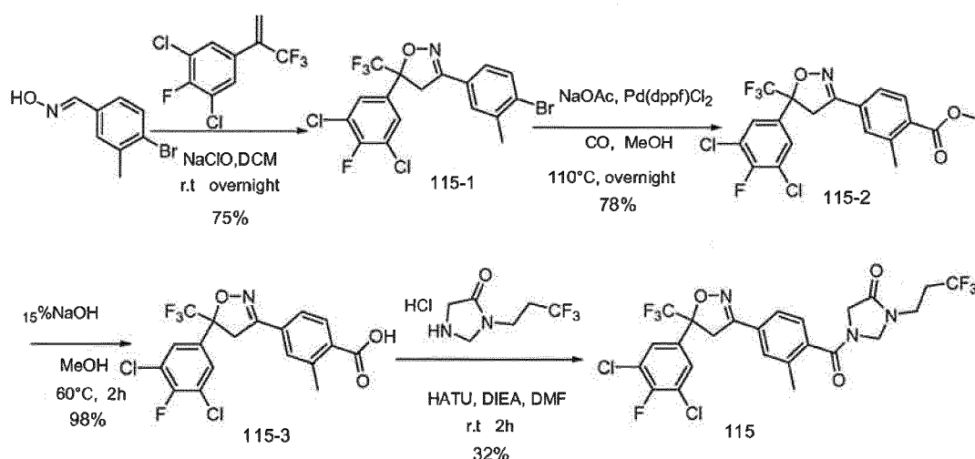
Scheme 16
