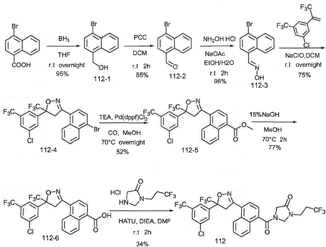
Scheme 14
