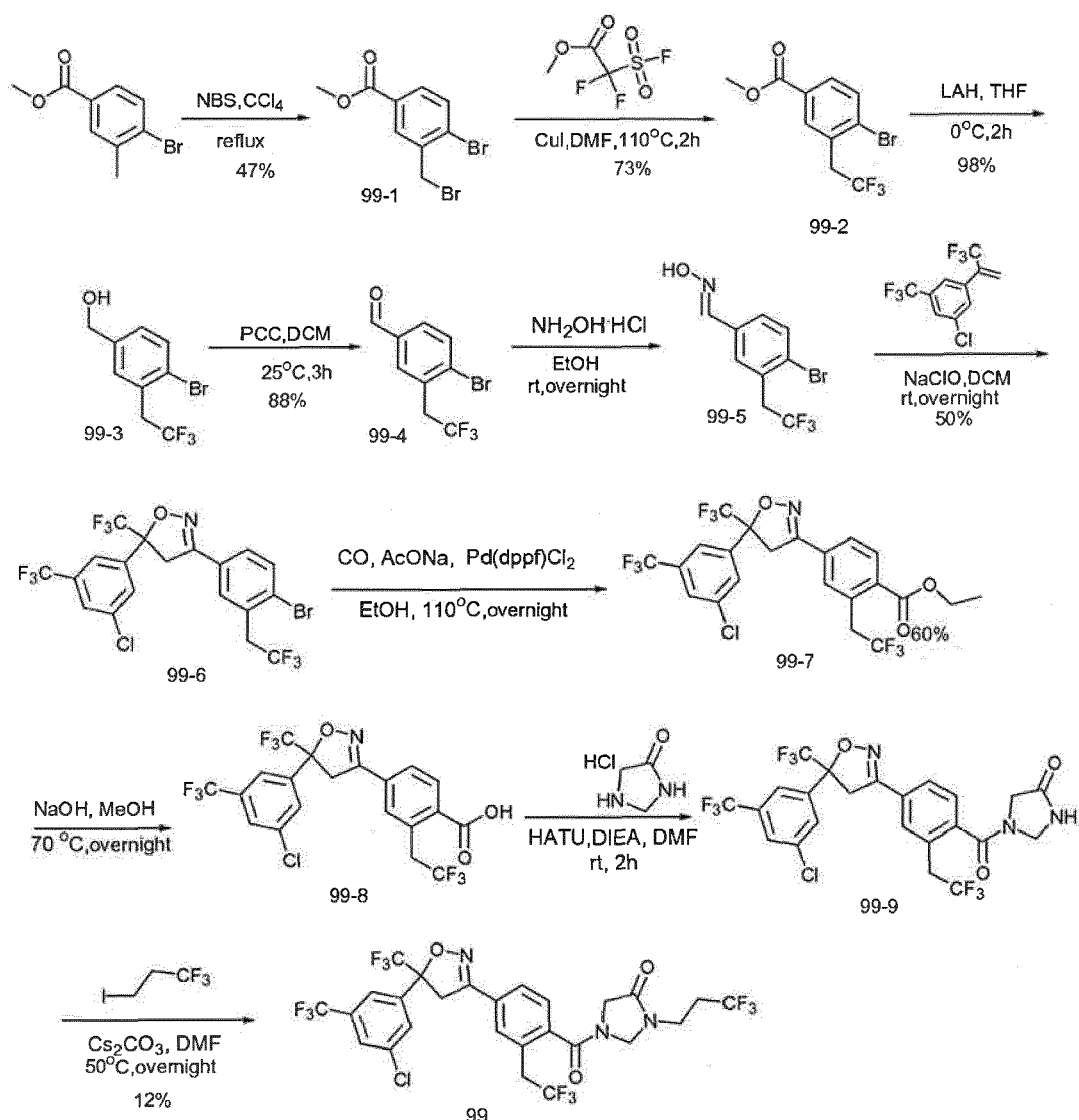
Scheme 13
