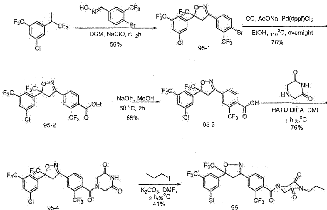
Scheme 10
