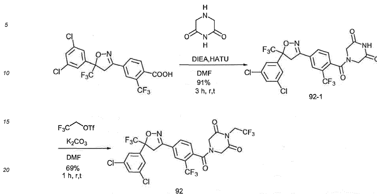
Scheme 8
