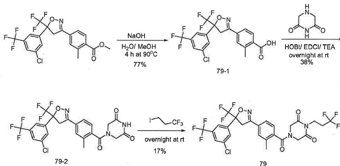
Scheme 6
