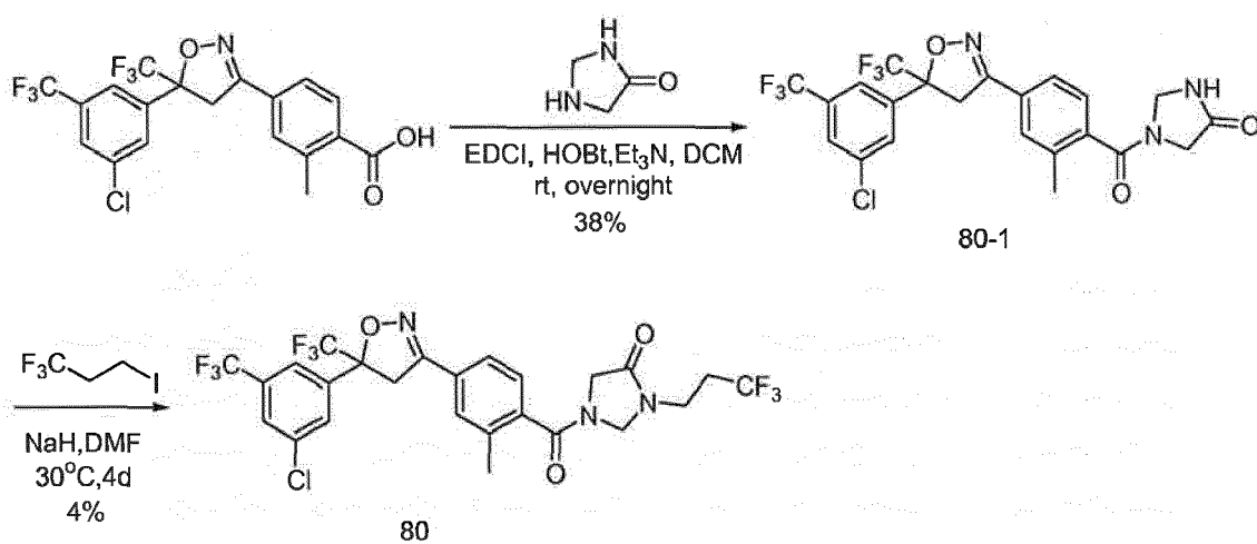
Scheme 7
