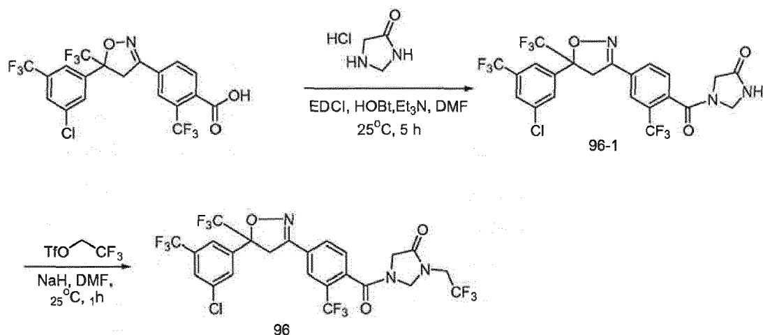
Scheme 11
