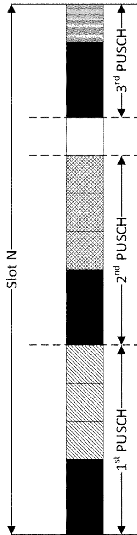
Fig. 12 Incorrect
