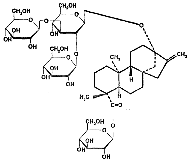
Rebaudioside A
