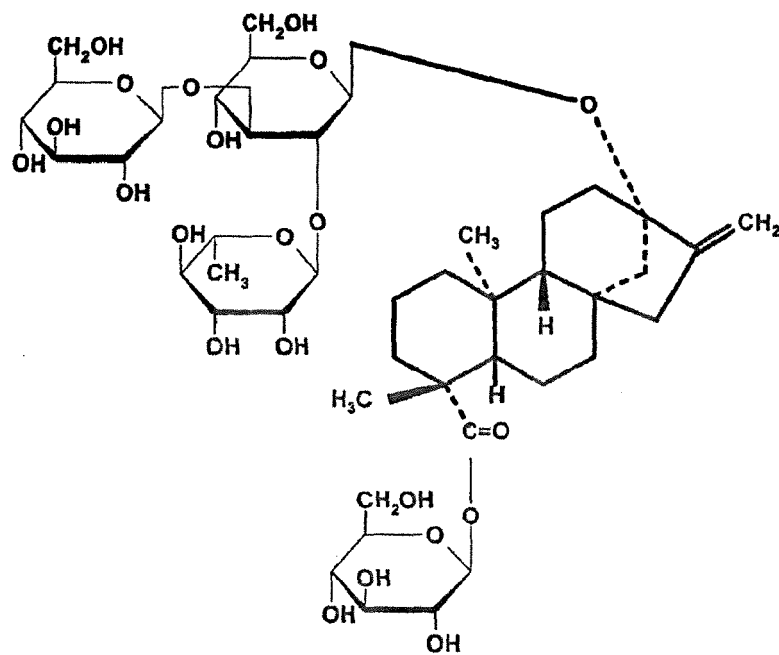
Rebaudioside C
