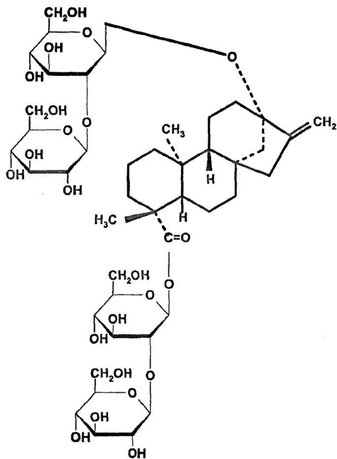
Rebaudioside E
