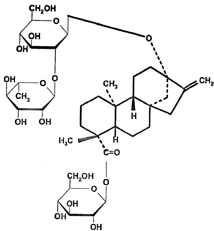
Dulcoside A
