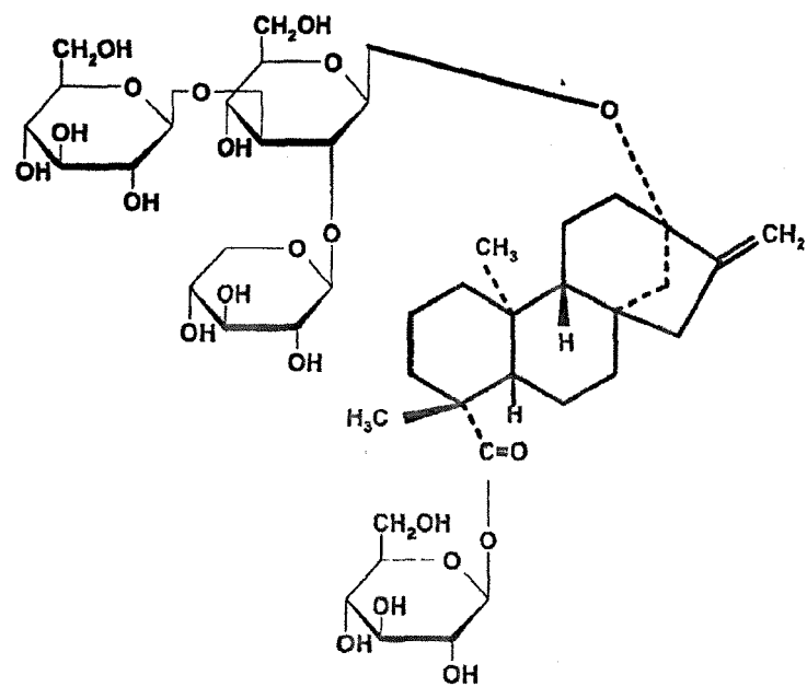
Rebaudioside F
