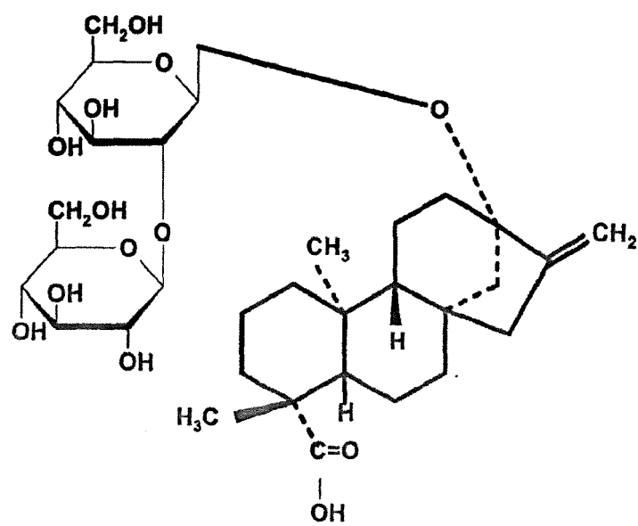
Steviolbioside
